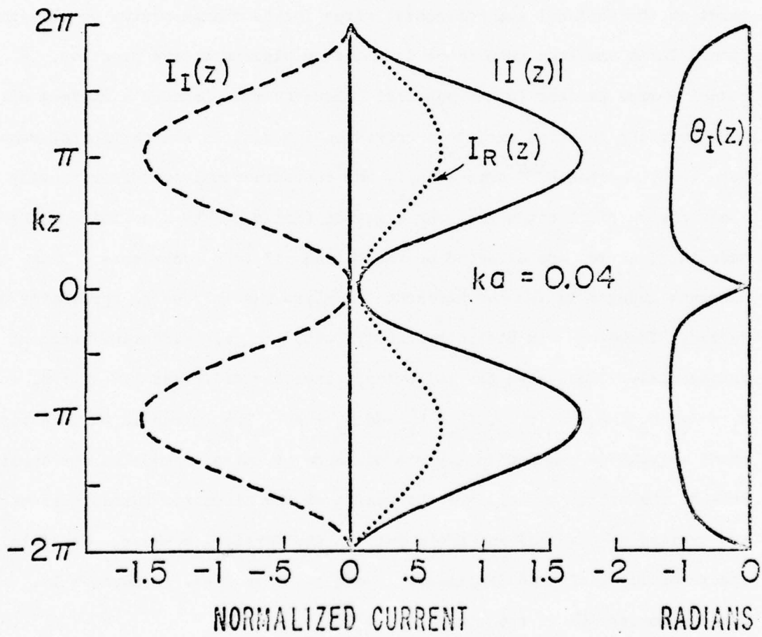
Fig. 14. Current on parasitic antenna (King-Wu theory).
