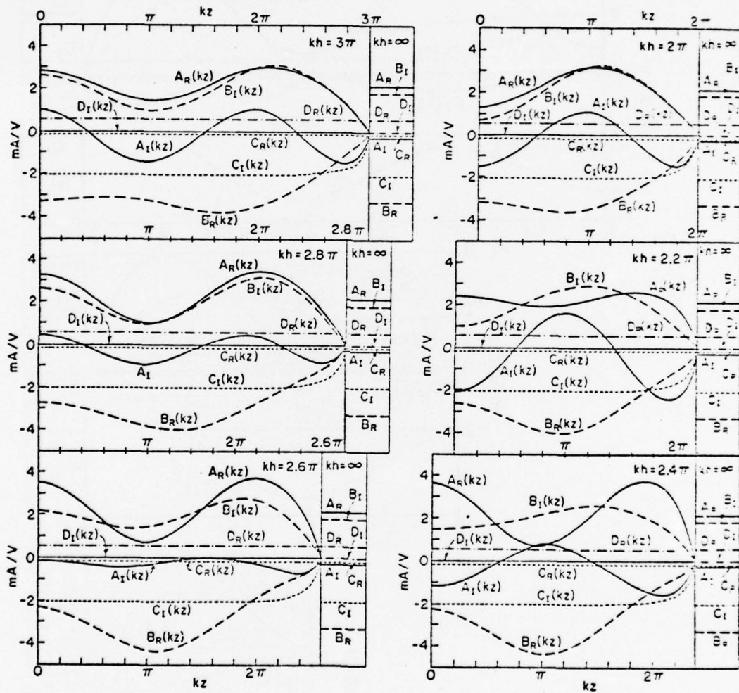
Fig. 43. Fourier coefficients of surface density of axial current on tubular cylinder, K_z(\theta, z) = A(kz) + B(kz)\cos\theta + C(kz)\cos 2\theta + D(kz)\cos 3\theta ; E-polarization, normal incidence; ka = 1 .
