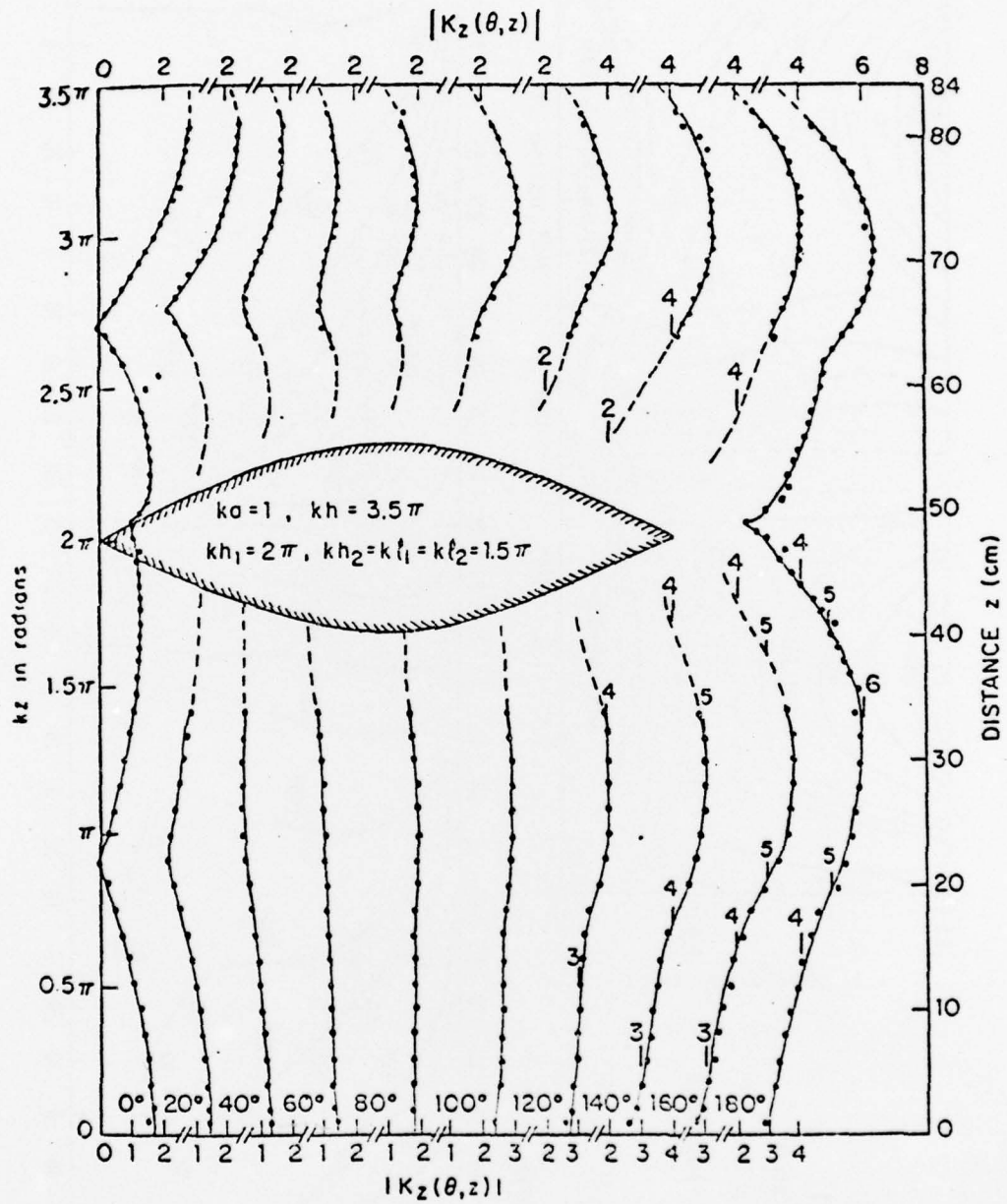
Fig. 54. Measured magnitude of surface density of axial current on vertical member of crossed cylinders; E-polarization, normal incidence.
