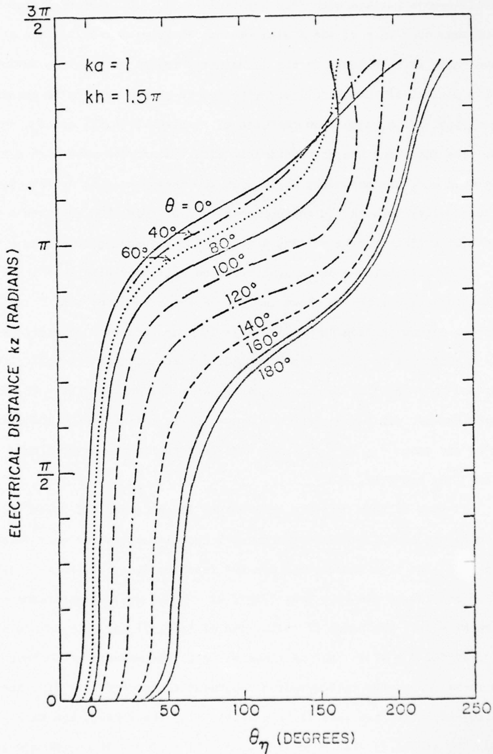
Fig. 26b. Theoretical phase of surface density of charge on tubular cylinder, \eta = |\eta|e^{i\theta_\eta} ; E-polarization, normal incidence.
