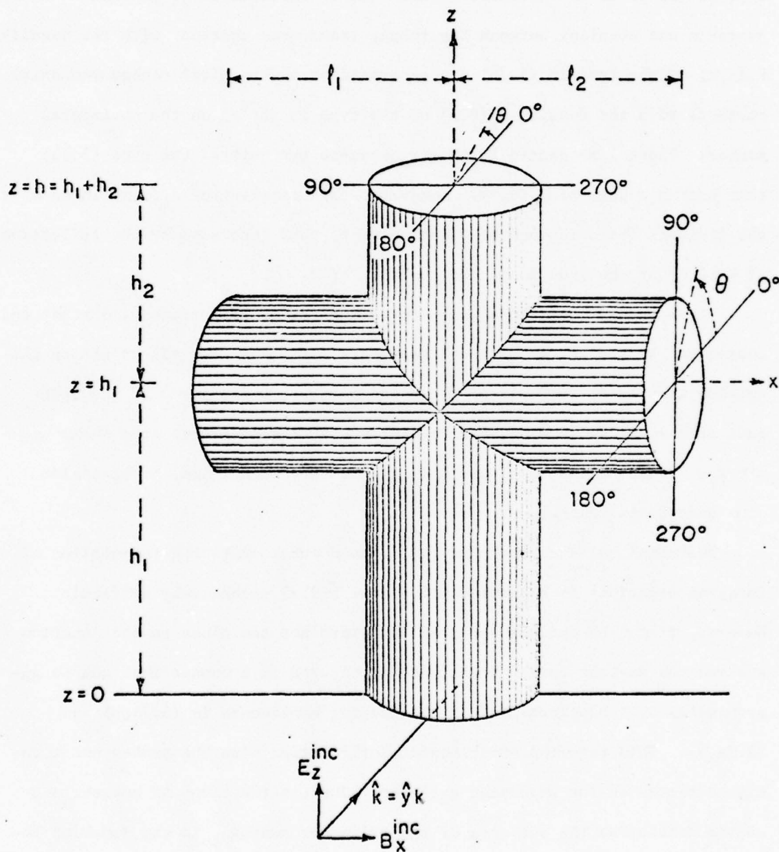
Fig. 47. Diagram of crossed electrically thick cylinders illuminated by normally incident, plane-wave field.
