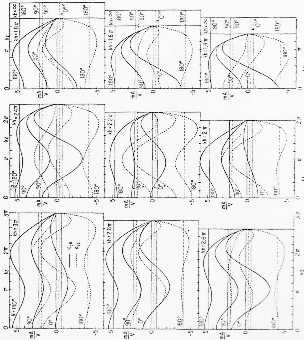
Fig. 28. Surface density of axial current on tubular cylinder, K_z(\theta, z) = K_{zR} + iK_{zI} ; E-polarization, normal incidence; ka = 1 .
