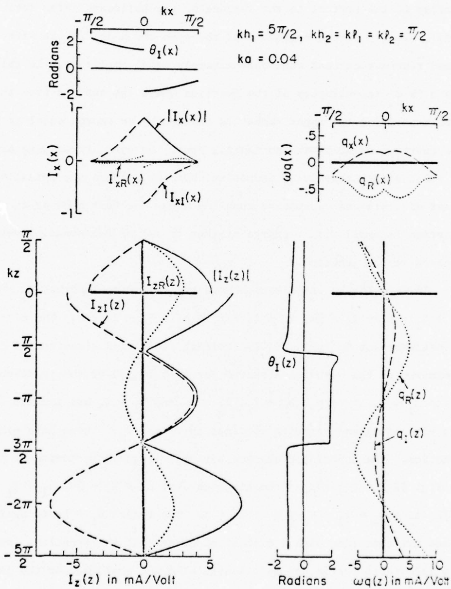
Fig. 15. Theoretical distributions of current and charge per unit length on crossed antenna in normally incident, plane-wave field; kh_1 = 5\pi/2, kh_2 = kp_1 = kp_2 = \pi/2 .
