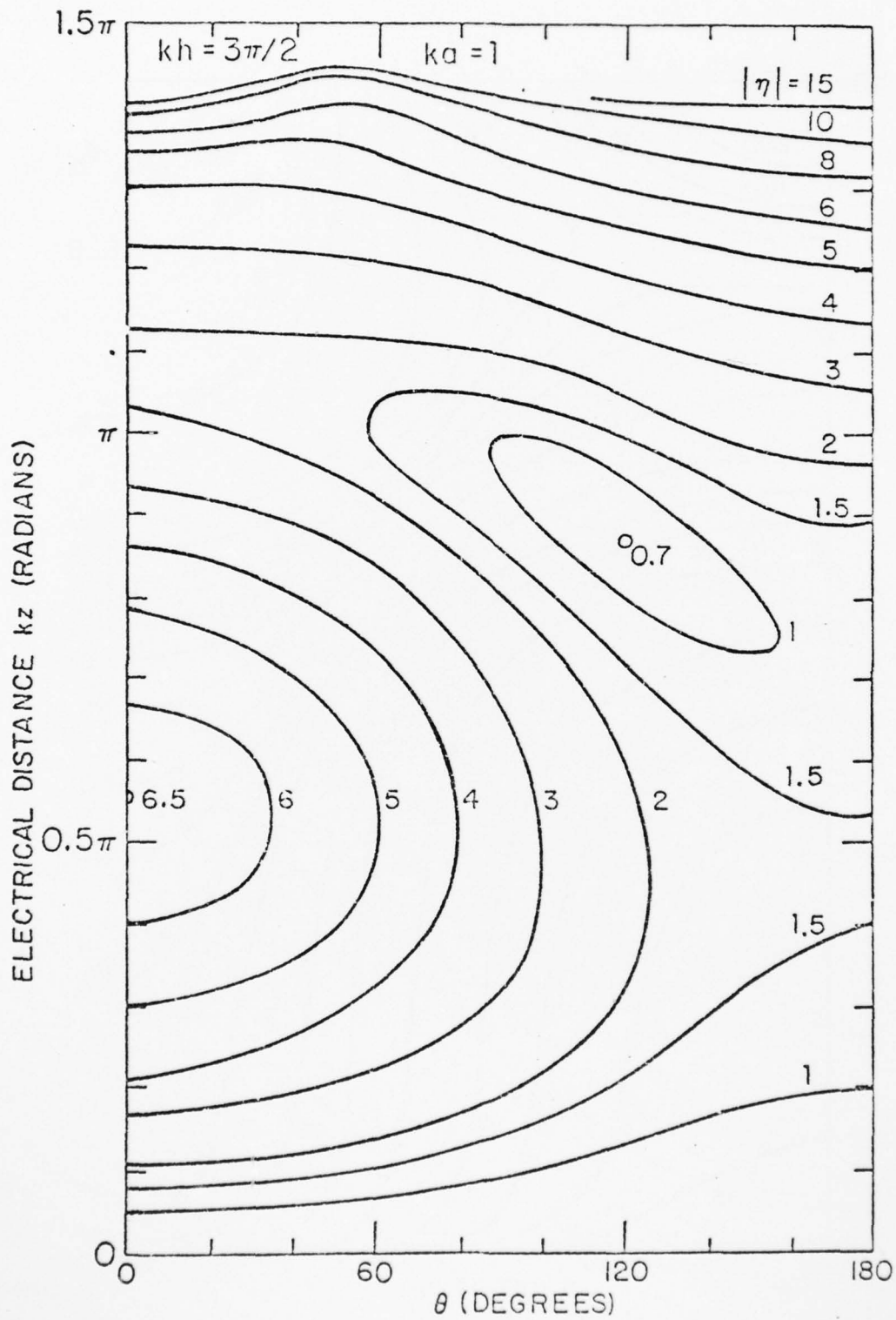
Fig. 27a. Theoretical contours of magnitude of surface density of charge on tubular cylinder; E-polarization, normal incidence.
