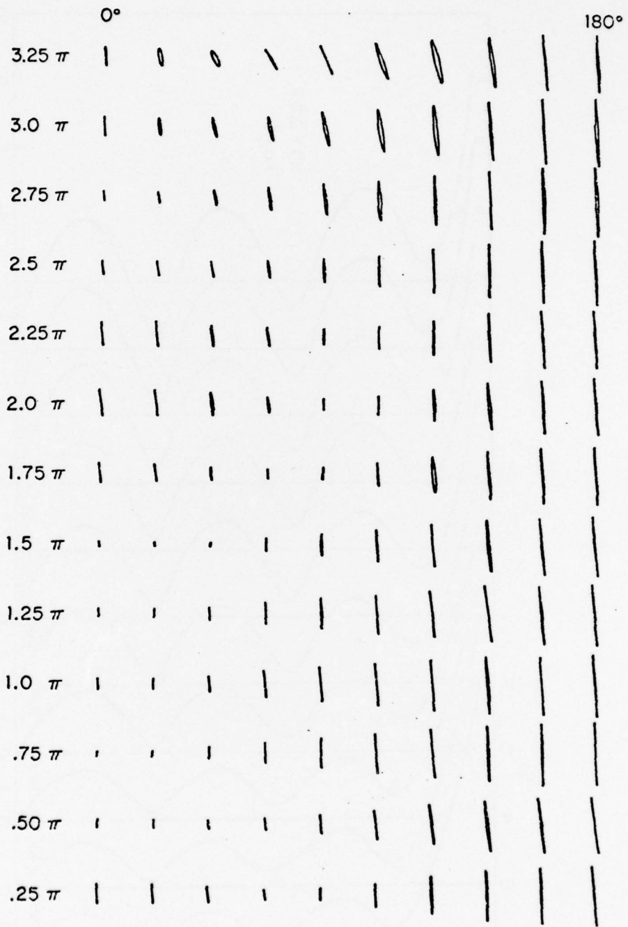
Fig. 37. Measured polarization ellipses of \vec{K}(\theta, z) on tubular cylinder; E-polarization, normal incidence; kh = 3.5\pi , ka = 1 .
