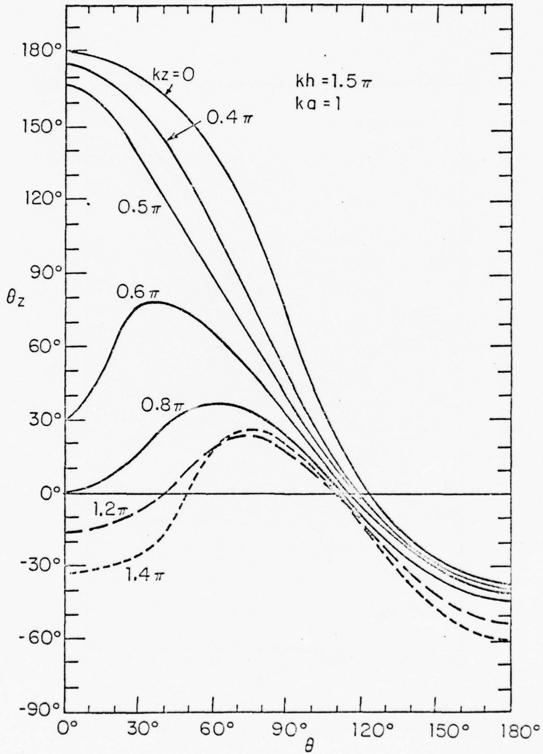
Fig. 22b. Theoretical phase of surface density of total axial current on tubular cylinder; E-polarization, normal incidence.
