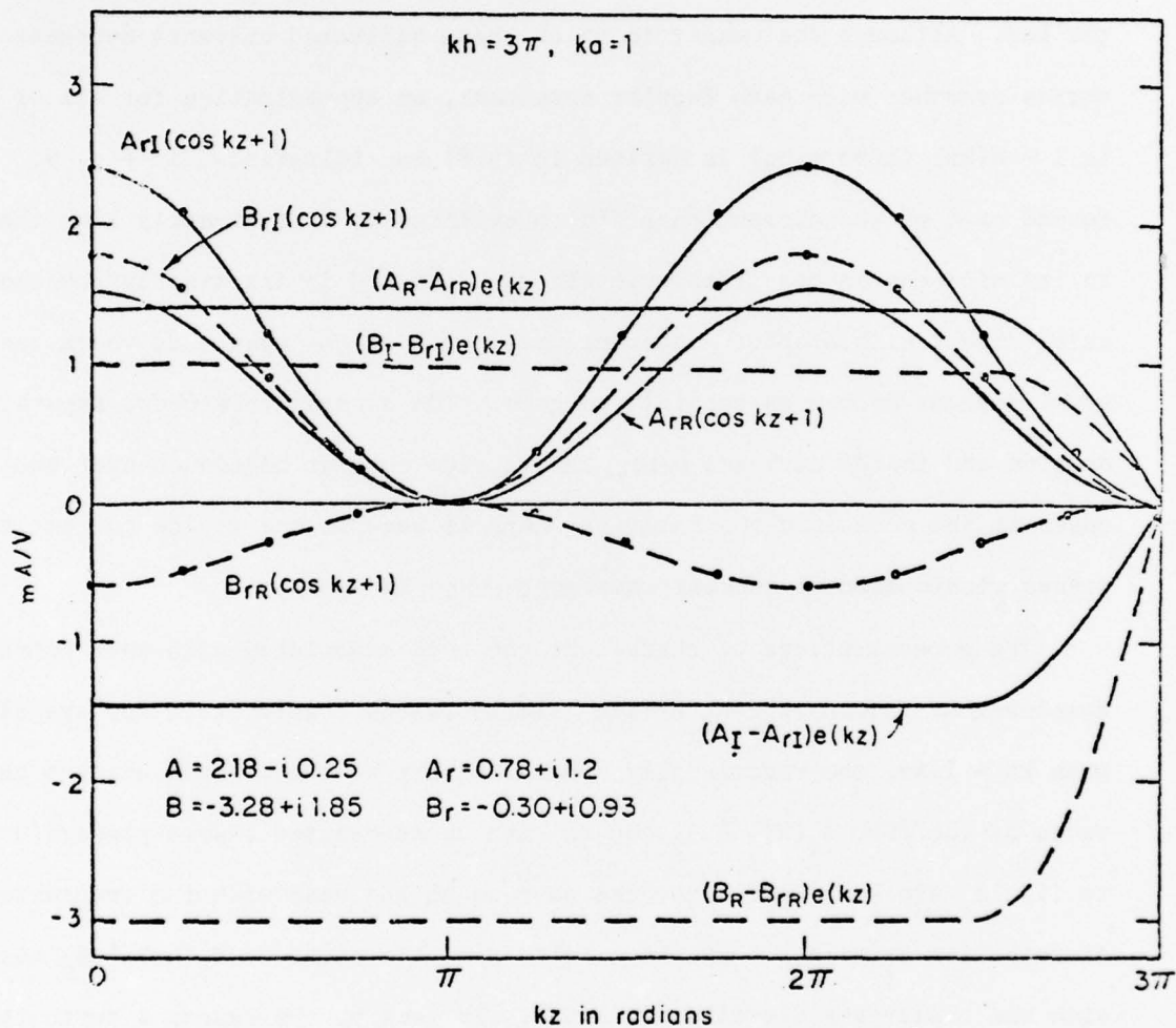
Fig. 46. Components in the approximate representation shown on right in Fig. 45: A(kz) = (A - A_R)e(kz) + A_I(\cos kz + 1) , B(kz) = (B - B_I)e(kz) + B_I(\cos kz + 1) .
