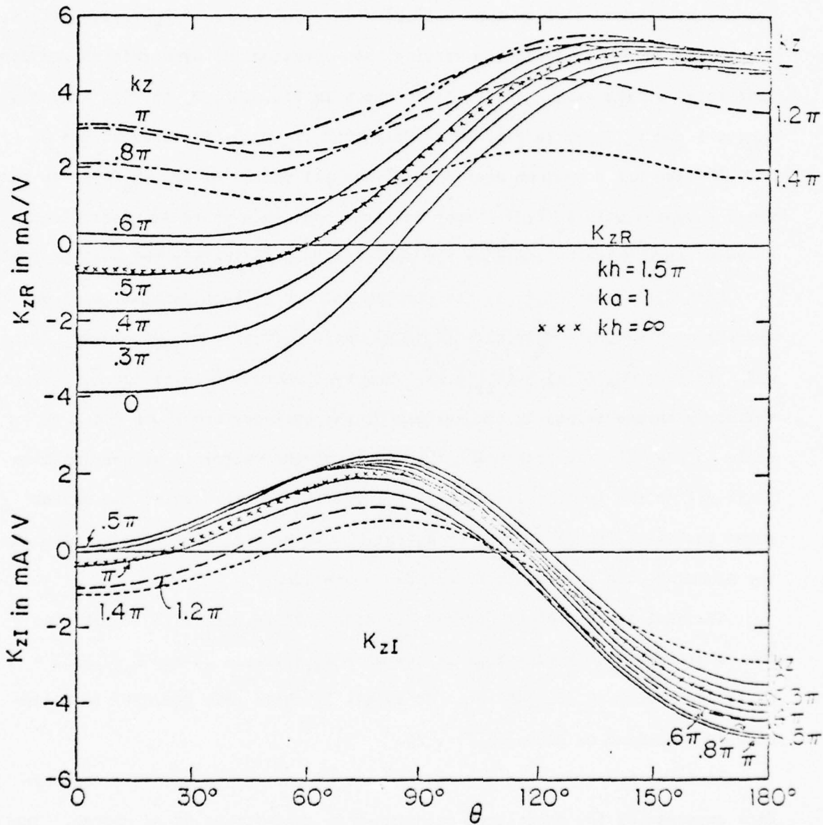
Fig. 22c. Real and imaginary parts of K_z(\theta, z) on tubular cylinder; E-polarization, normal incidence. K_z(0) with kh = \infty .
