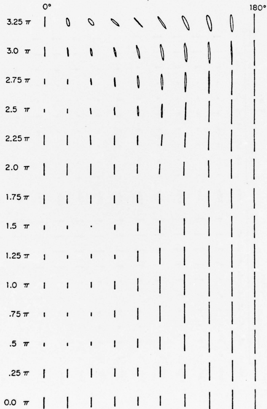
Fig. 36. Theoretical polarization ellipses of \vec{K}(\theta, z) on tubular cylinder; E-polarization, normal incidence; kh = 3.5\pi , ka = 1 .
