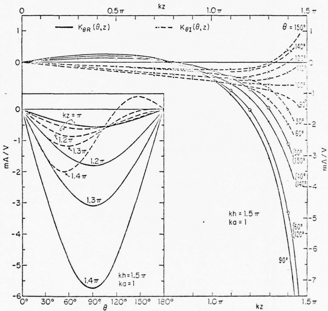
Fig. 23c. Real and imaginary parts of K_\theta(\theta, z) on tubular cylinder; E-polarization, normal incidence.
