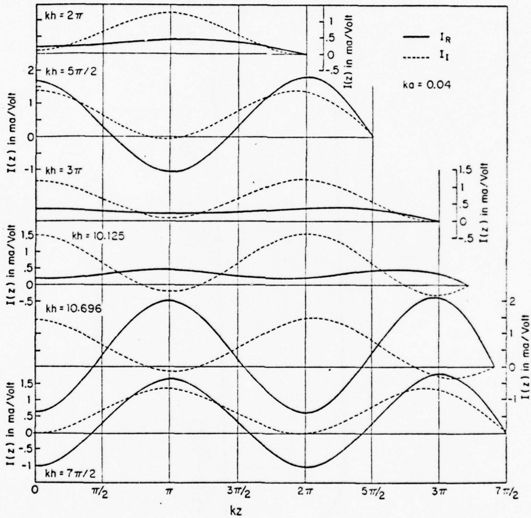
Fig. 8. Real and imaginary currents on parasitic antenna in normally incident, plane-wave field.
