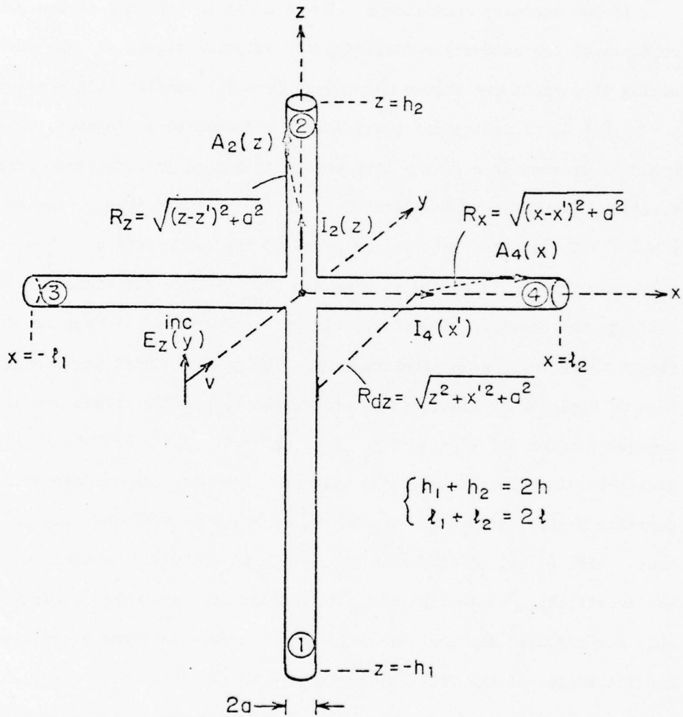
Fig. 13. Crossed wires in normally incident, plane-wave field.
