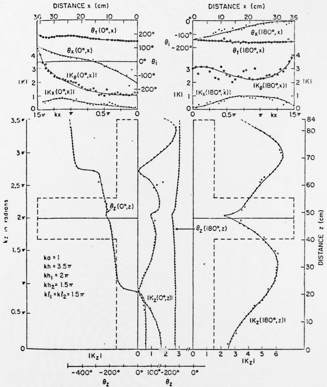
Fig. 51. Measured surface densities of current on crossed cylinders; E-polarization, normal incidence; kh_1 = 2\pi , kh_2 = kl_1 = kl_2 = 1.5\pi .
