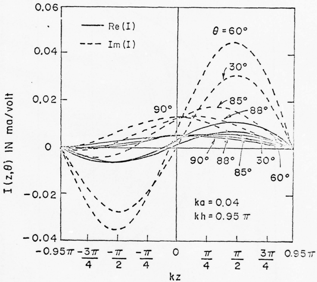
Fig. 11. Real and imaginary currents on parasitic antenna in normally incident, plane-wave field; kh = 0.95\pi .
