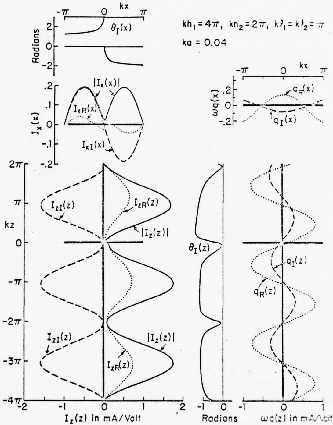
Fig. 17. Theoretical distributions of current and charge per unit length on crossed antenna in normally incident, plane-wave field; kh_1 = 4\pi, kh_2 = 2\pi, k l_1 = k l_2 = \pi.
