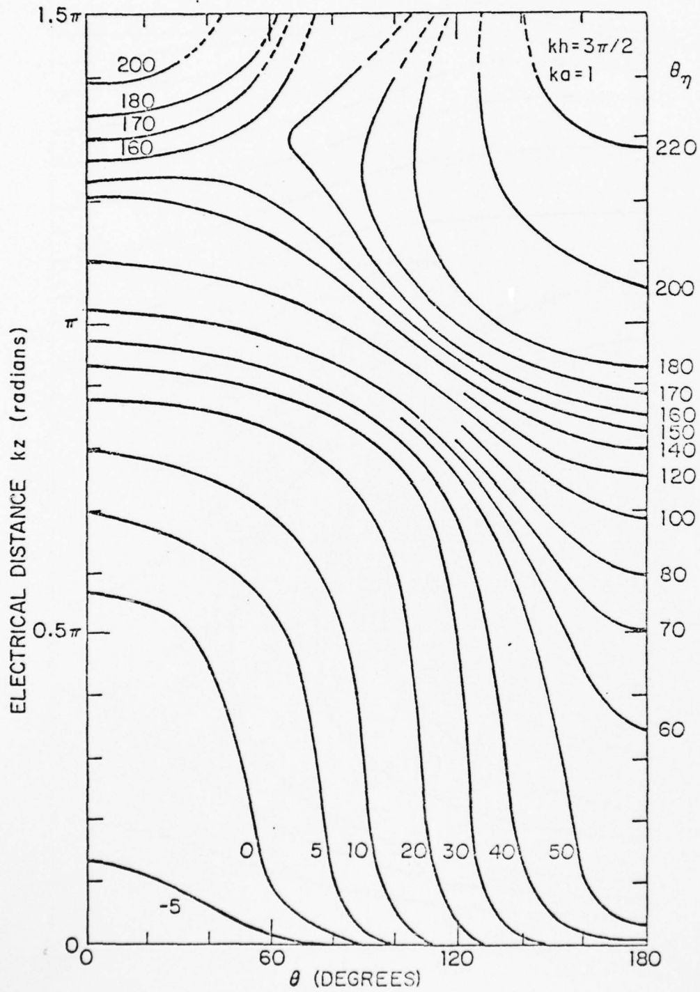
27b. Theoretical contours of constant phase of surface density of charge on tubular cylinder; E-polarization, normal incidence.
