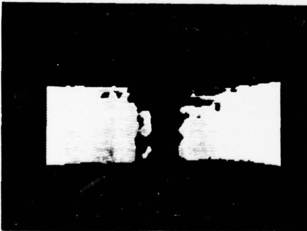
Figure 8. C-scan comparison of bonded and unbonded, flat, fiber glass samples.
