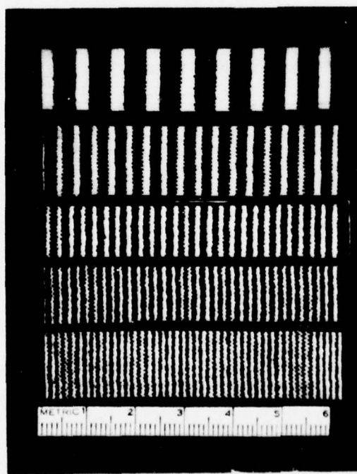
3B. MULTIPLE ECHO ACOUSTIC INTERFEROMETRIC RESULTS
