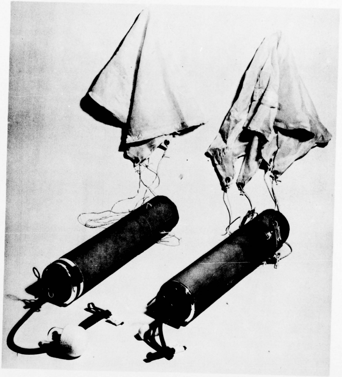
Fig. 7 - Dewar samplers
