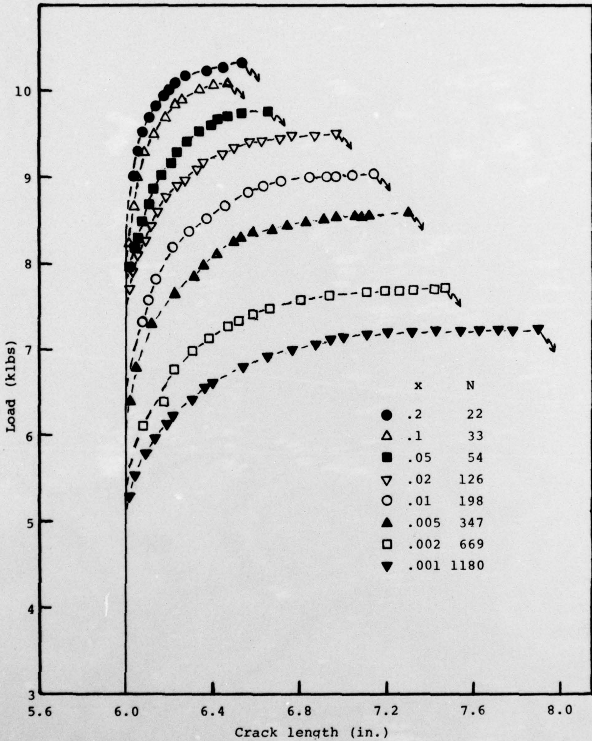
Fig.4. Crack growth curves for different cyclic load increments in 7075-T6 alloy.
