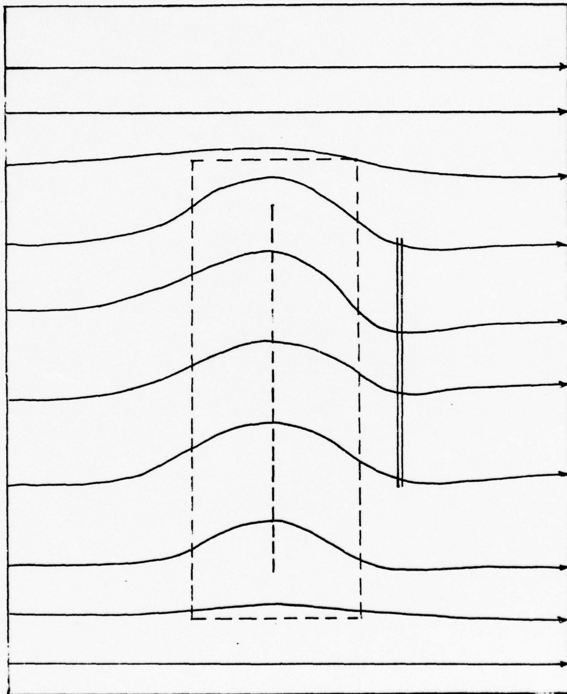
Figure 10. 9^\circ \times 1.5 km mountain range case. Six-layer fine resolution model streamlines for \sigma = .91667 . Dashed lines depict outline of mountain range and mountain ridge line.
