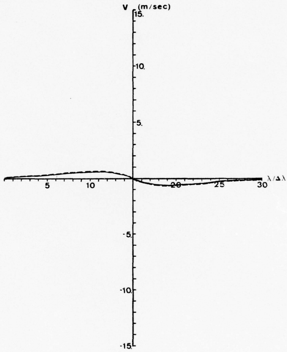
Figure 7. 3° x 1.5 km mountain case. Analytic v profiles for \sigma = 0.0 at 44°N computed on a 30 point grid (dashed curve) vs. a 60 point grid (solid curve).
