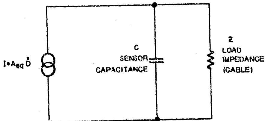
Figure 3. Equivalent Circuit of D-dot Sensor
