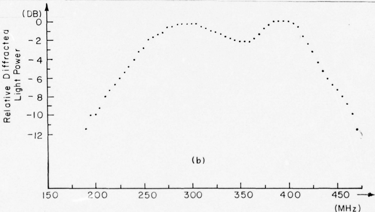
Fig. 10 (a) Frequency Responses of the Bragg-Diffracted Light Power for the Individual Acoustic Waves, (b) Frequency Response of the Bragg-Diffracted Light Power for the Combined Acoustic Waves.
