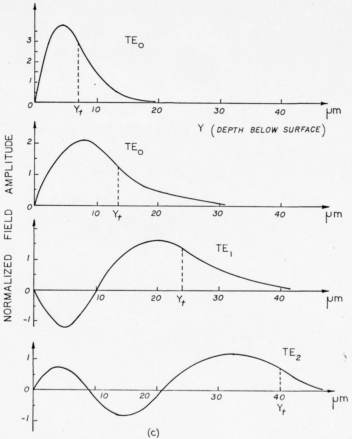
Fig. 3 c) Profiles of the TE Optical Waveguide Modes in Y-cut \text{LiNbO}_3 Out-Diffused Layers ( Y_t is the Turning Point).
