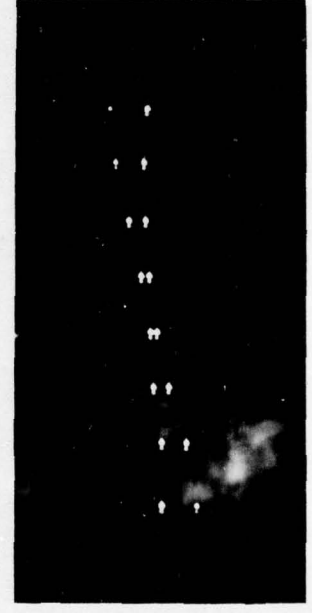
FIG. 31 Spectrum Analysis of RF Signals Using Guided - Wave Acousto - Optic Bragg - Diffraction : (a) Measurement of Inter-Modulation between Two Frequency Components f_1 and f_2 (b) Deflected Light Spots from Two Frequency Components of Various Frequency Separation and Power Level
