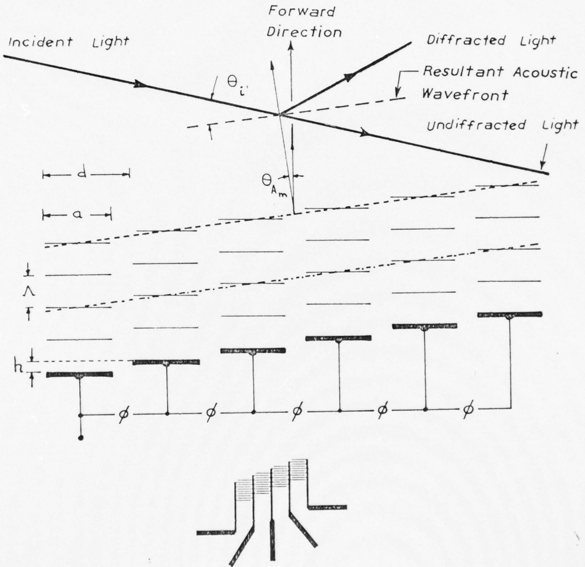
Four-Element stepped Array Transducer
