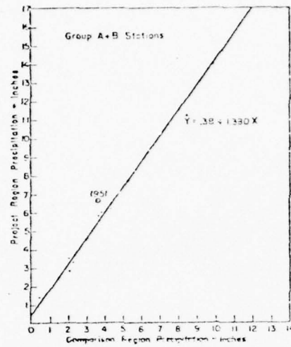
Fig. 5-1. Scatter Diagram showing the relationship between precipitation amounts in the project area and comparison area for a 10-year period, (from Brier and Enger, 1952)
