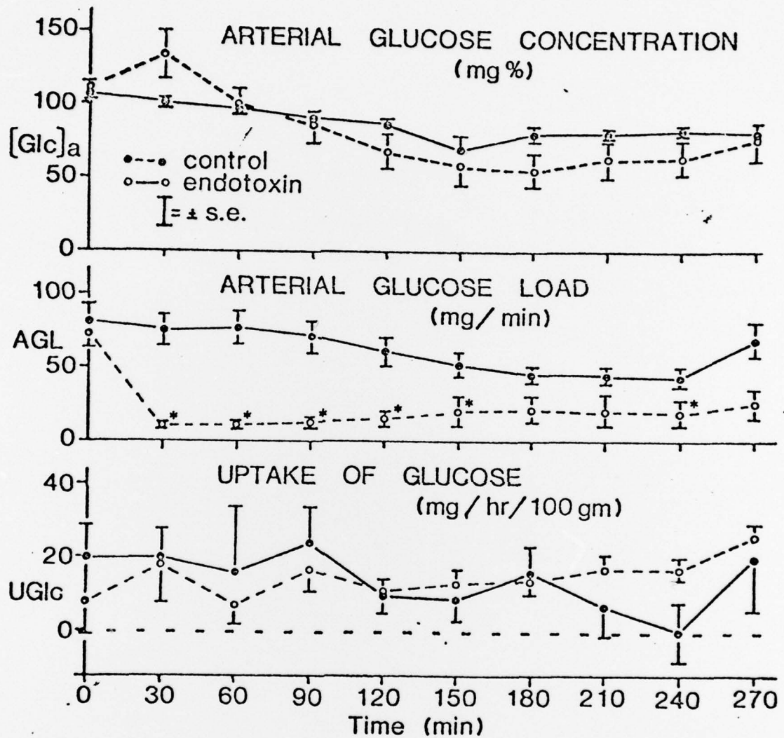
FIGURE 2. Arterial glucose concentration ([Glc] a ), arterial glucose load (AGL), and uptake of glucose (UGlc) results from the innervated isolated forelimb preparations. Values are means (N = 8) ±SE. *Significantly different from control, (p < 0.05).
