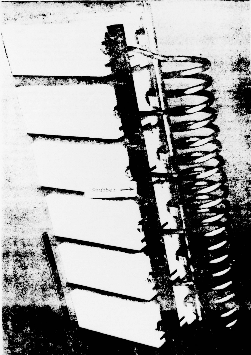
Figure 1. 4 Kilojoule PFN
