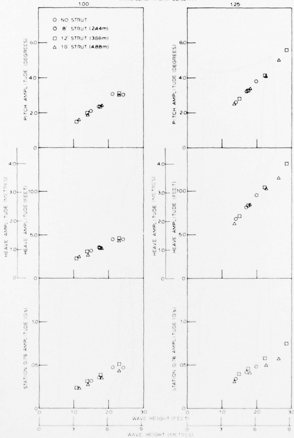
Figure 5 - Pitch, Heave, and Acceleration at Station 0.76 Single Amplitude Values versus Wave Height for a Ship Speed of 20.0 Knots
