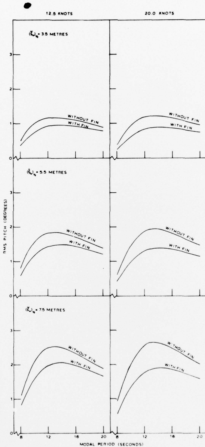
Figure 7 - Comparison of Analytical Predictions of the Pitch Motion of the Mariner with and without a Bow Fin
