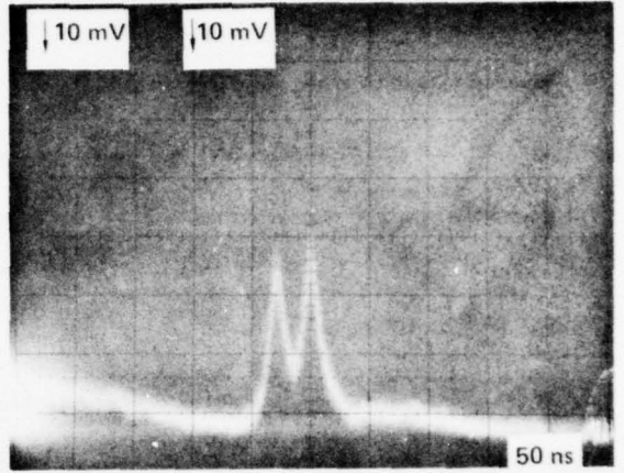
b. SUPERIMPOSED SPOTS 30 ns DELAY AND ADDED
