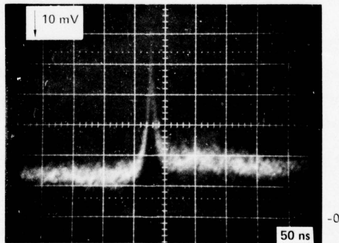
b. READOUT WITH 320 SCANS RECORDING ENERGY OF 1.25 mj/cm 2
