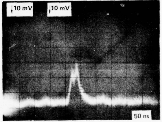
d. SUPERIMPOSED SPOTS 15 ns DELAY AND ADDED
