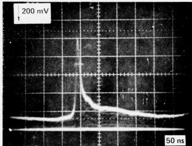
a. READOUT WITH 32 SCANS RECORDING ENERGY OF 12.5 mj/cm 2
