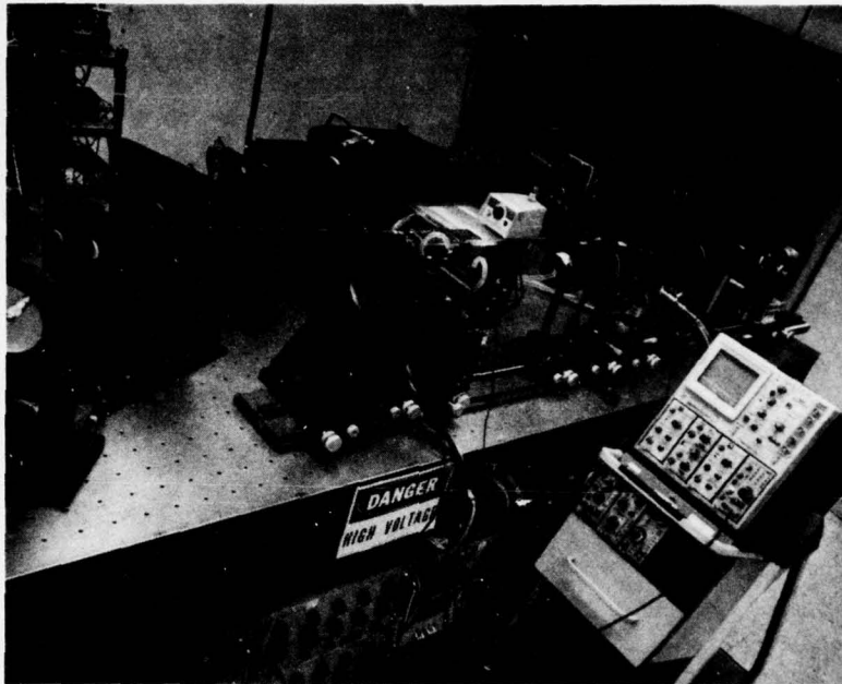
Figure 2-2. Photograph of the OTIS Scanner
