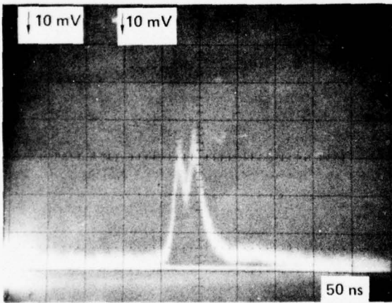
c. SUPERIMPOSED SPOTS 20 ns DELAY AND ADDED
