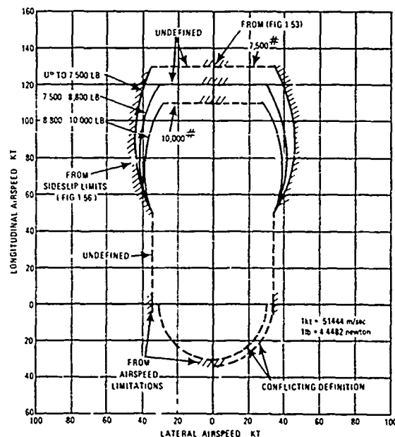
Figure 3 Complete Airspeed Limitation
