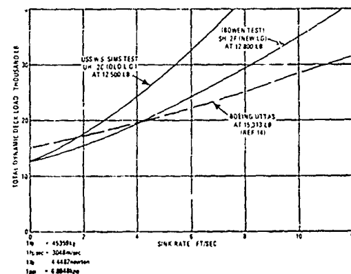
Figure 8 Deck Loads and Pressures
