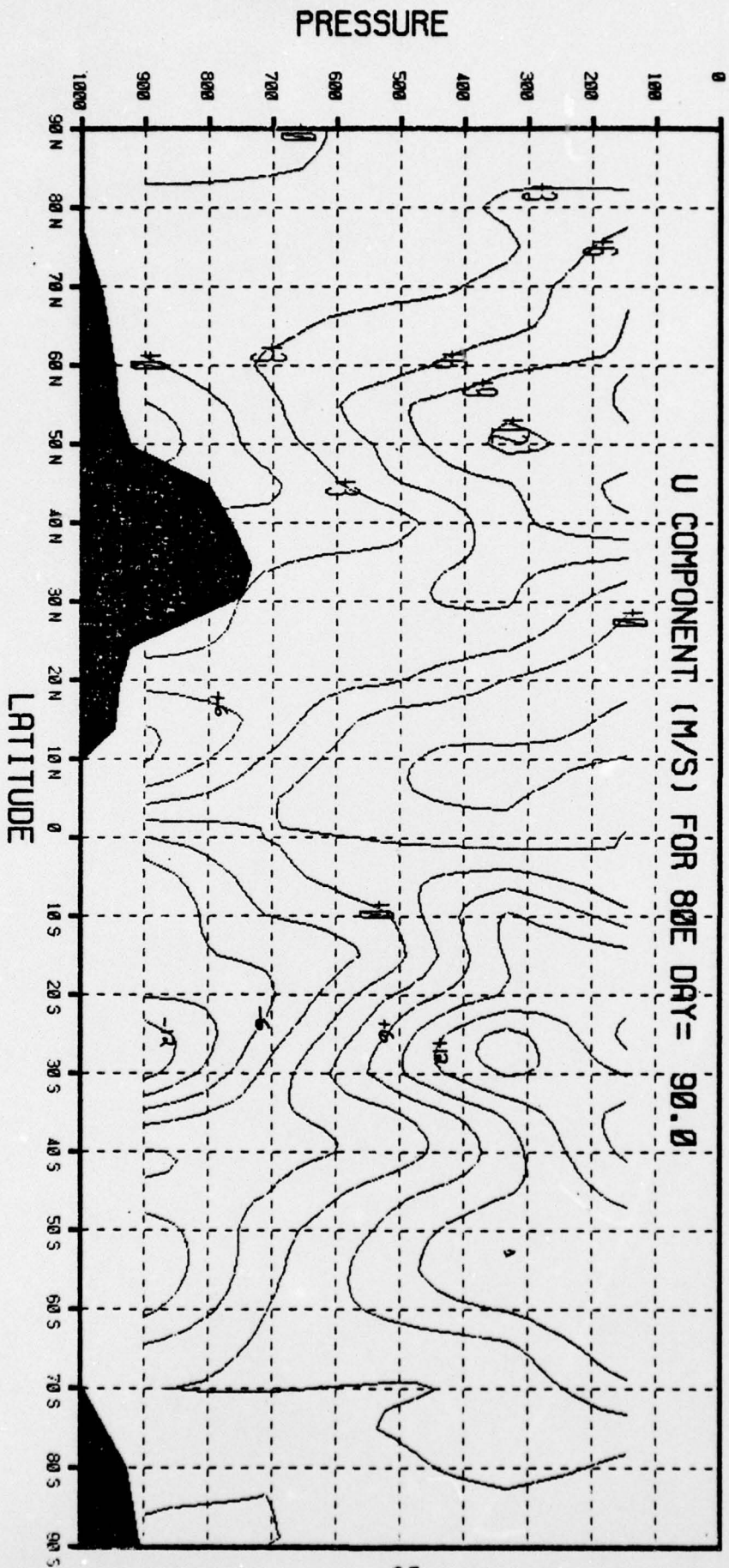
Figure 5d. Zonal u component for day 90 (April 11).
