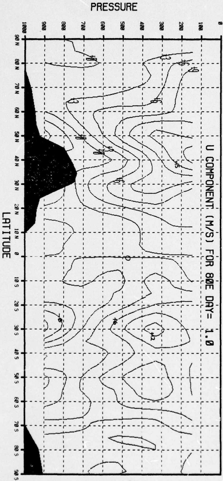
Figure 5a. Zonal u component for day 1 (January)
