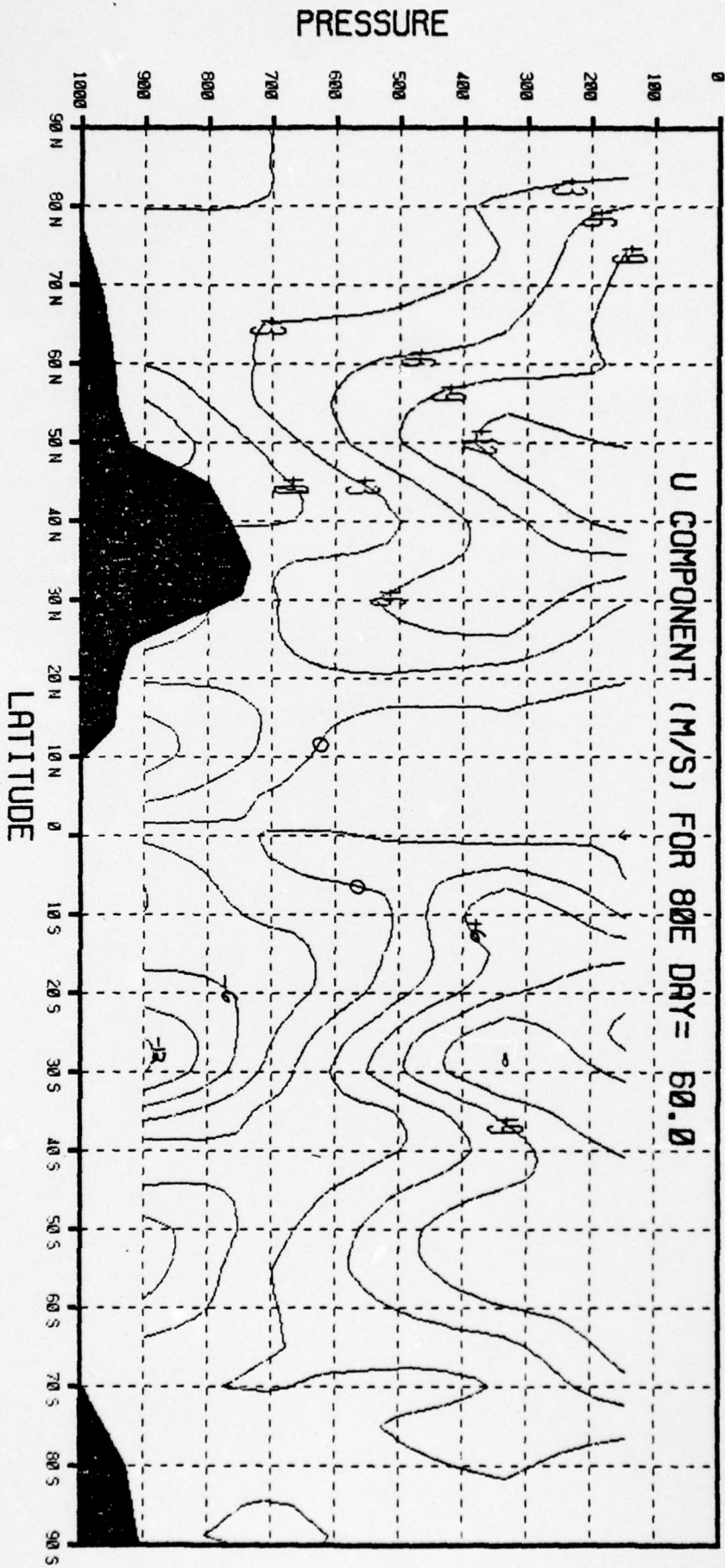
Figure 5c. Zonal u component for day 60 (March)
