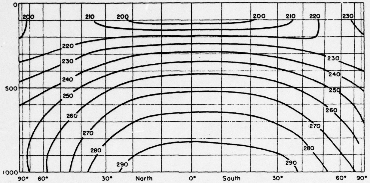
Figure 3a. The time-and-longitude averaged temperature ( \bar{T} ) in January as estimated by Palmén and Newton (1969). Values are in degrees K.
