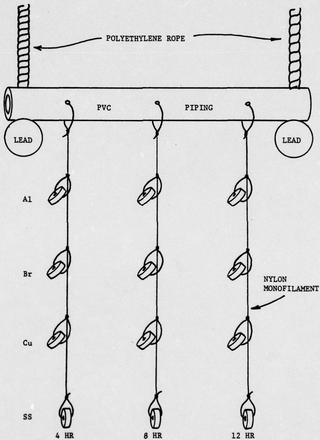
Figure 3. Mooring array.
