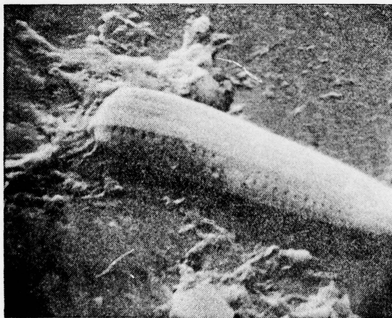
Plate 8.b. Stainless steel immersed 8 hrs, 5900X. Solitary diatom.
