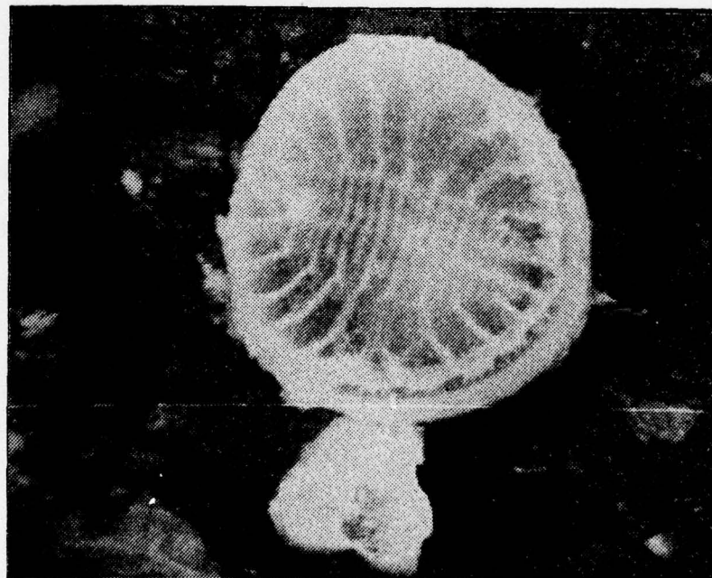
Plate 2.b. Aluminum immersed 3 weeks, 2230X. Solitary diatom.
