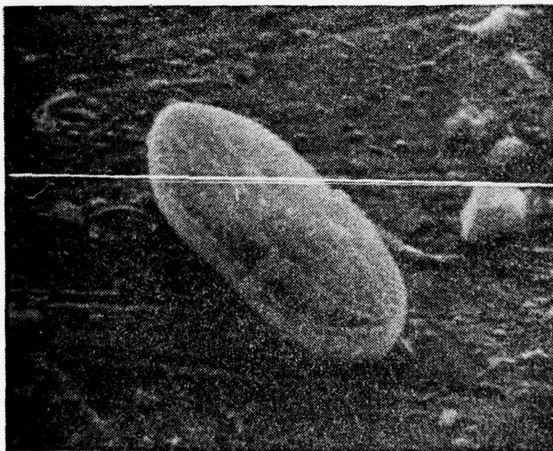
Plate 10.b. Stainless steel immersed 3 weeks, 2600X. Solitary diatom.
