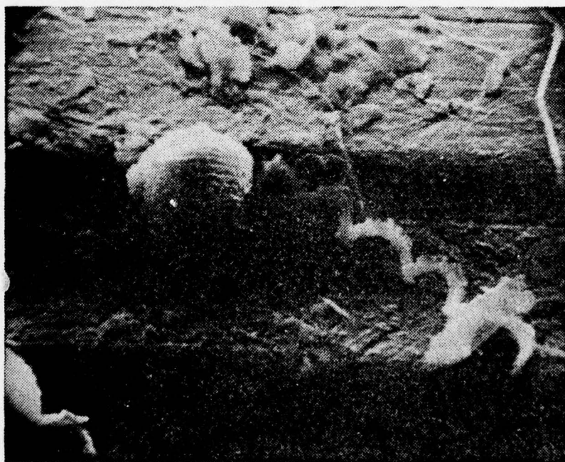
Plate 16.b. Stainless steel immersed 3 weeks, 1200X. Stalked protozoan.
