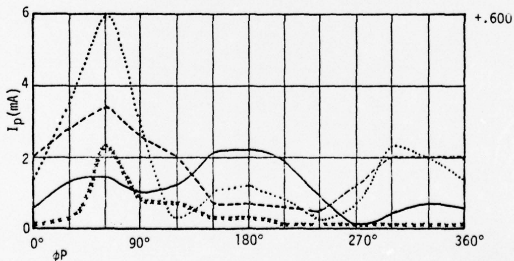
FIGURE 7B: CURRENT DISTRIBUTION ( Z = .6, .8, 1.0 )
