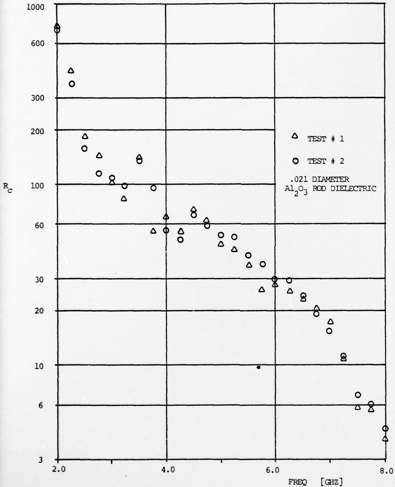
FIGURE 13 COUPLING IMPEDANCE OF 'T' SHAPE HELIX
