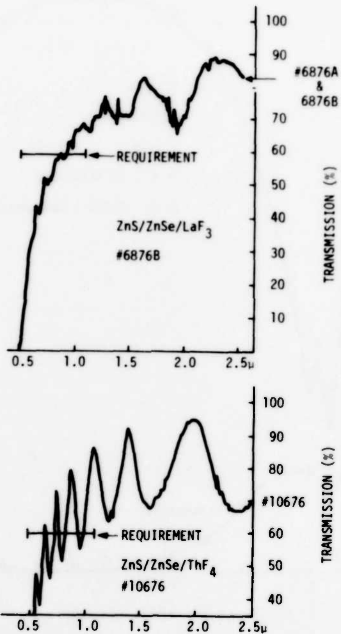
Figure 17. Transmission of Coated ZnS Windows between 0.5 and 2.5 μm
