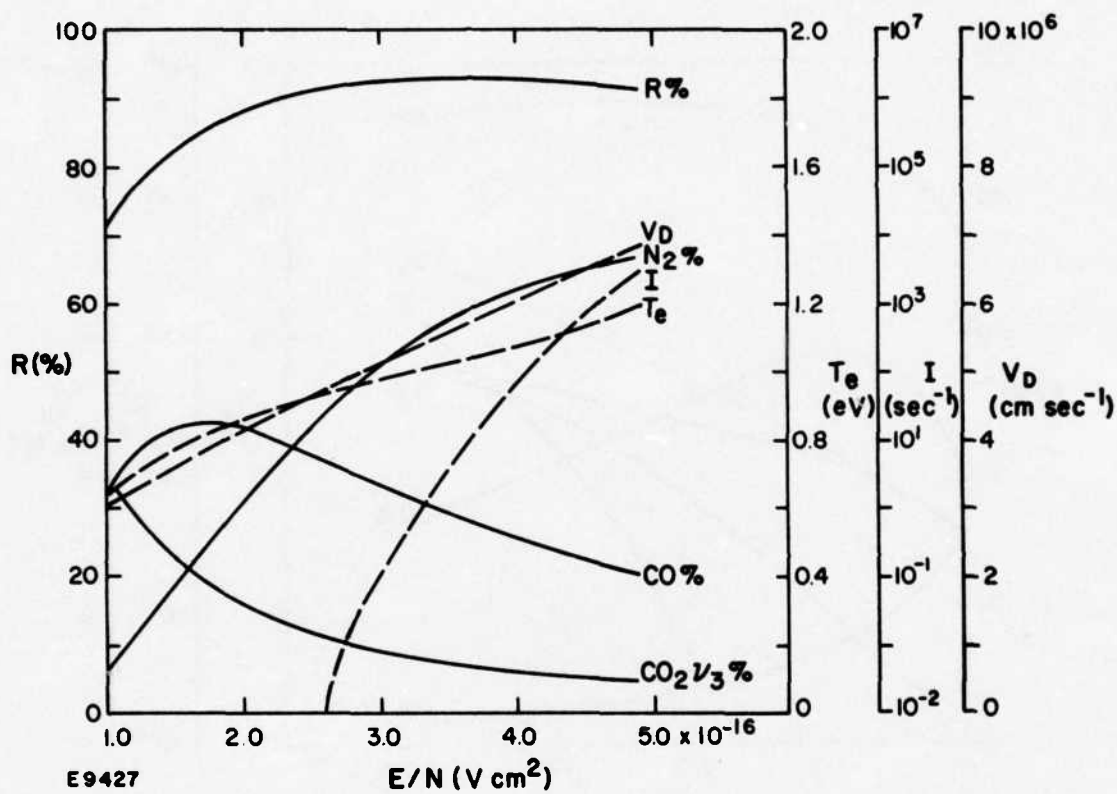
Fig. 2(b) Fractional Energy Pumped into Vibrational Modes by Electrons, as Function of E/N , in the Gas \text{N}_2:\text{CO}_2:\text{CO}:\text{H}_2 (8.2: 1: 0.6: 0.18).
