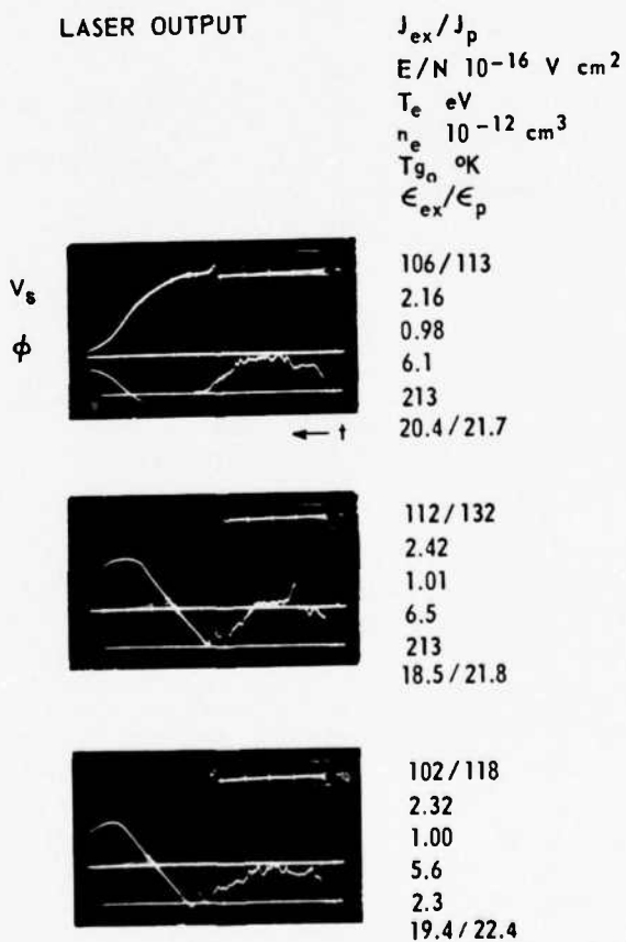
Fig. 21 Laser Output for N_2:CO_2:CO:H_2 (8.22:1:0:0.19) at Low Temperature.
