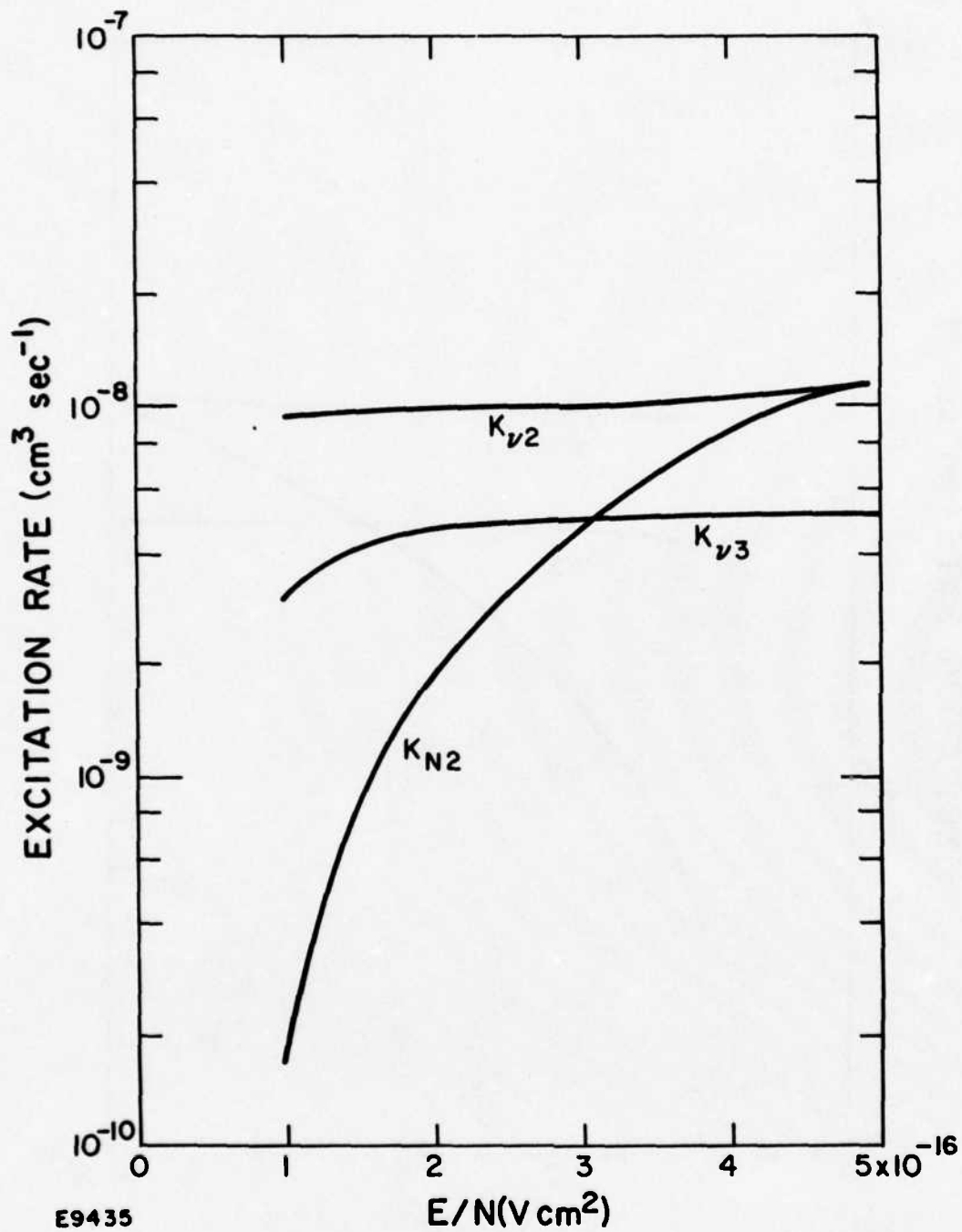
Fig. 3(d) Electron Impact Vibrational Excitation Rates in the Gas \text{N}_2:\text{CO}_2:\text{CO}:\text{H}_2 (4. 1: 1: 0: 0.09).
