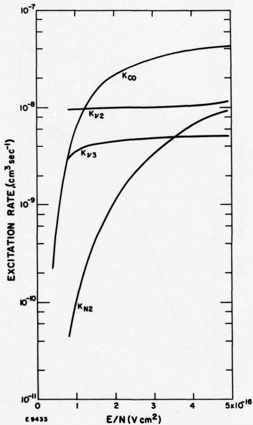
Fig. 3(a) Electron Impact Vibrational Excitation Rates in the Gas \text{N}_2 : \text{CO}_2 : \text{CO} : \text{H}_2 (8. 2: 1: 0. 6: 0. 18).
