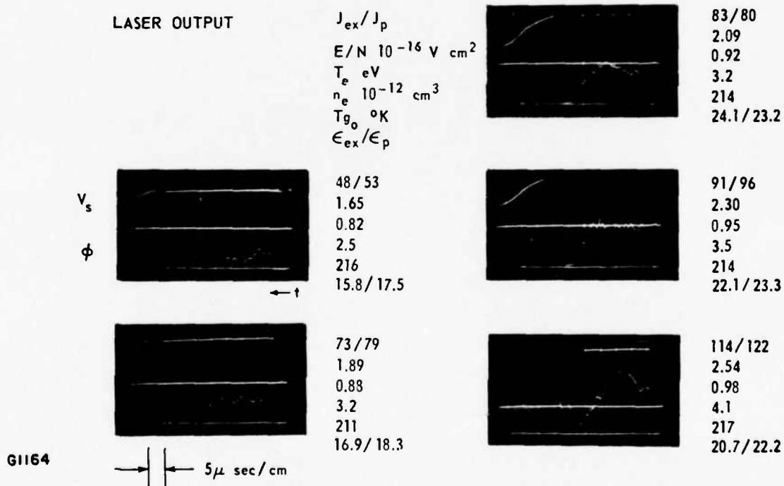
Fig. 17 Laser Output for \text{N}_2:\text{CO}_2:\text{CO}:\text{H}_2 (3.67:1:0:0.19) at Low Temperature.
