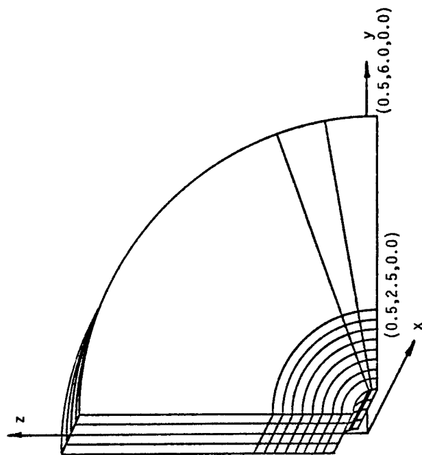
Figure 21. 108-Element Finite Element Mesh, Double Corner Crack Problem, d/t = 1.0
