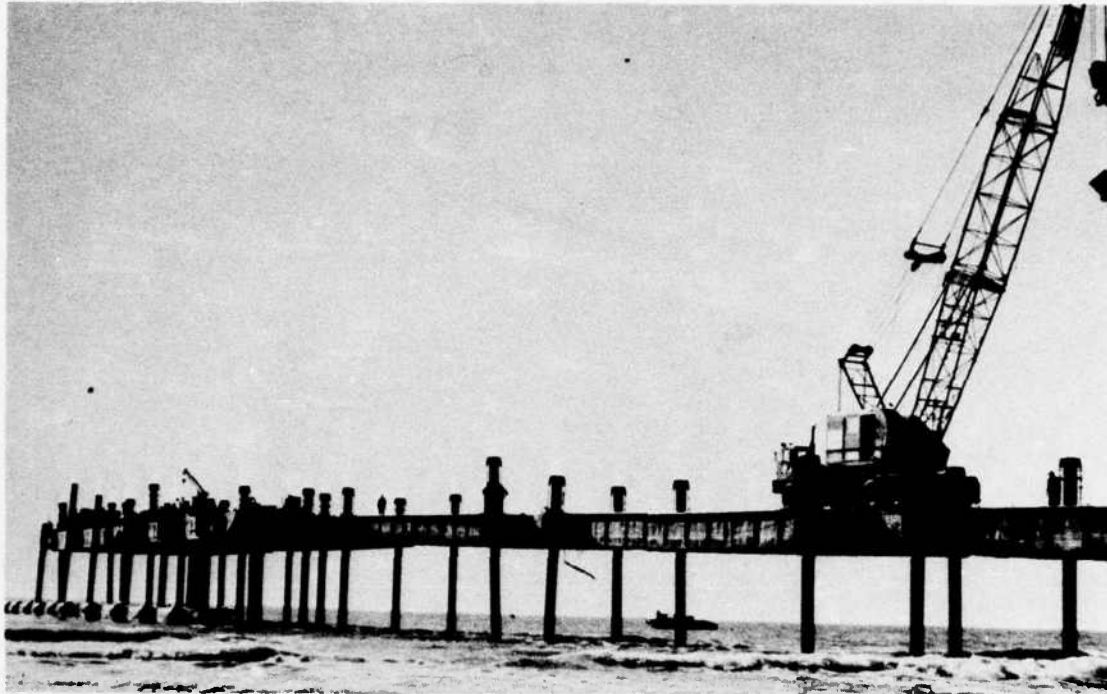
Figure 13. P&H Model 8100, 90-ton (82-Mg) rated capacity truck crane moving to pichead on causeway.
