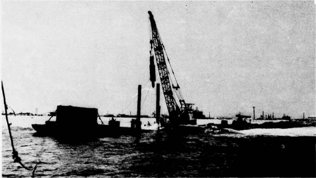
Figure 3. Placing and driving pile during 6-foot (1.8-m) wave.
