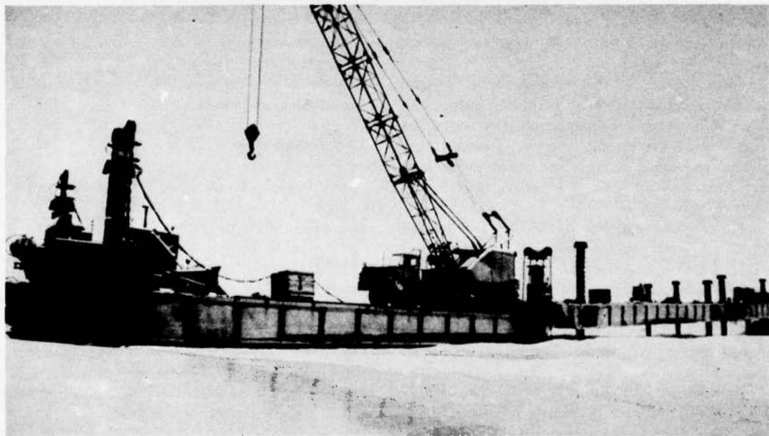
Figure 4. Elevating section with crane and tractor on board.
