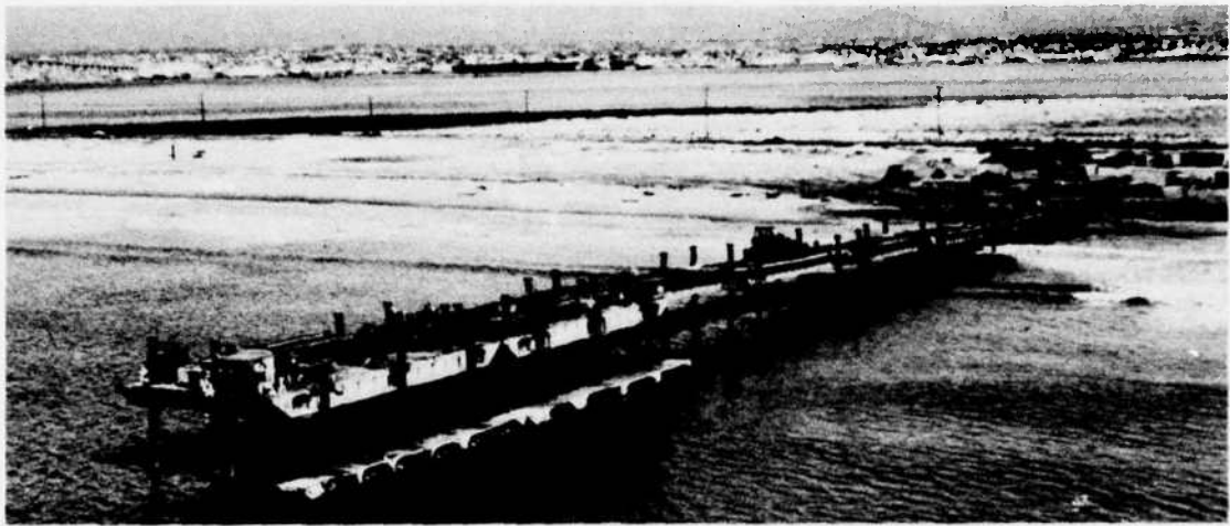
Figure 11. Foam bumpers secured to two 1x15 pontoon strings and restrained by six steel piles.
