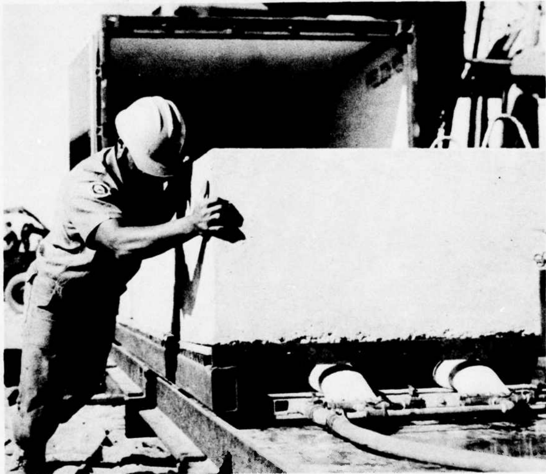
Figure 24. Air-bearing transporter.
