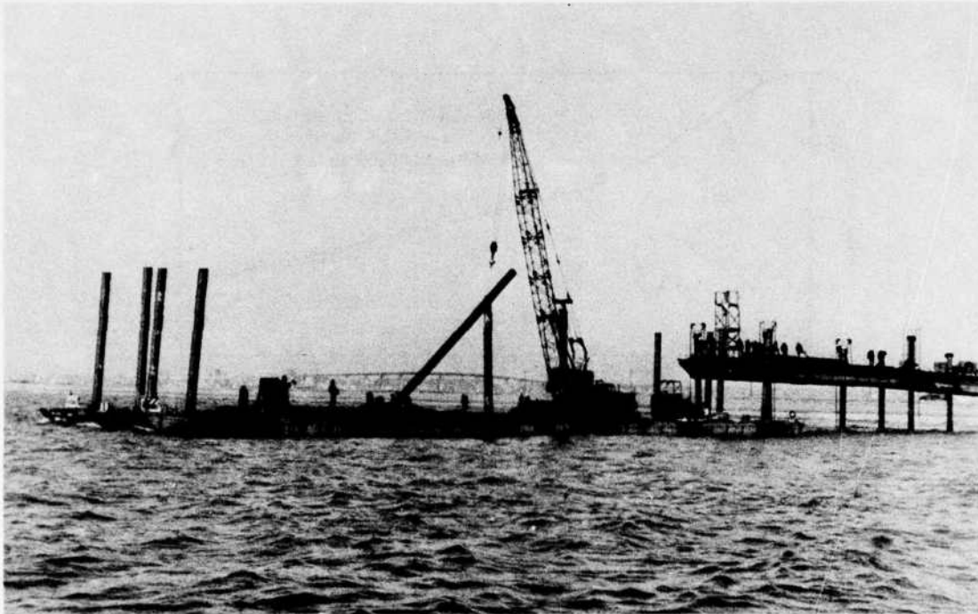
Figure 5. Hydraulic jacks lifting causeway section while piles are being placed in following sections.
