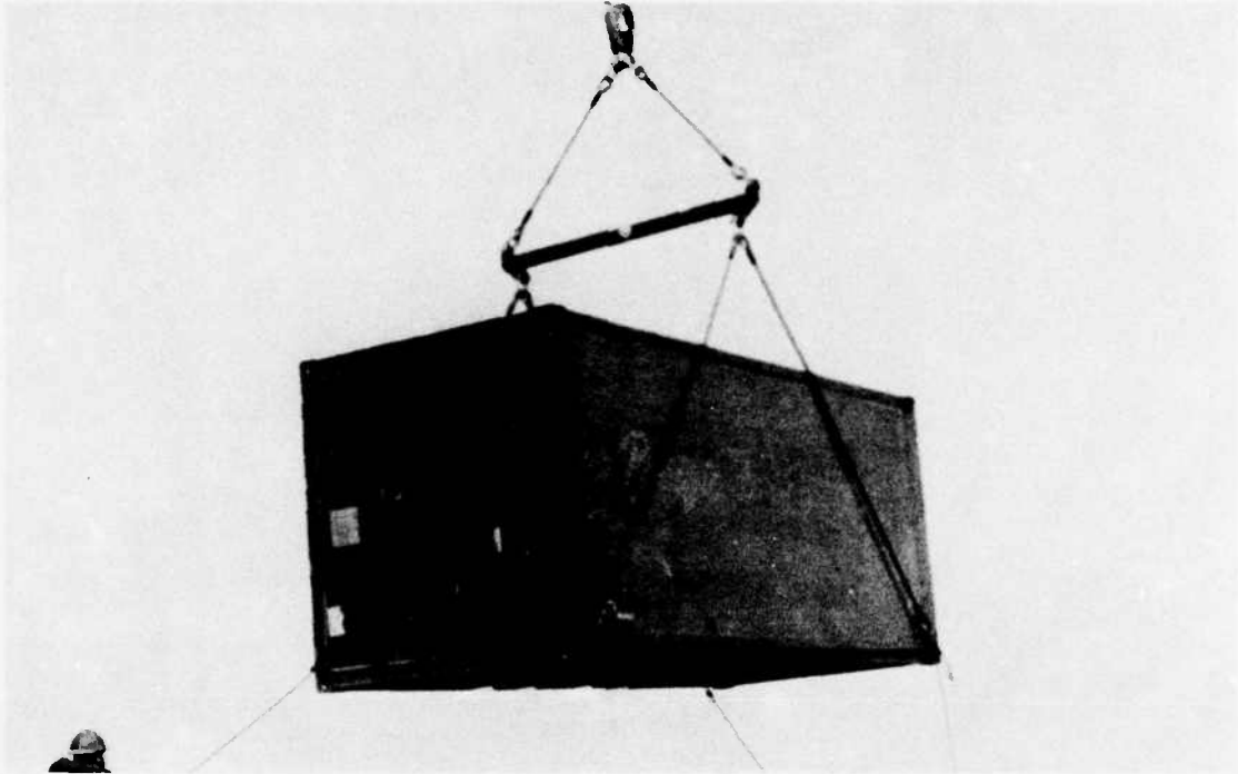
Figure 15. Wire rope slings with bulb hooks.
