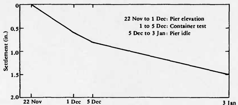
Figure 6. Settlement of elevated pier.
