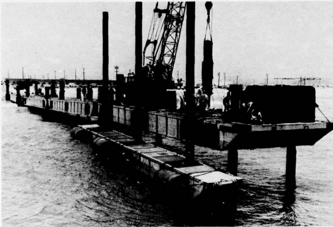
Figure 2. Four-section elevated pier, Phase I tests.
