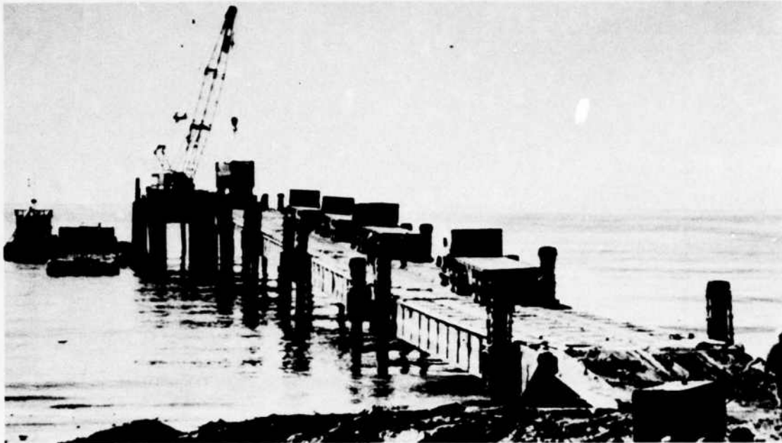
Figure 26. Unloading containers from three-section causeway ferry at elevated pierhead.
