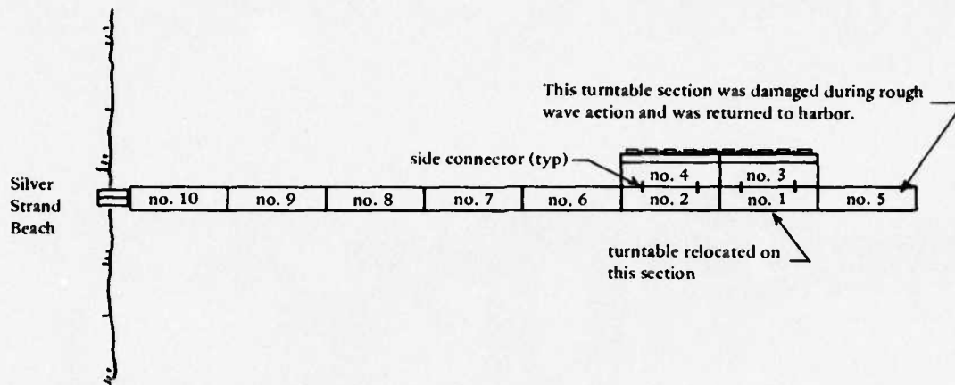
Figure 25. Location of sections of elevated causeway for Phase II operations.
