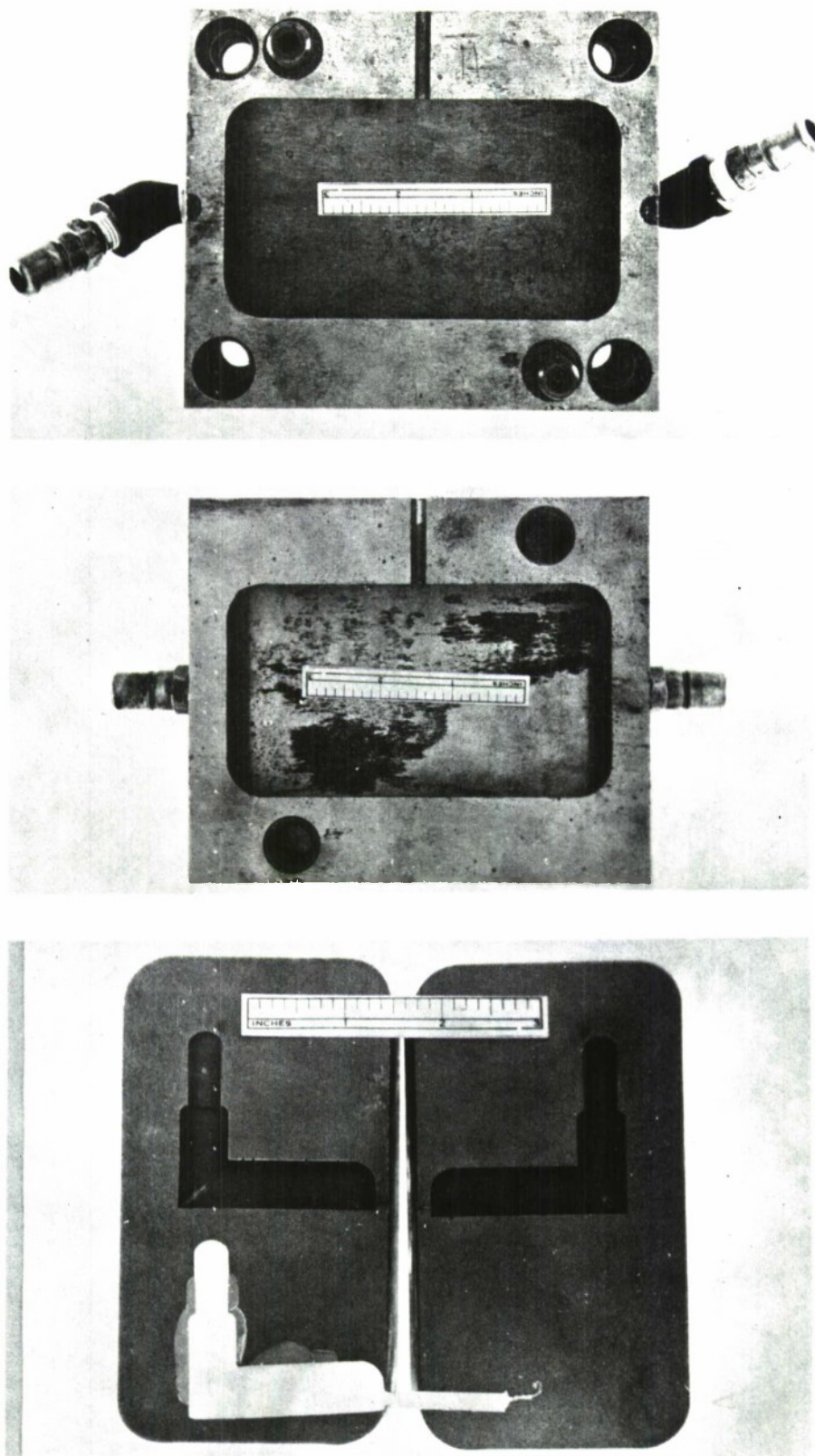
Figure 4. Standard steel D-M-E die base with cooling channels (upper and middle photographs) and REN RP3269-1 epoxy mold with polyethylene component produced for the M16 Rifle Safety Flag, PN 8448666.
