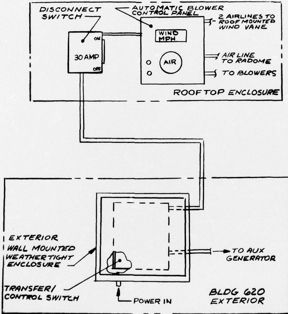
Figure 42. Wiring Path
