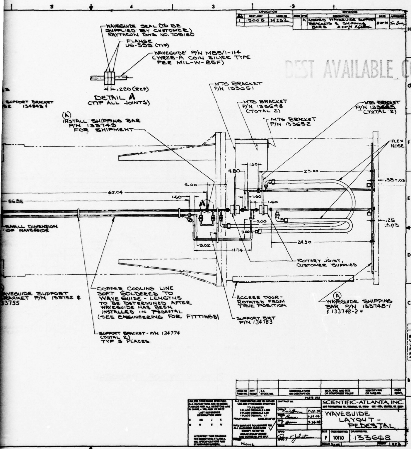
Figure 13. Waveguide Layout Pedestal
