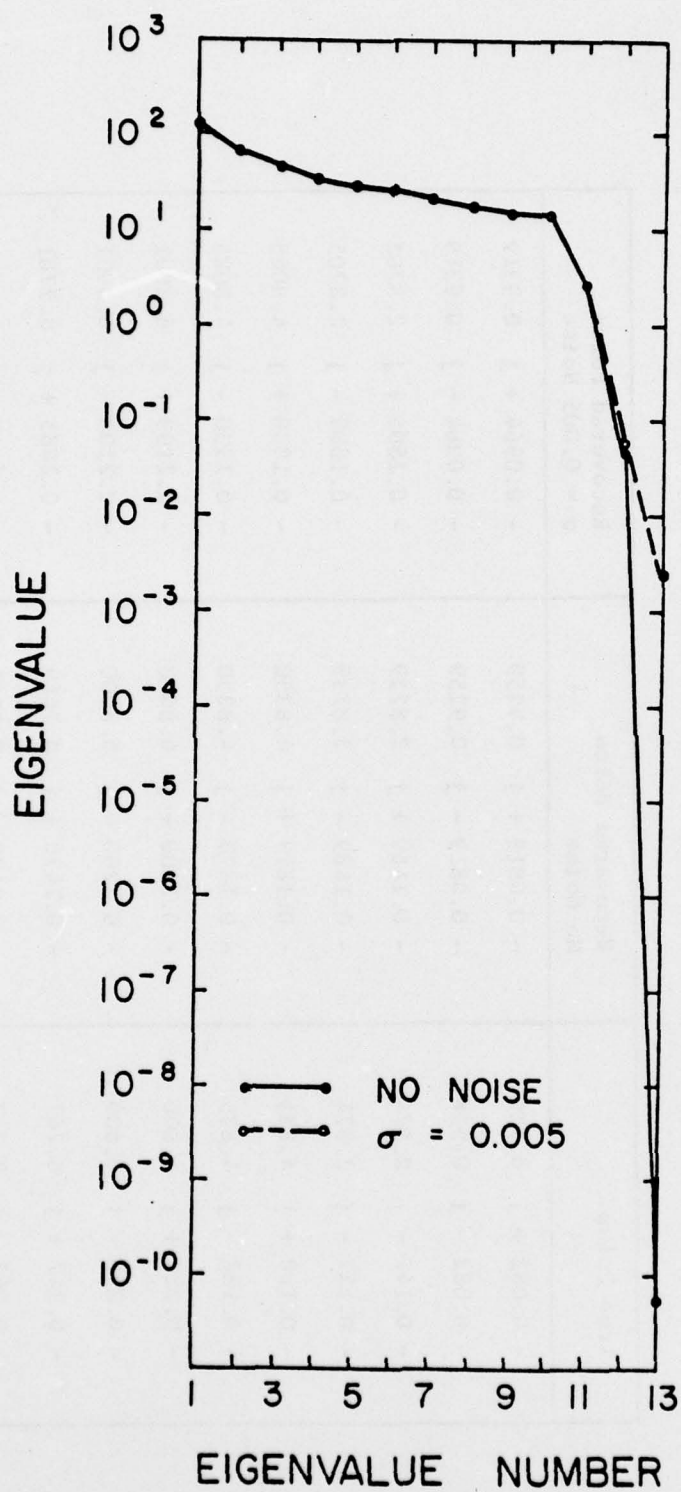
Figure 4.4. Resulting eigenvalues from response generated using poles of Table 4.2 for non-noise case and noise with \sigma = 0.005 .
