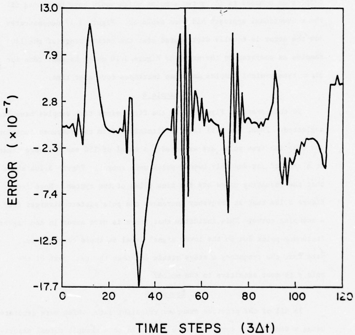
Figure 3.17. Original response minus the reconstructed response of Example 7.
