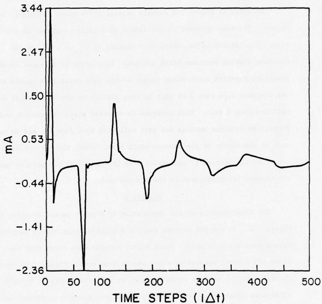
Figure 3.2. Source current on 1.0 m dipole.
