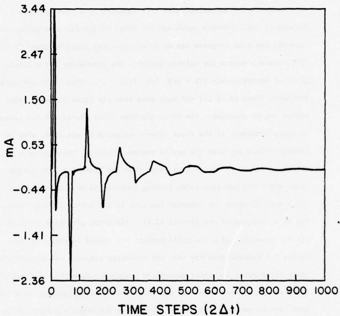
Figure 3.5. Reconstructed transient response using extracted poles of Example 1.
