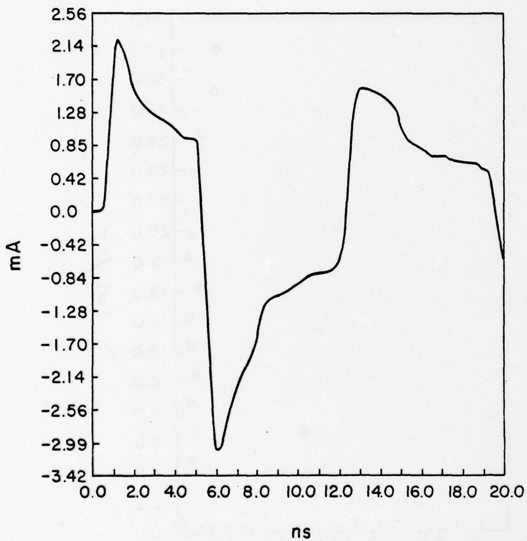
Figure 3.19. Original experimental data of Example 9.
