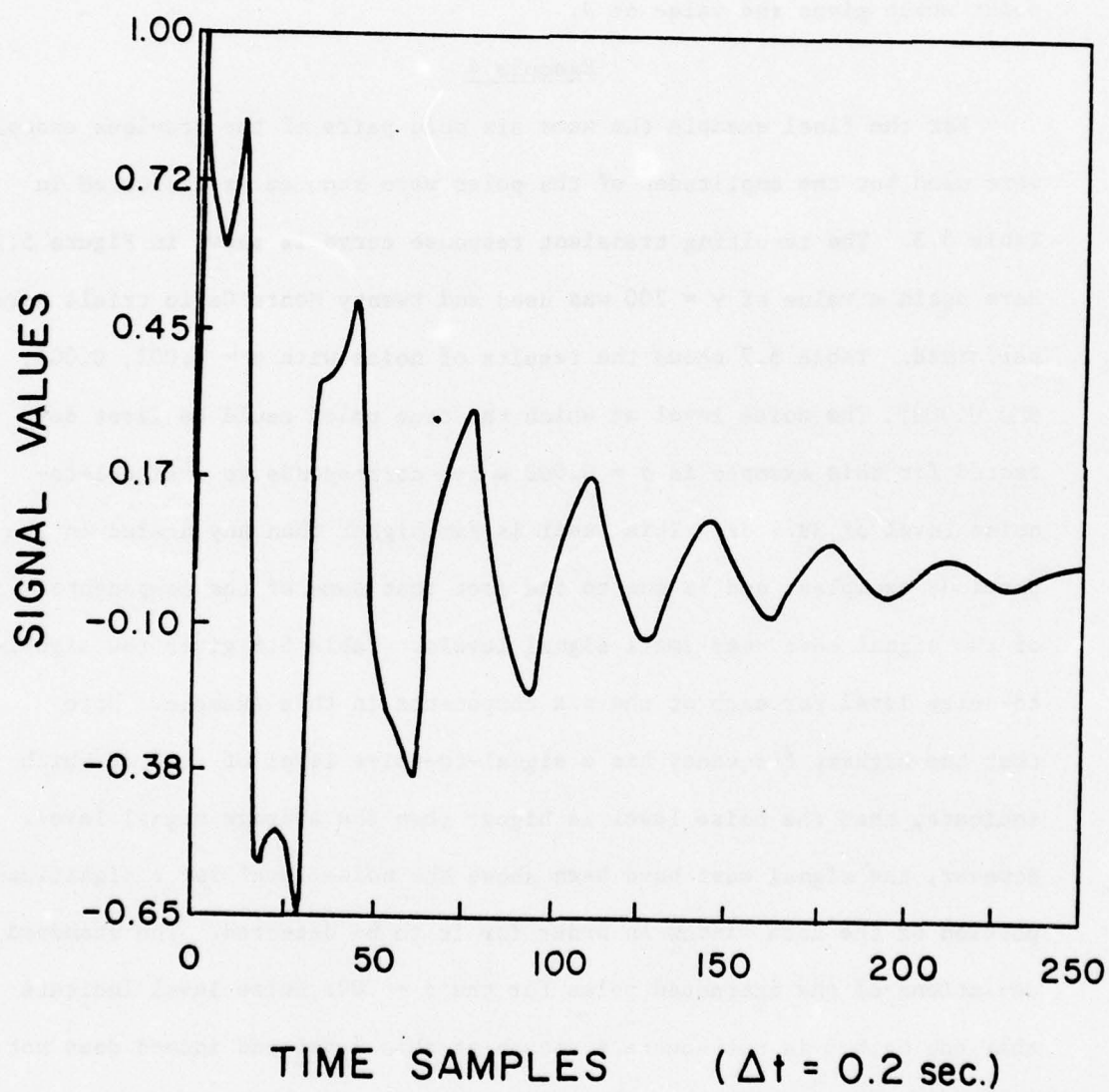
Figure 5.2. Transient waveform used in Example 4.
