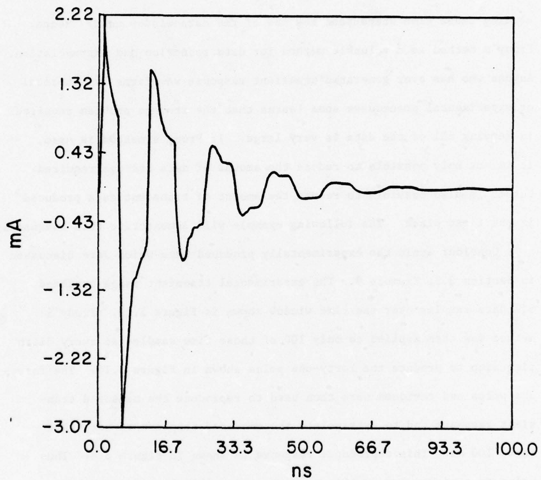
Figure 6.6. Extrapolated current response for 1.0 m monopole of Example 9, Chapter 3.
