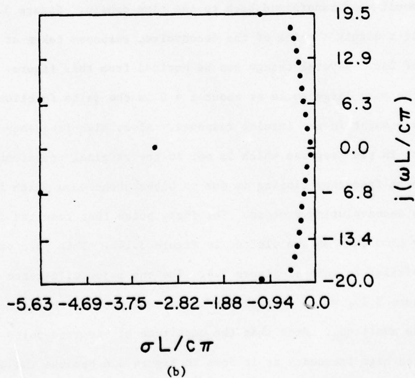
Figure 3.13. (a) Data window starting at time step sixty-one, Example 5. (b) Resulting pole locations.
