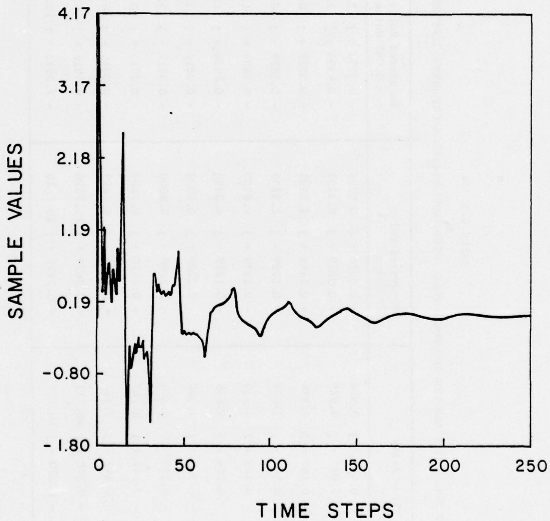
Figure 4.1. Transient response resulting from the six pole pairs of Table 4.1.
