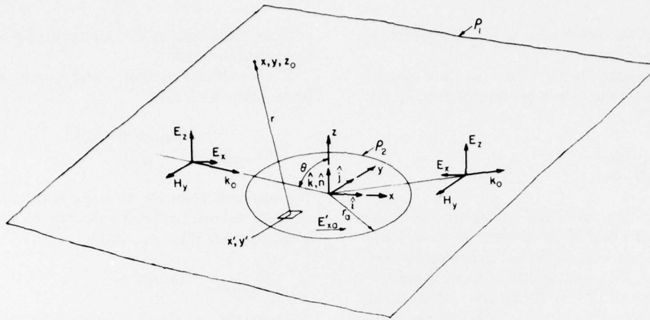
Figure 2. Uniform earth of resistivity \rho_1 containing an anomalous area of resistivity \rho_2 . The electromagnetic field vectors refer to the incident (at an angle \theta -left) and reflected (right) waves. E'_{x\alpha} is the perturbed electric field on the anomaly. Surface coordinates are primed and spatial coordinates are unprimed. Both coordinate systems have coincident origins. The radius of the circular area is r_a .
