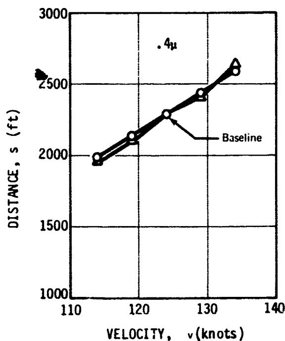
Figure 18.—Effect of Winds and Brake Application Velocities on Stopping Distance (KC-135)
