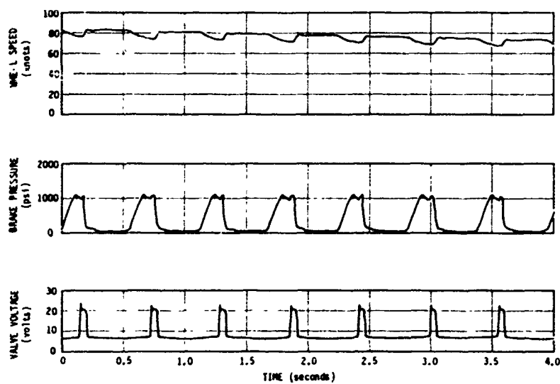
Figure 9.—B-52H Simulator Performance (Baseline Airplane) Intermediate Mu (.25)
