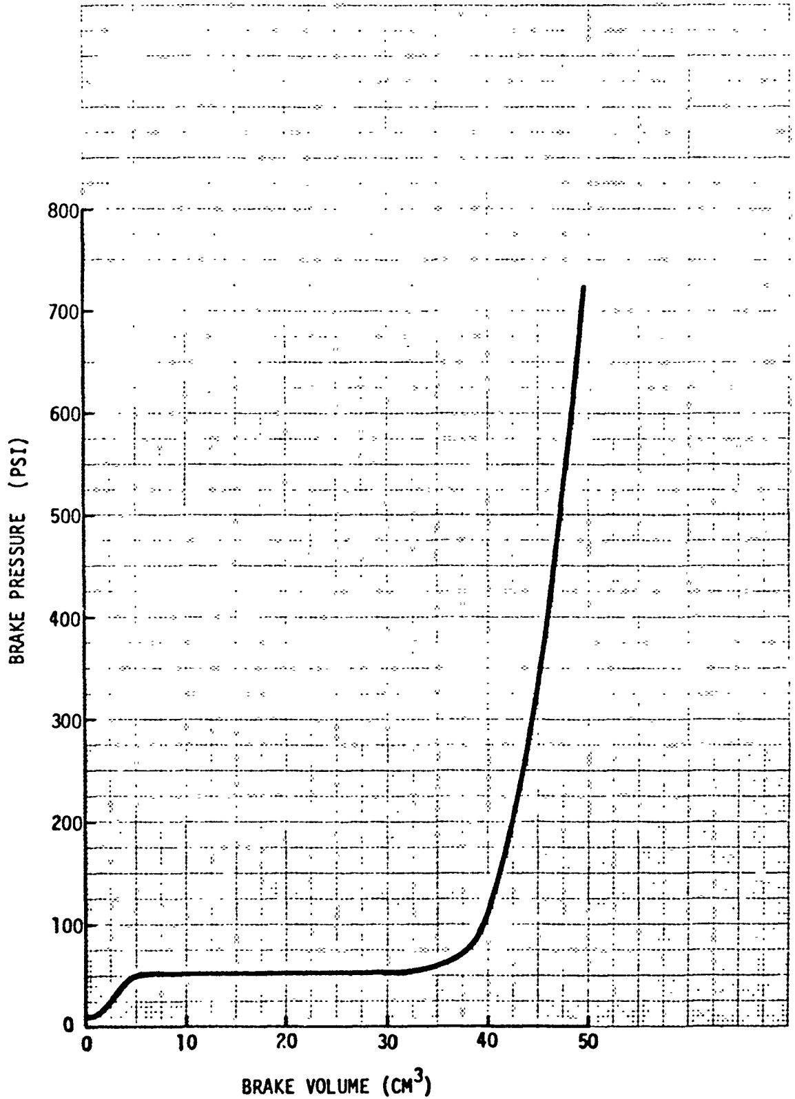
Figure 6.—B-52H Brake Pressure - Volume Characteristic
