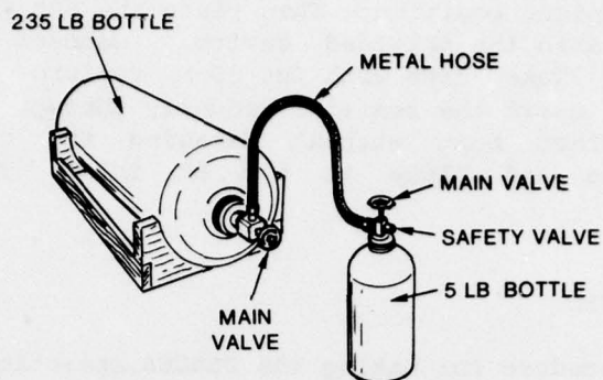
Figure 9. Setup for charging \text{SF}_6 bottle.
