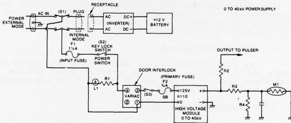
Figure 2. High-voltage power supply.
