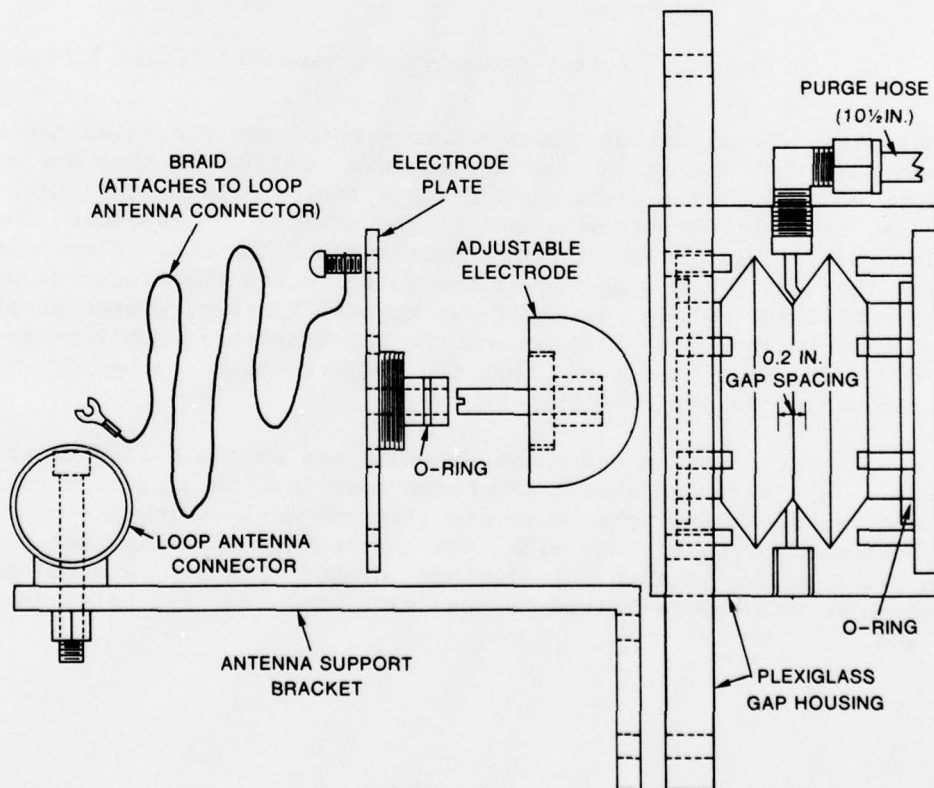
Figure 8 Gap housing assembly (scale 1.8:1).
