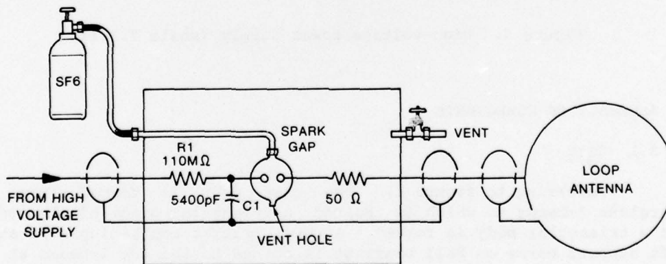
Figure 3. Pulser.
