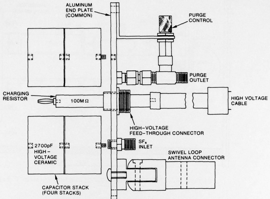
Figure 6. Pulser ground-plate assembly (scale 1.8:1).
