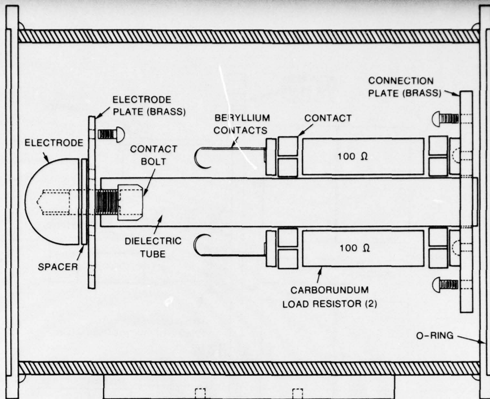
Figure 7. Pulser housing, cylinder (scale 1.8:1).
