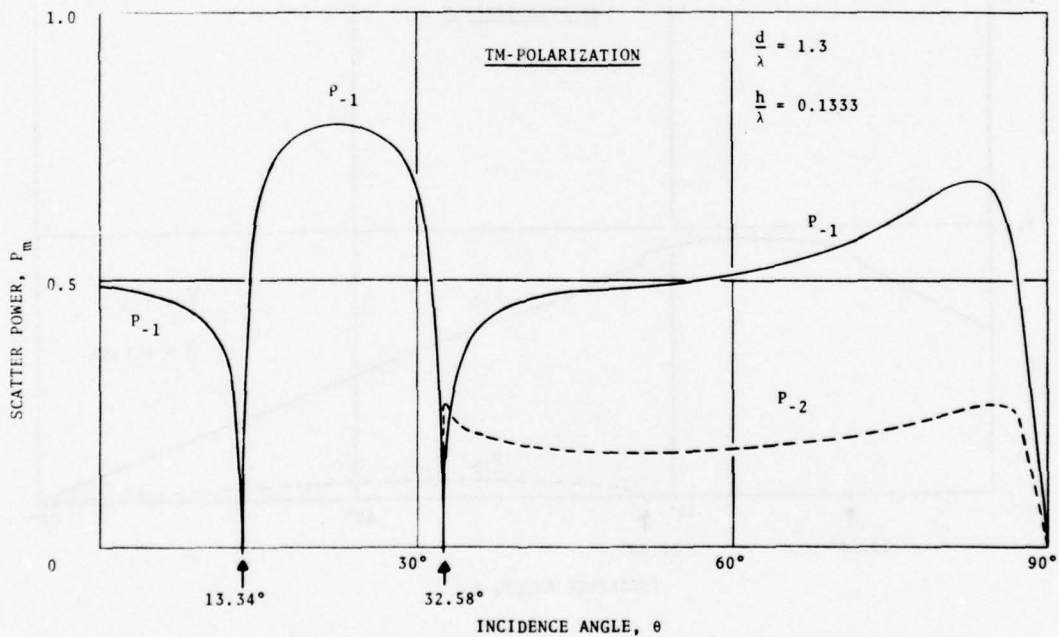
Fig. 5b. Powers P_m of propagating space harmonics vs. arrival angle \theta of incident wave (Profile 1; Spectral orders: m = -1, -2 ).
