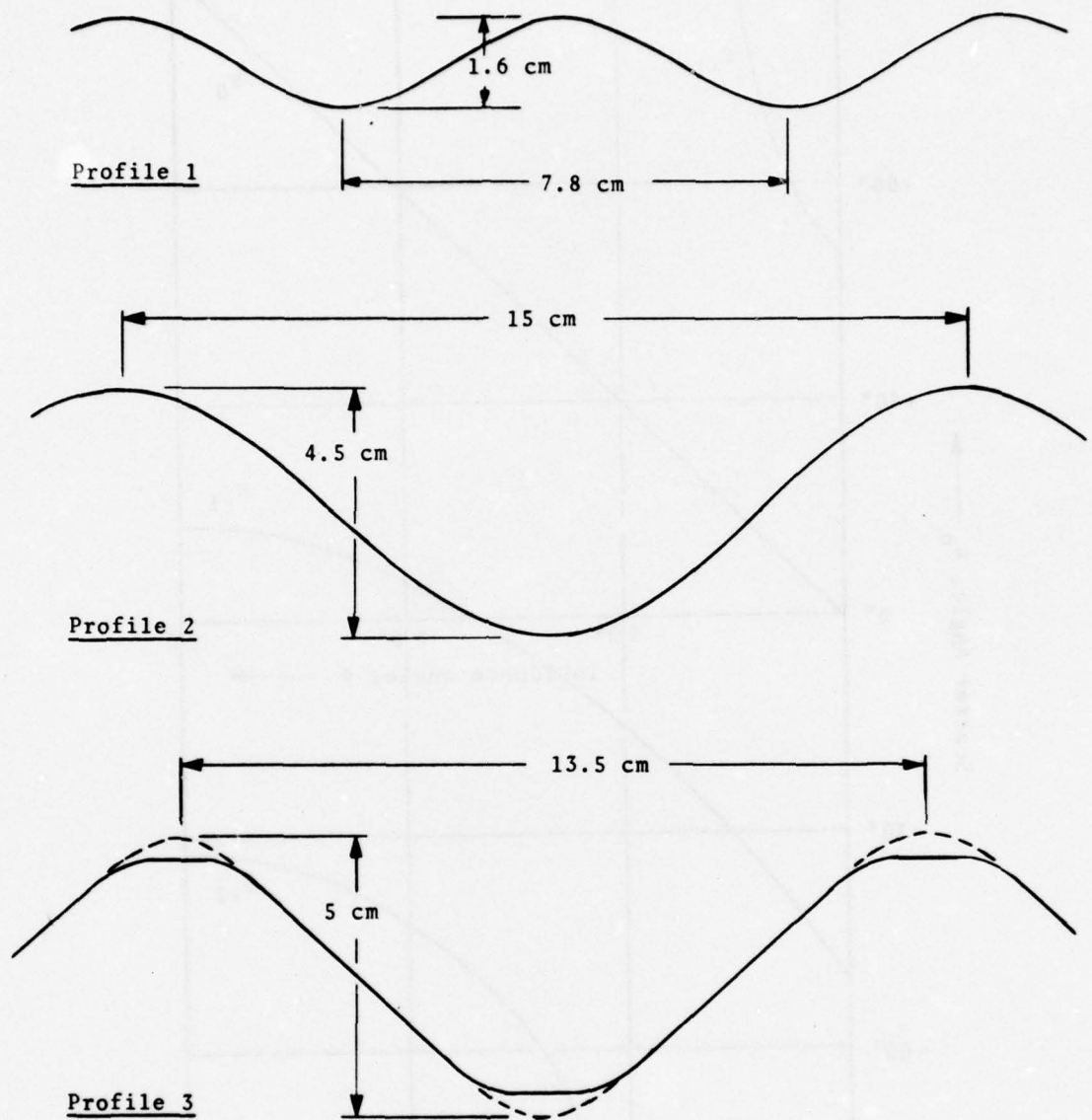
Fig. 2. Traces of hangar-door profiles. Numerical evaluation of periodic-surface scatter theory has been performed for these profiles assuming a wavelength of 6 cm (C-band).
