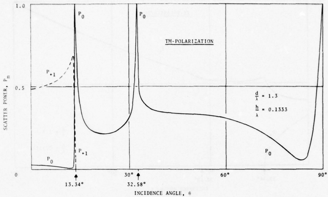
Fig. 5a. Powers P_m of propagating space harmonics vs. arrival angle \theta of incident wave (Profile 1; Spectral orders: m = +1, 0 ).
