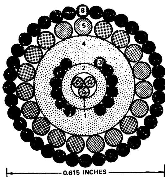
Figure 3. Simplex tow cable.
