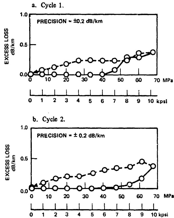
Figure 32. ITT cable pressure tests, graded index fiber.
