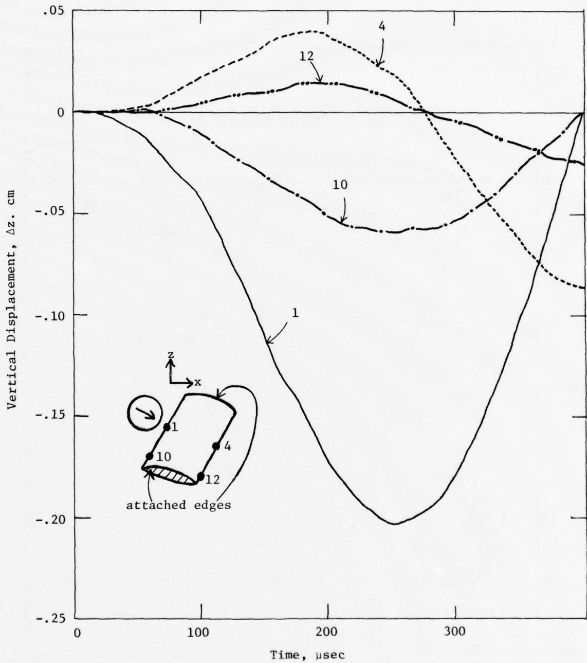
Figure 9. Vertical Displacement Histories of Selected Points on Stainless Steel (SS403) Turbine Blade Following 675 fps Impact of 85 gm Water Sphere at 25^\circ on Leading Edge (Case E)
