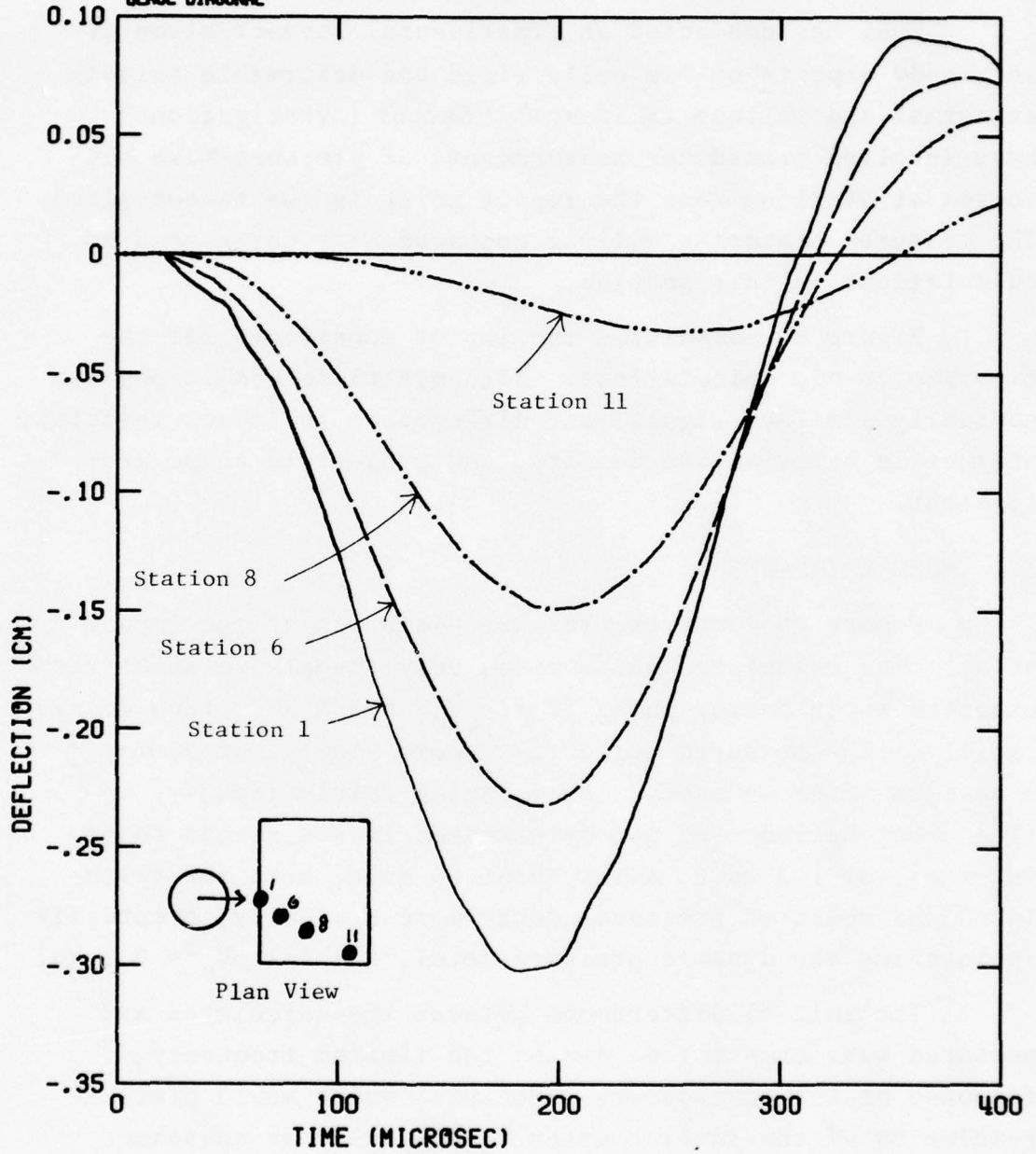
Figure 47. Vertical Displacement Histories at Selected Points on Surface of Bo-Al Turbine Blade Impacted on Leading Edge by 85-gm Water Sphere at 25° Obliquity (Case F)
