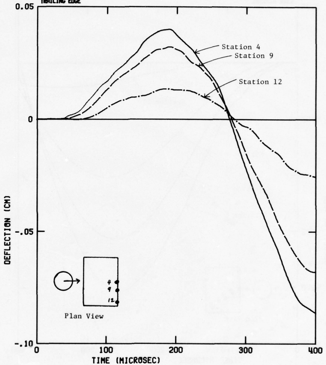
Figure 42. Vertical Displacement Histories at Selected Points Along Trailing Edge of Stainless Steel (SS403) Blade Impacted by 85-gm Water Sphere at 25° Obliquity (Case E)
