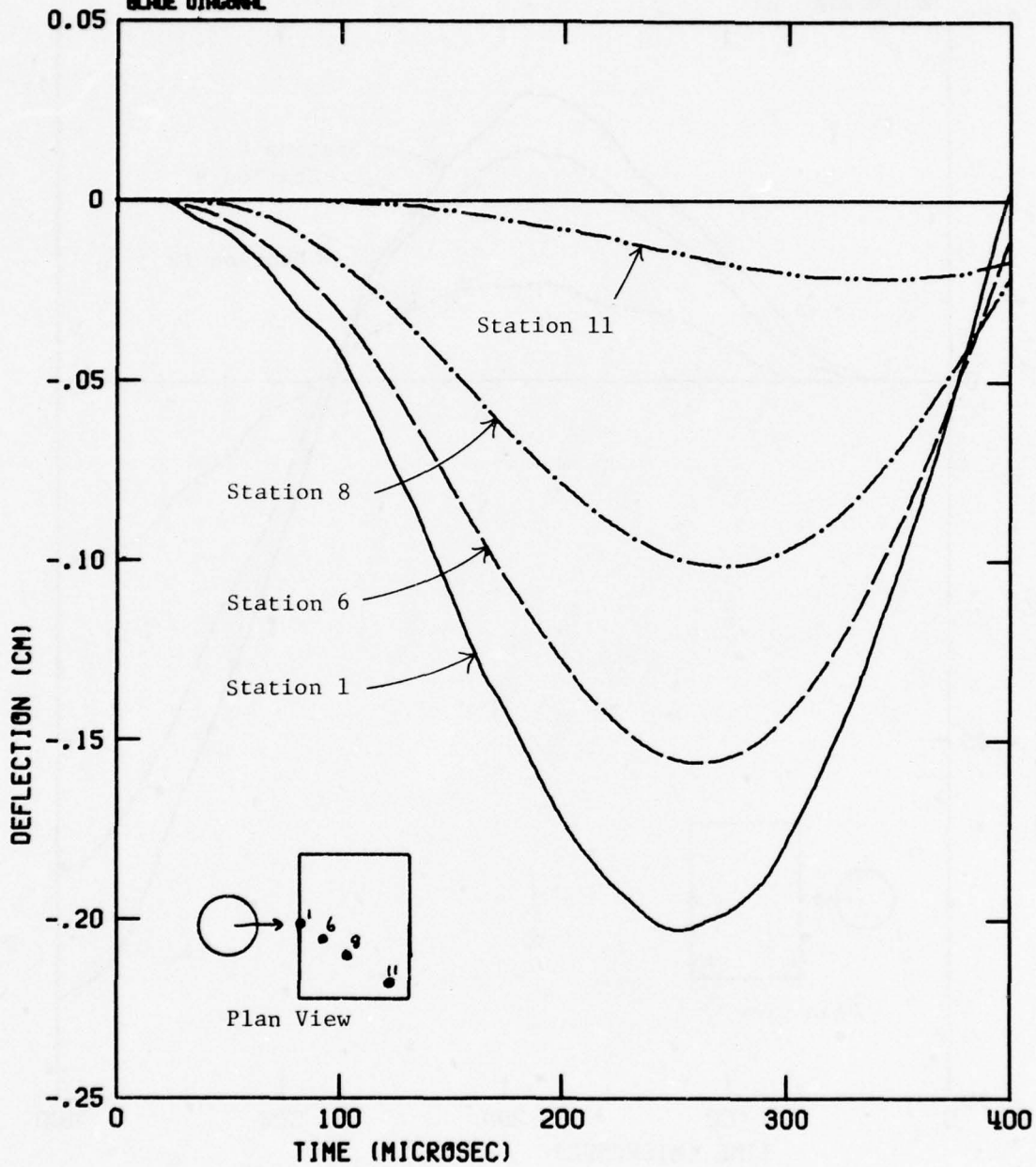
Figure 43. Vertical Displacement Histories at Selected Points on Surface of Stainless Steel (SS403) Blade After Impact of 85-gm Water Sphere at 25° Obliquity on Leading Edge (Case E)
