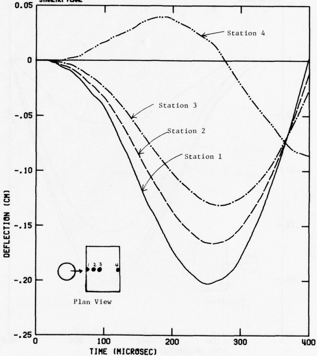
Figure 40. Vertical Displacement Histories at Selected Points Downstream of Impact of 85-gm Water Sphere at 25° Obliquity on Leading Edge of Stainless Steel (SS403) Blade (Case E)
