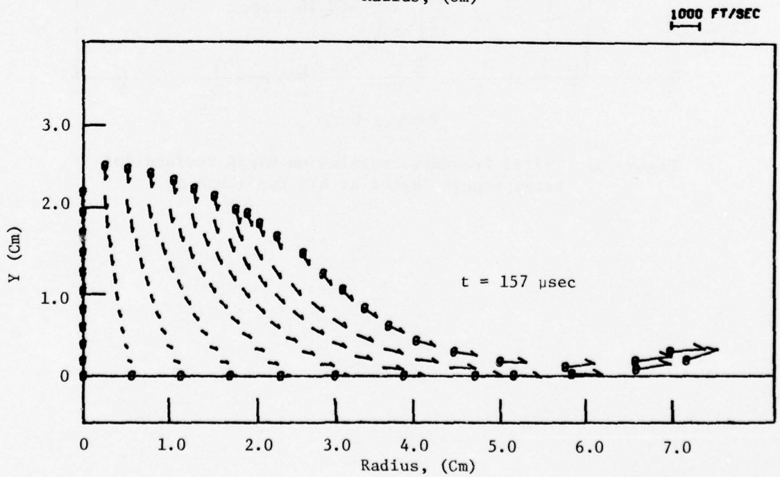
Figure 2. Velocity Field for a Water Sphere Impact at 675 fps onto a Rigid Surface (Case A) at 41 and 157 \mu\text{sec} .
