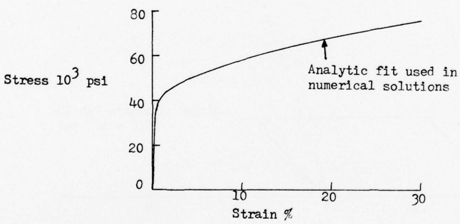
Figure A-2. SS403 simple tension stress-strain curve fit used in the numerical solutions showing the comparison with the base curve from Watter and Lincoln (Ref. 8) and the extrapolation to large strains
