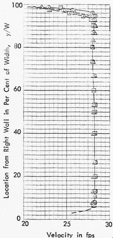
Horizontal Velocity Profiles at h/D = 0.5
