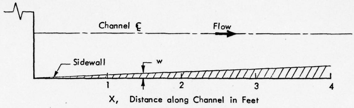
Plan View of Channel Surface
