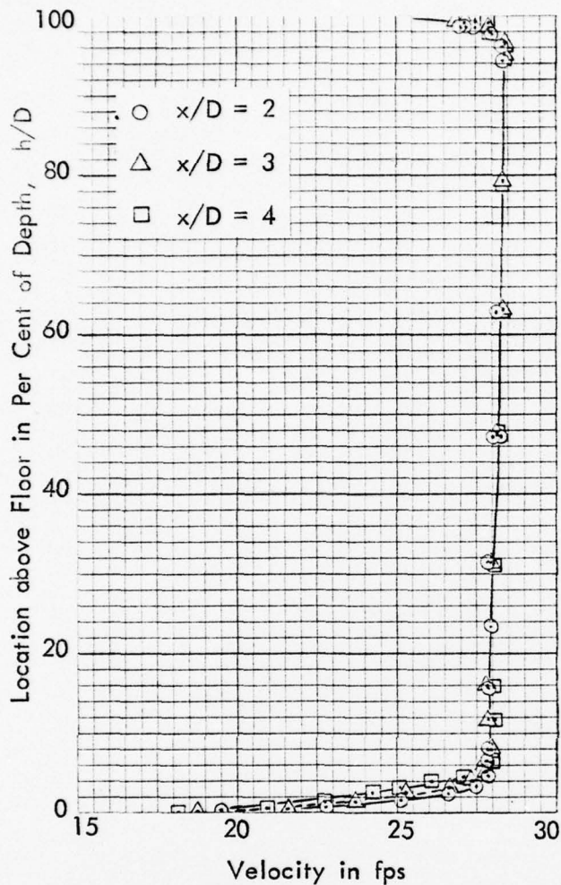
Vertical Velocity Profiles in Center Plane
