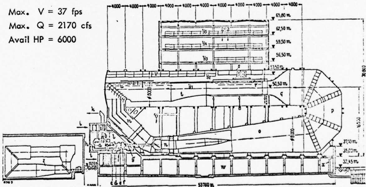
Fig. D-3 - The Variable-Pressure, Free Surface Test Facility of VWS in West Berlin with Horizontal Gravity Air Separator (from Ref. [D-9])
