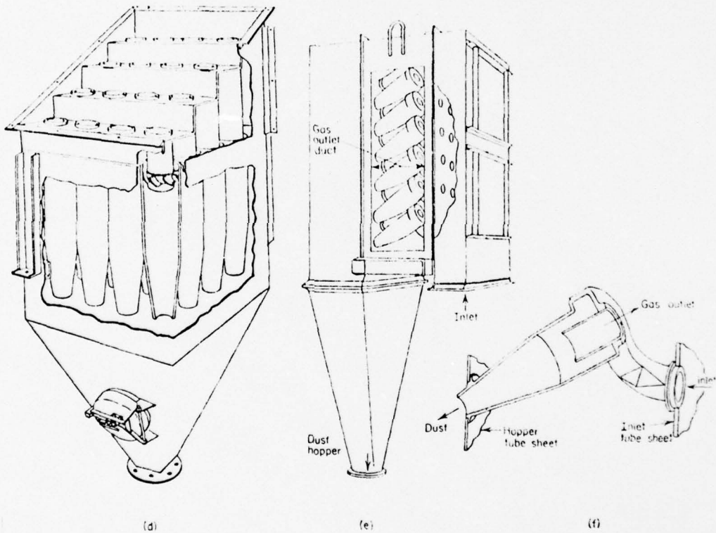
Typical commercial cyclones. (a) Duclone collector. ( Ducon Company .) (b) Sirocco type D collector. ( American Blower Co. ) (c) Van Tongeren cyclone. ( Bull Engineering Co. ) (d) Multiclone collector. ( Western Precipitation Corp. ) (e) Dustex miniature collector assembly. ( Dustex Corp. ) (f) Cutaway of the Dustex cyclone tube.
