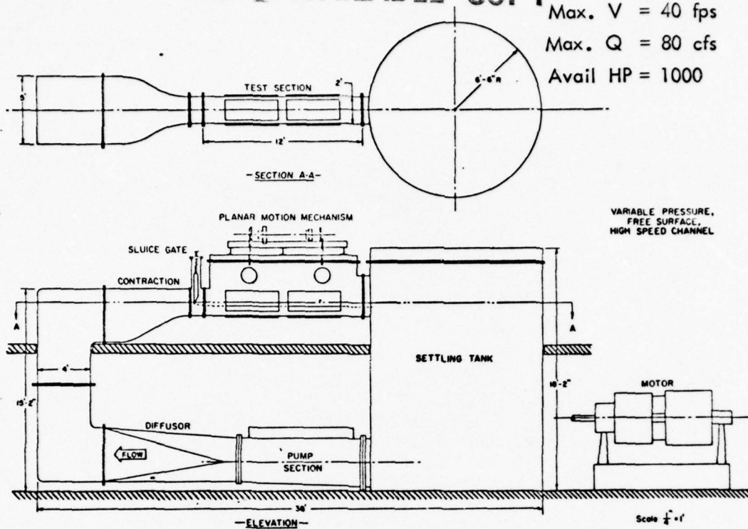
Fig. D-2 - The Hydronautics Variable-Pressure, Free Surface Test Facility with Vertical Gravity Air Separator (from Ref. [D-8])
