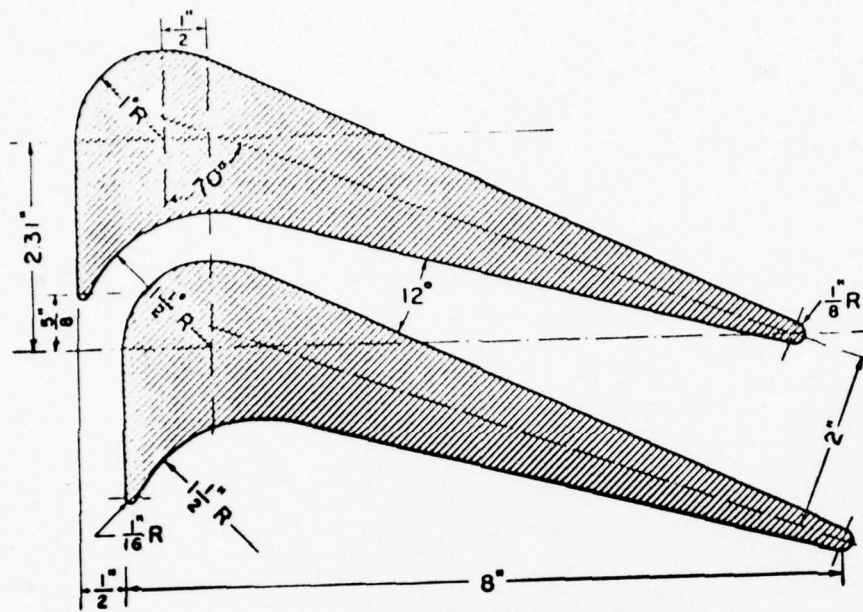
Vane Detail
