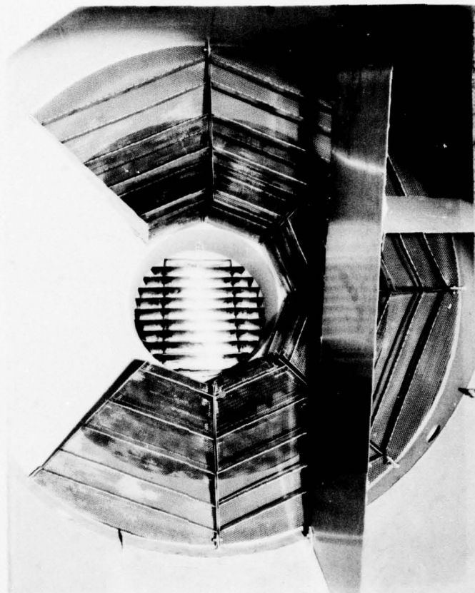
Fig. E-3 - Partial Assembly of the Resistance Members of the Separator Diffuser of the SAF 42-Inch Tunnel (view looking upstream with separator support plates shown in right foreground)
