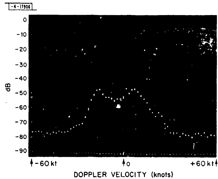
Fig. A-2. Precipitation spectrum at azimuth of 90°.
