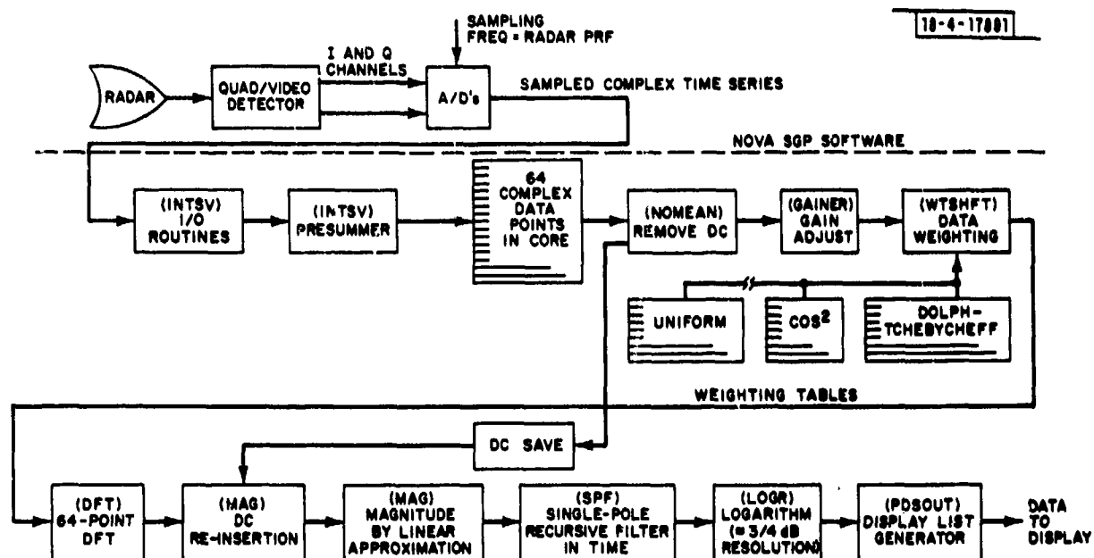
Fig. IV-14. SGP system block diagram.
