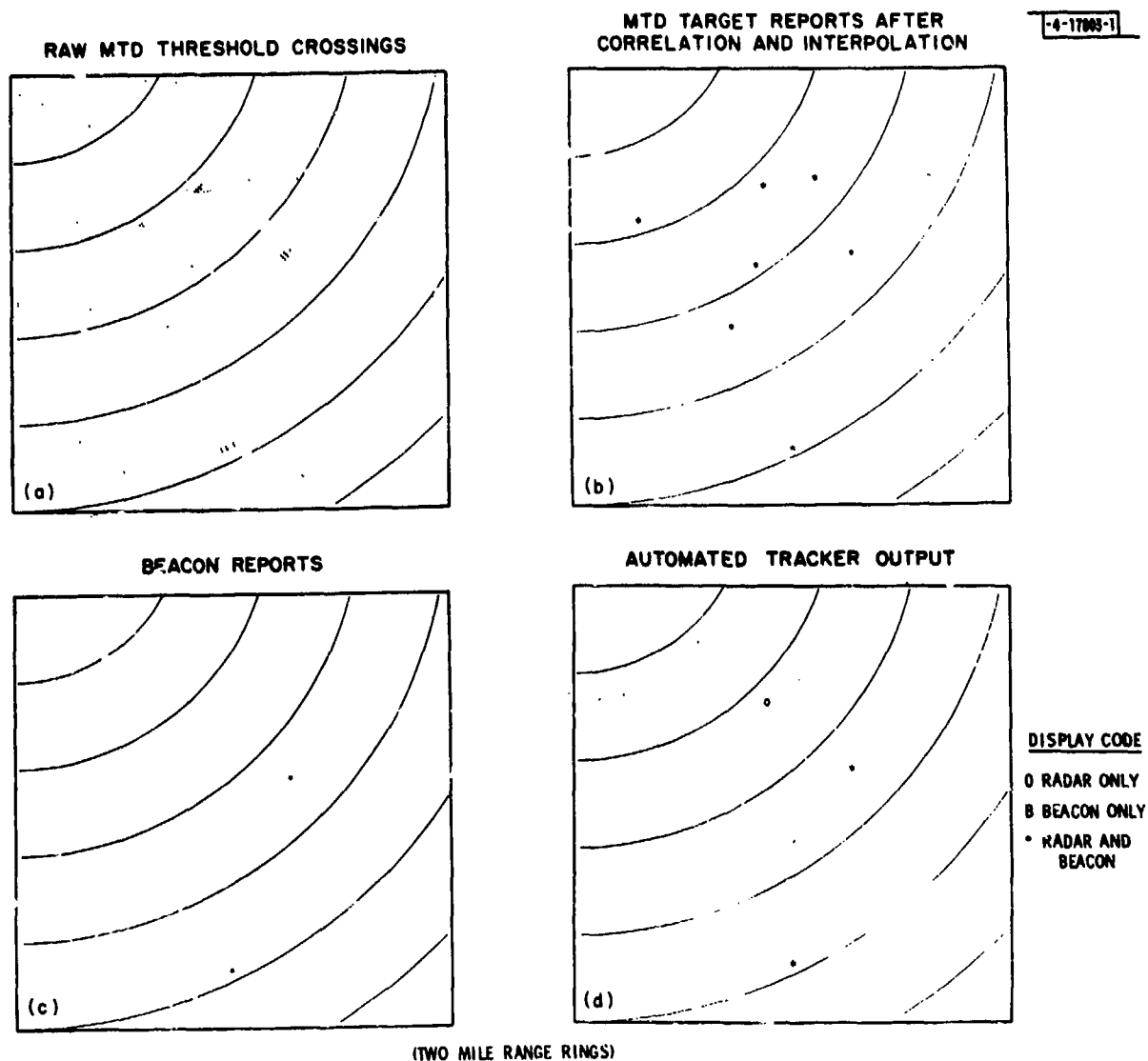
Fig. IV-16. Single scan displays of MTD data (O:radar only; B:beacon only; *:radar and beacon).
