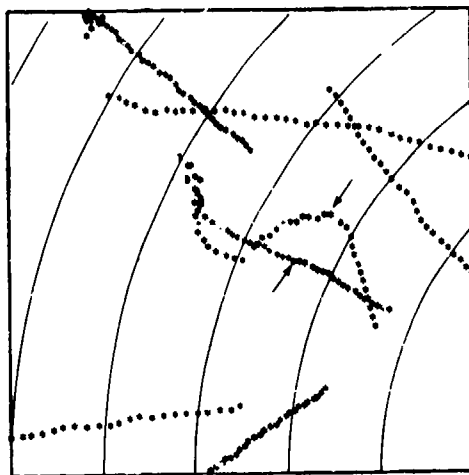
Fig. V-54. MTD automated tracker output - radar and beacon data (test flight of 2 September 1975).
