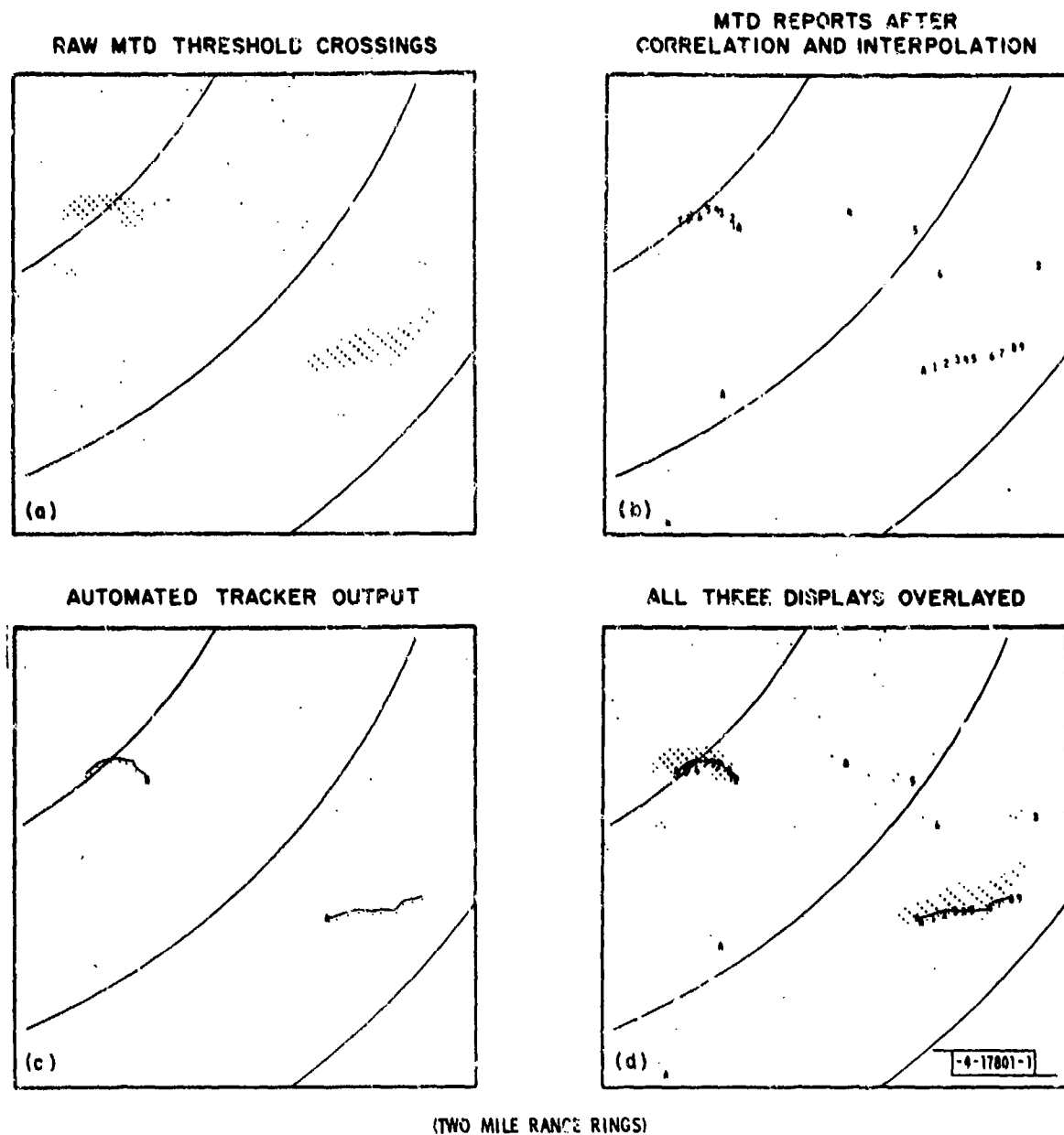
Fig. IV-21. Different types of MTD data displayed singularly and overlaid.
