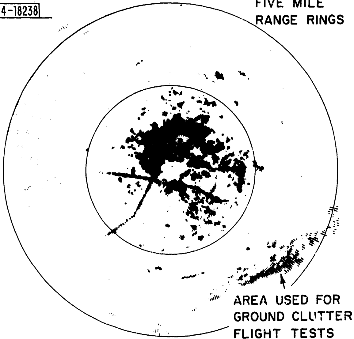
Fig. V-32. Digital map of ground clutter at NAFEC (5 nmi range rings).
