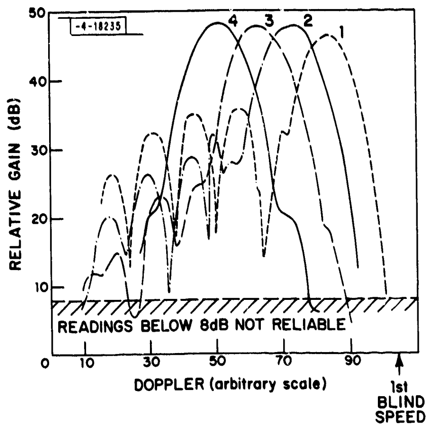
Fig. V-9. Doppler response of MTD weather thresholded channels (measured).
