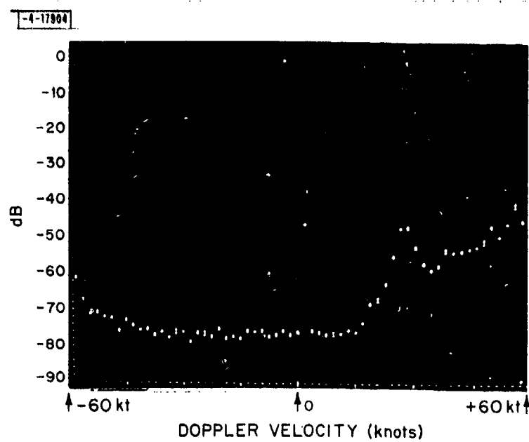
Fig. A-4. Precipitation spectrum at azimuth of 150°.
