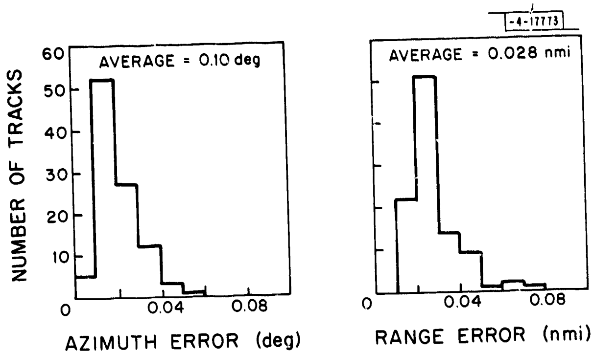
Fig. V-51. MTD/beacon track report accuracy (100 tracks).
