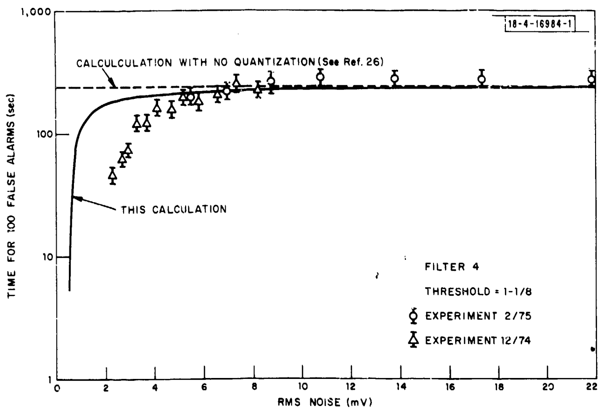
Fig. V-5. False alarm time vs. rms noise level.
