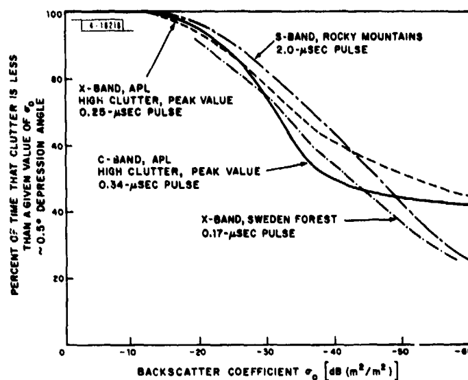
Fig. III-1. Land clutter backscatter distribution from surface radars (from Reference 4).
