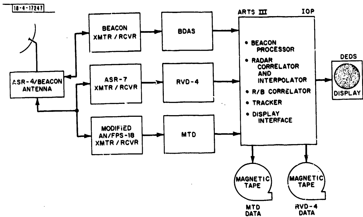
Fig. II-3. MTD/RVD-4 experimental test set-up.
