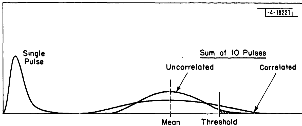
Fig. III-8. Noncoherent integration (probability distributions).
