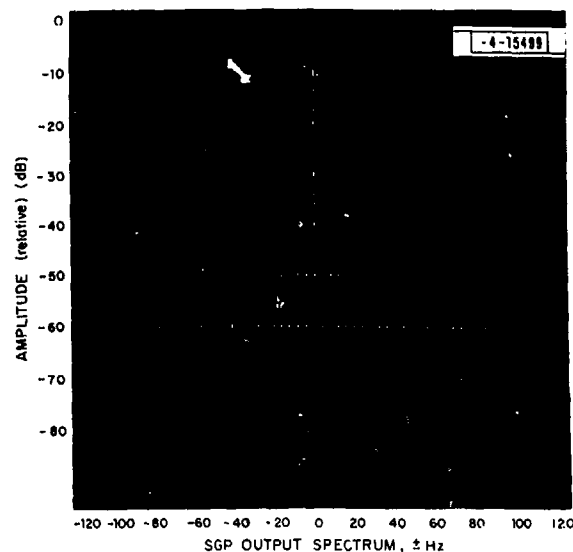
Fig. IV-13. Fixed target at 31 nmi. (Output of FPS-18 with SGP; horizontal scale to \pm 125 Hz.)
