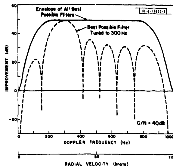
Fig. III-4. Improvement of target-to-interference ratio, scanning antenna.
