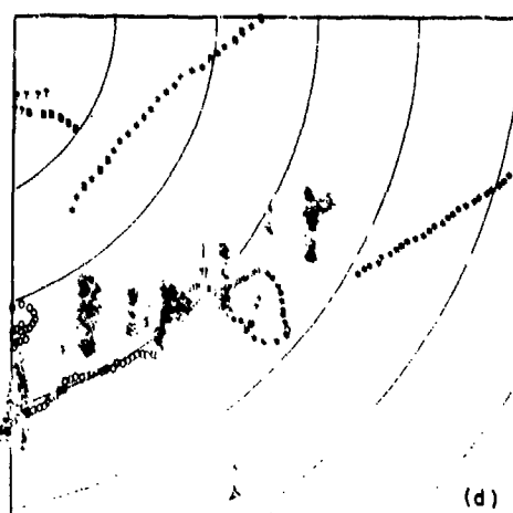
Fig. V-40. MTD-automated tracker output for ground clutter test flight (12 August 1975); altitude = 1000 ft.
