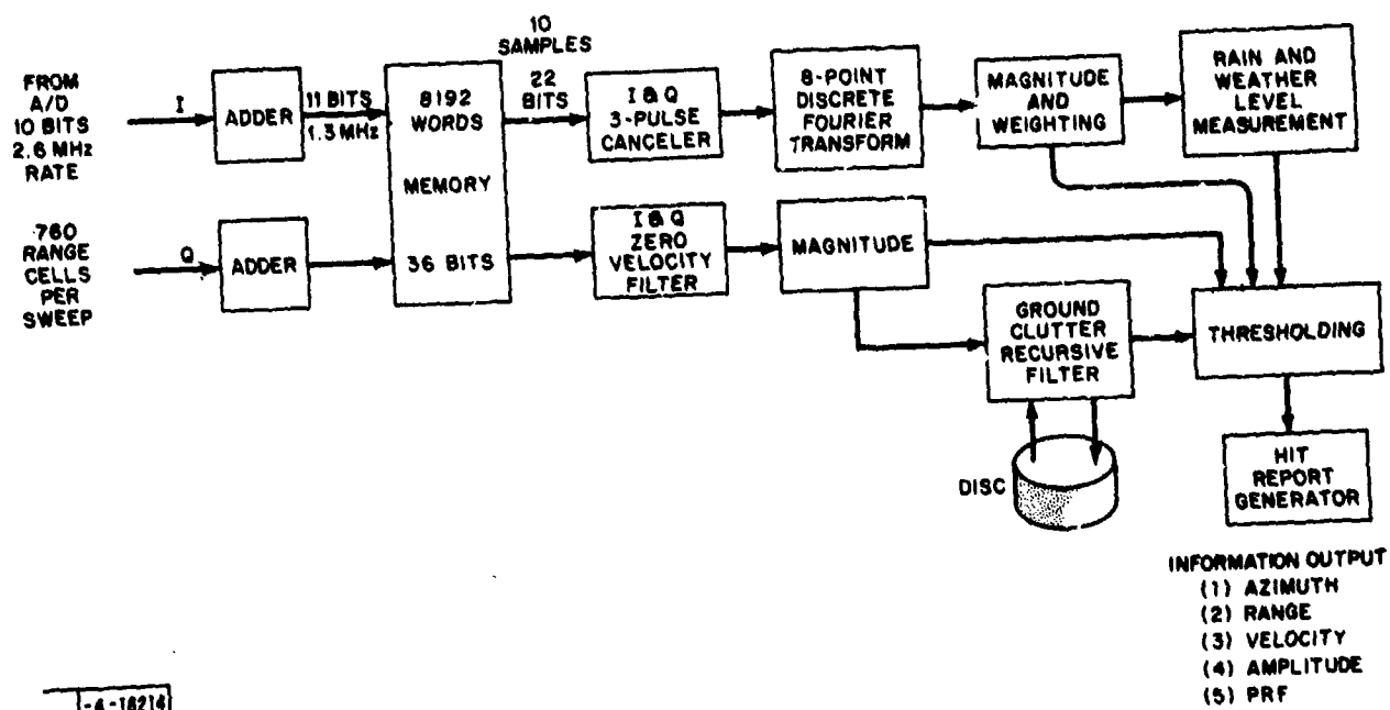
Fig. II-2. MTD processor block diagram.
