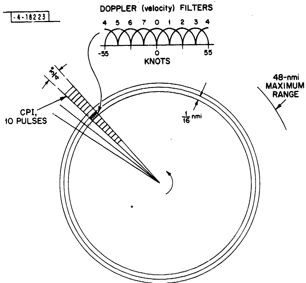
Fig. III-10. MTD resolution.
