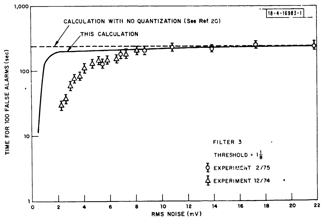
Fig. V-4. False alarm time vs. rms noise level.
