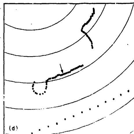
Fig. V-37. MTD-automated tracker output for ground clutter test flight (12 August 1975); altitude = 1000 ft.
