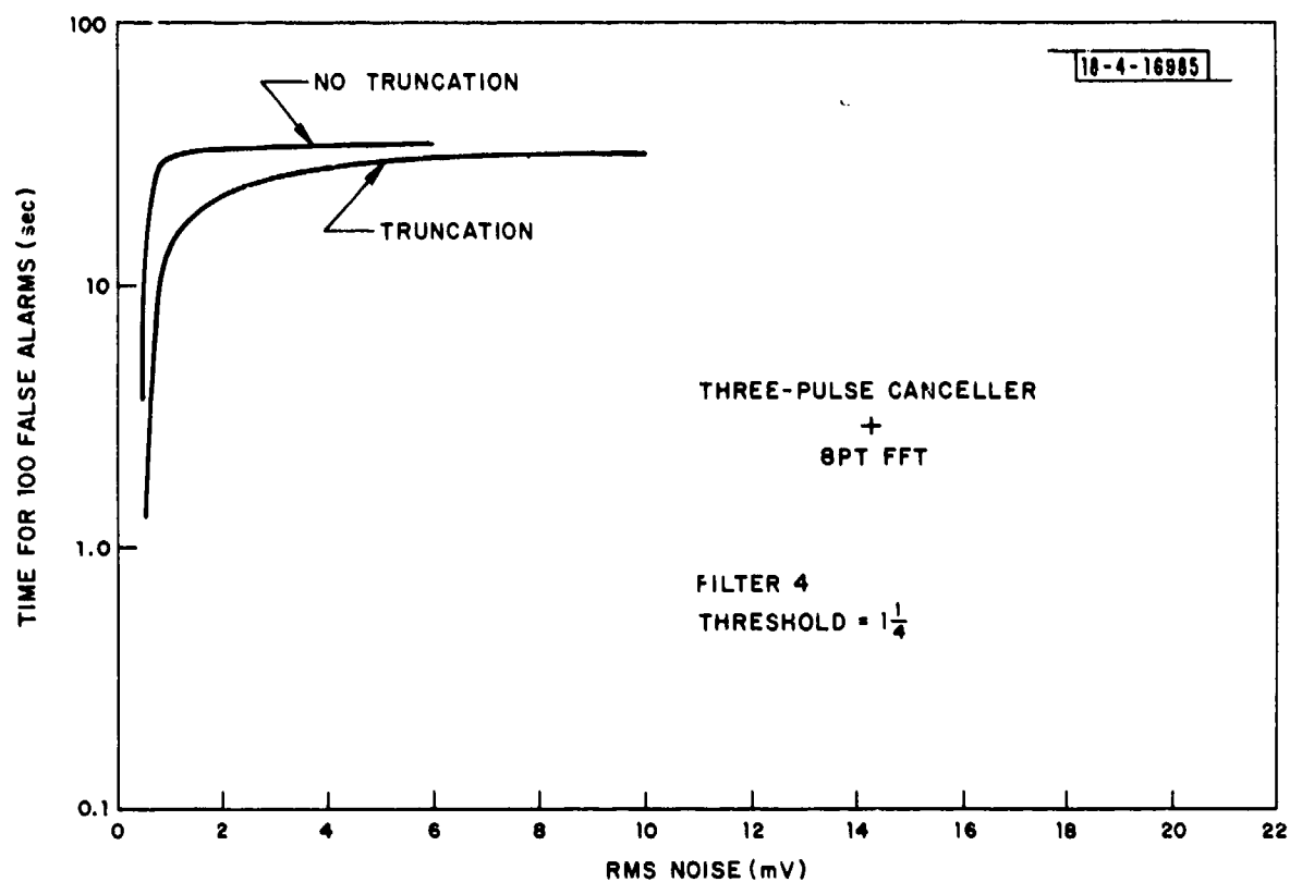
Fig. C-6. False alarm time vs. rms noise voltage: filter 4, threshold = 1\frac{1}{4} .
