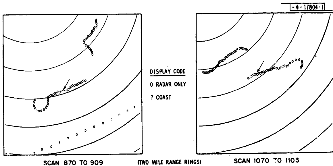
Fig. V-46. MTD-automated tracker output - radar only data (test flight of 12 August 1975).
