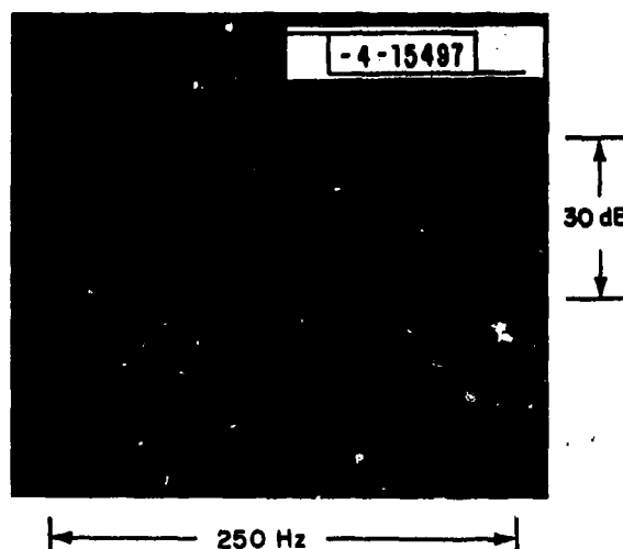
Fig. IV-11. Fixed target at 35 nm. (Output of FPS-18 with SGP; note balanced sidebands at \pm 30 Hz,)
