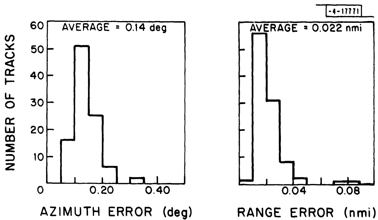
Fig. V-49. MTD report accuracy (100 tracks).
