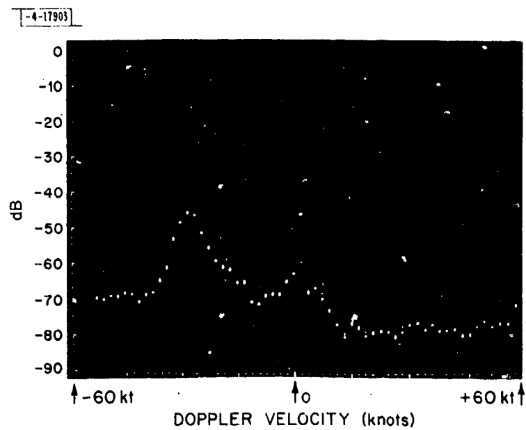
Fig. A-5. Precipitation spectrum at azimuth of 300°.
