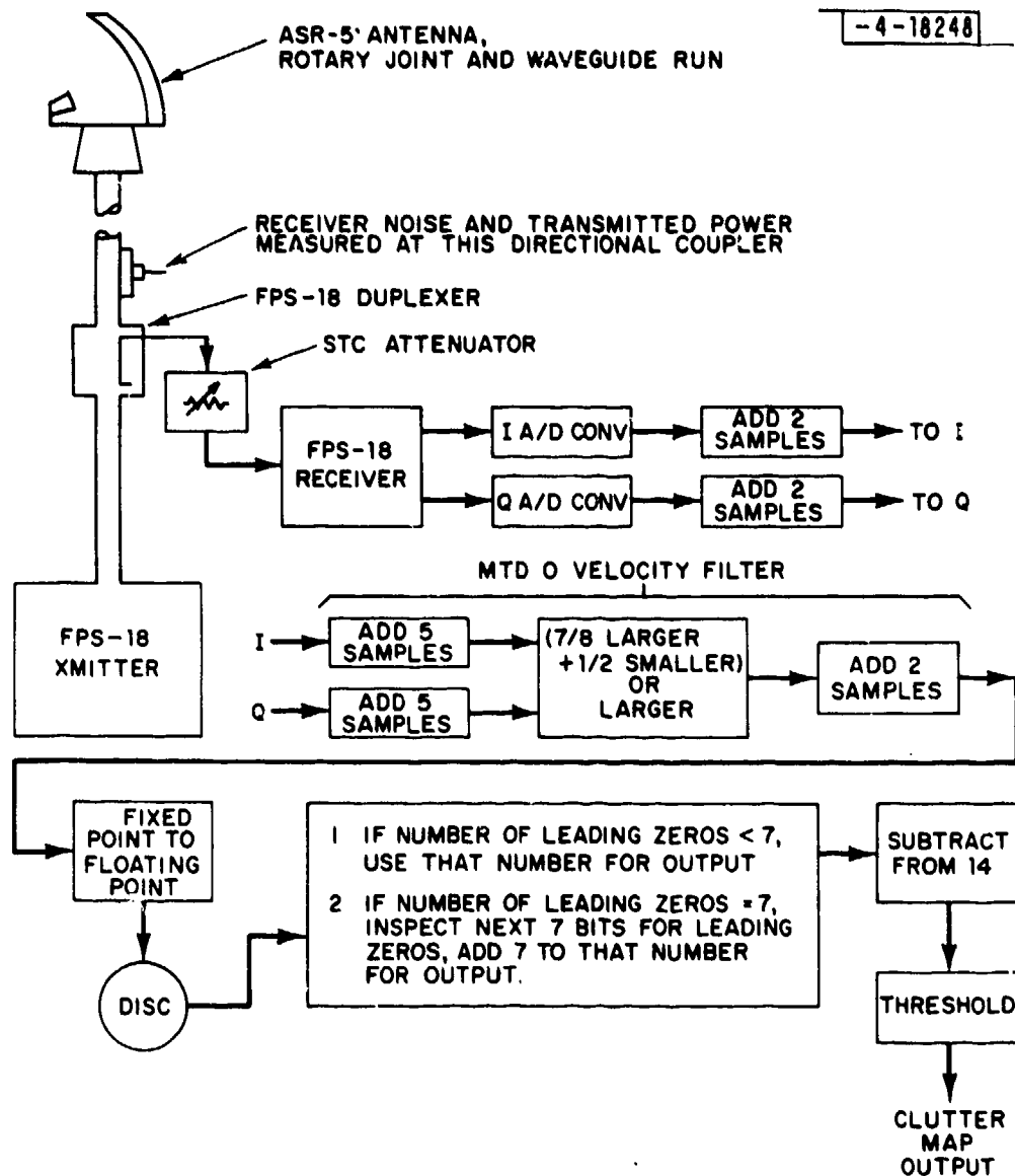
Fig. B-1. Clutter map measurement system.
