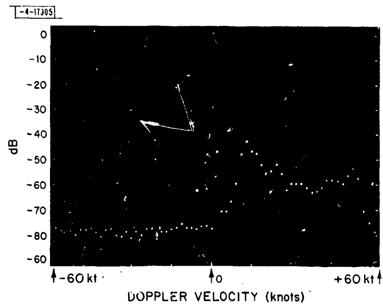
Fig. A-3. Precipitation spectrum at azimuth of 130°.
