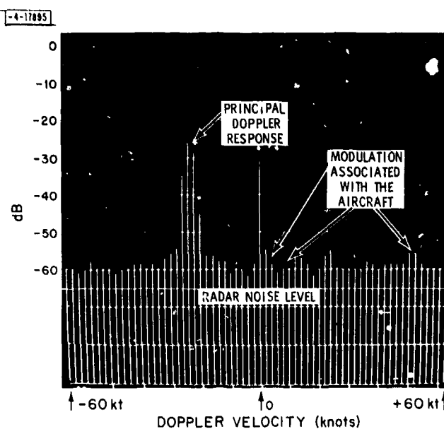
Fig. A-11. Airliner approaching radar at traffic pattern speed.
