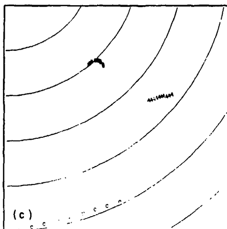
Fig. 1V-19. Multiple scan displays of automated tracker output (radar only data).
