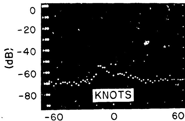
Fig. A-9. SGP doppler spectra of angels (probably multiple soaring seagulls).
