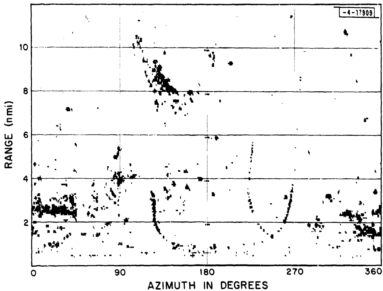
Fig. B-5. Range vs. azimuth plot of \sigma at NAFEC site.
