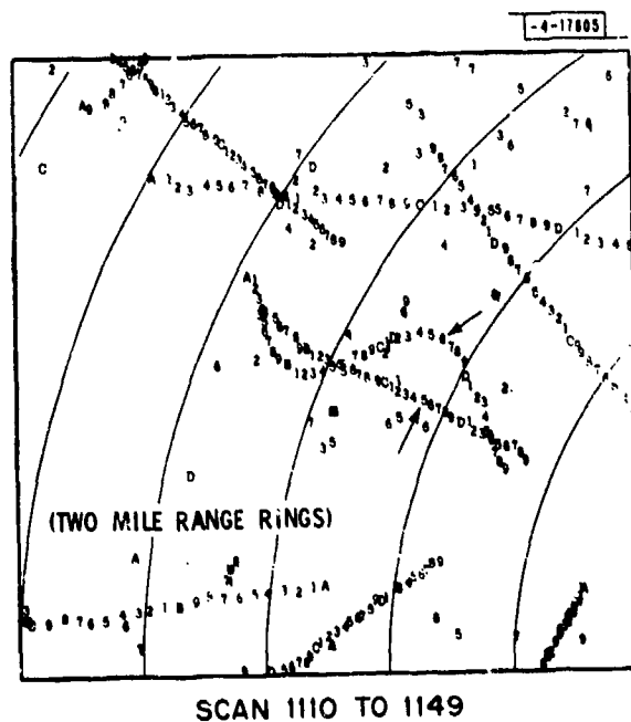
Fig. V-53. MTD report data (40 scans) (tests of 2 September 1975).
