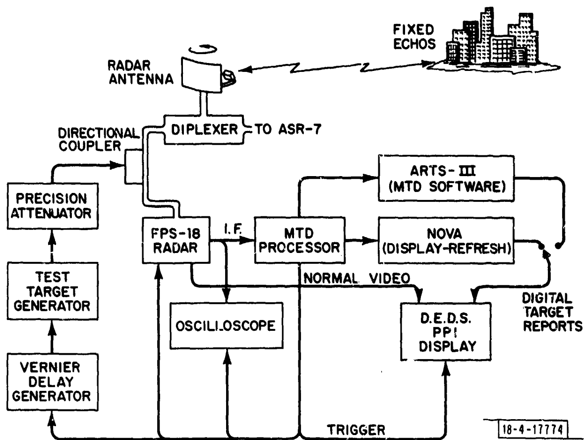
Fig. V-33. SCV test set-up.
