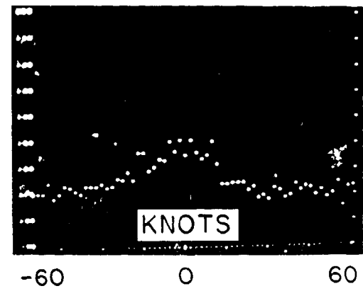
Fig. A-9. SGP doppler spectra of angels (probably multiple soaring seagulls).
