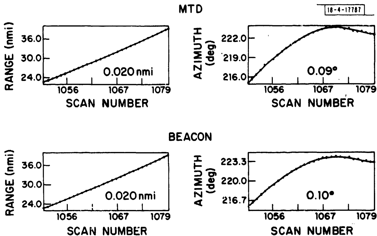
Fig. V-48. Range and azimuth vs. scan number (measured and fitted); for MTD and beacon data.
