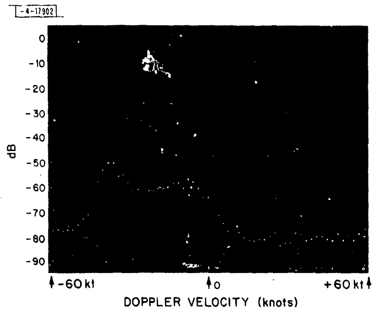
Fig. A-6. Precipitation spectrum at azimuth of 320°.
