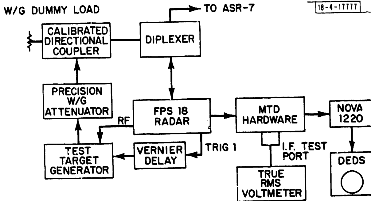
Fig. V-8. MTD sensitivity test set-up.
