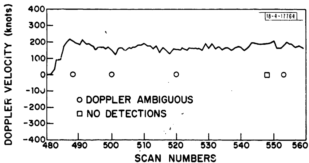
Fig. V-62. Doppler velocity of EB-57 (jet), measured.
