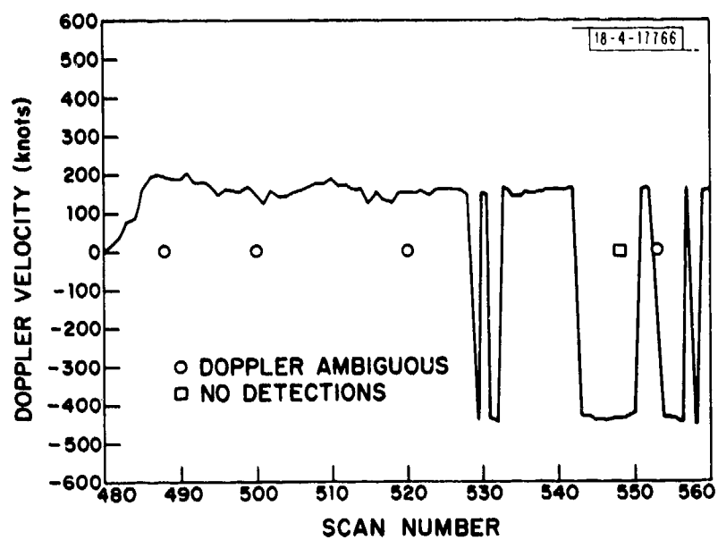
Fig. V-61. Doppler velocity of EB-57 (jet), measured using Univac algorithm.
