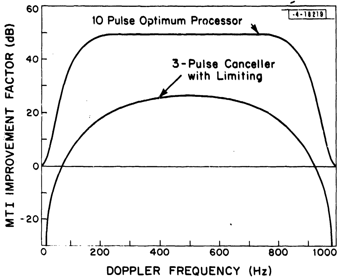
Fig. III-5. Comparison of optimum processor with conventional 3-pulse canceller.
