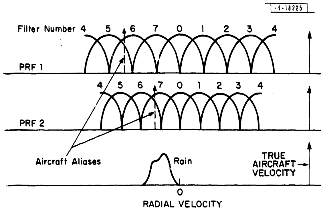
Fig. III-12. Detection in rain using two PRF's. (Schematic diagram of multiple PRF response to rain and aircraft. The doppler foldover occurs whenever the sampling rate is too low).
