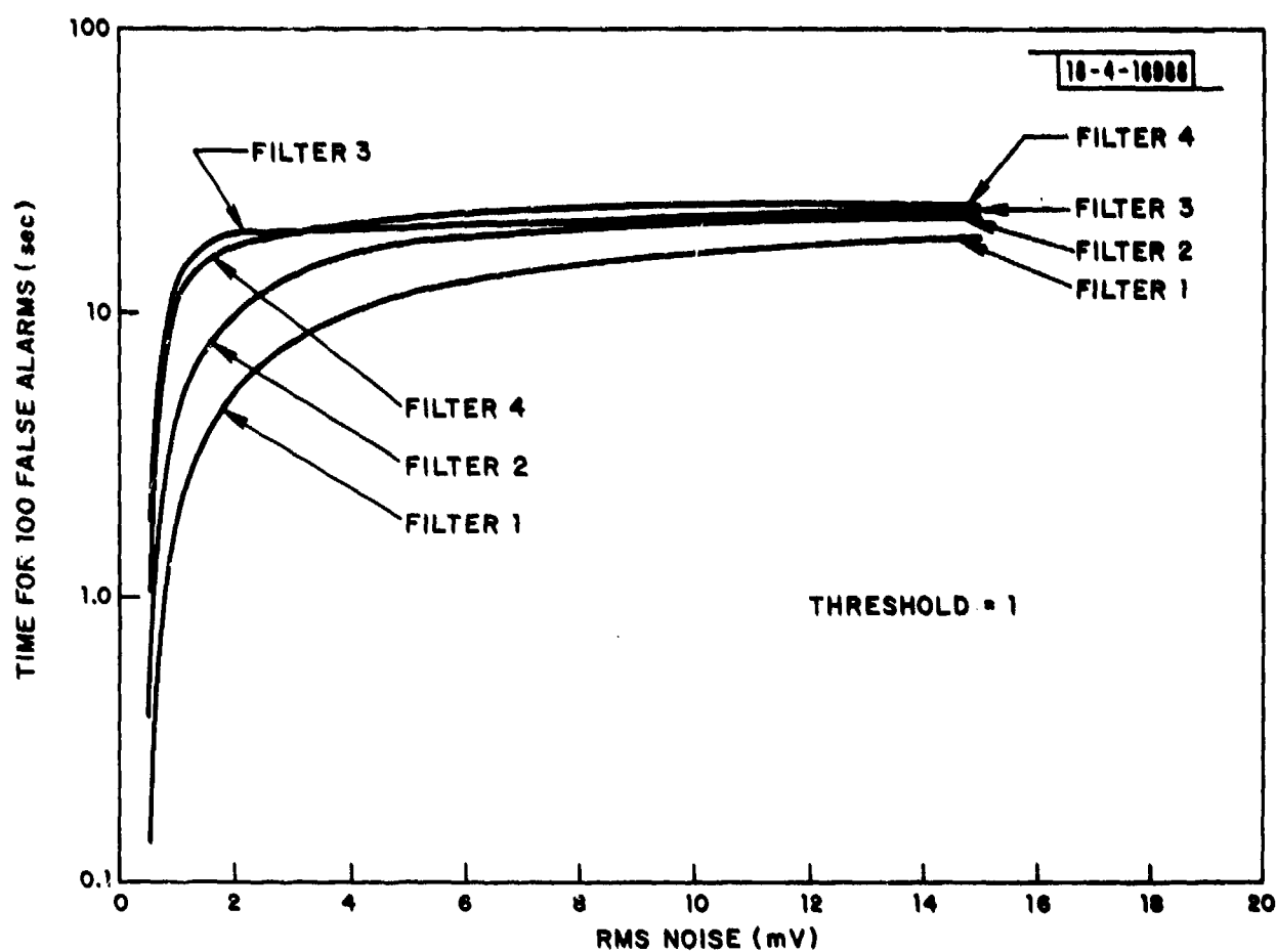
Fig. C-2. False alarm time vs. rms noise voltage: threshold = 1.
