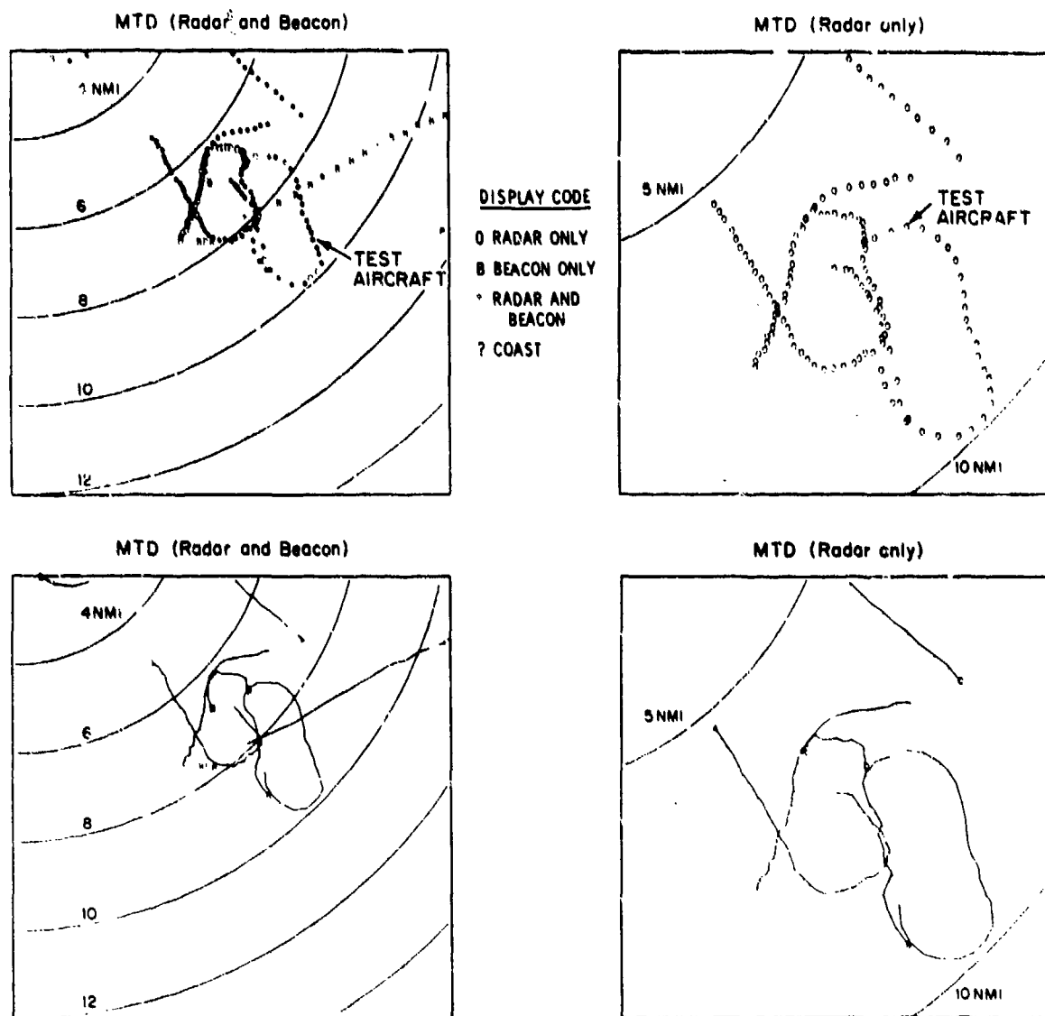
Fig. II-7. MTD subclutter performance: radar/beacon tracking and radar only compared.
