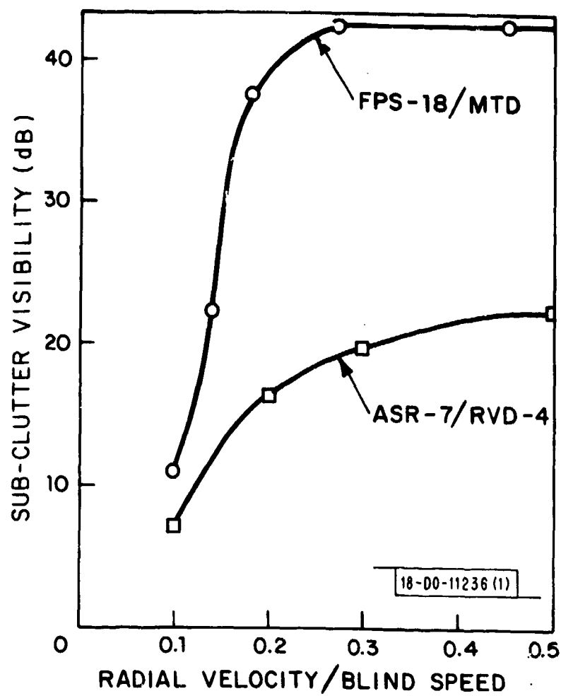
Fig. V-34. Subclutter visibility for P_D = 0.5 (measured).
