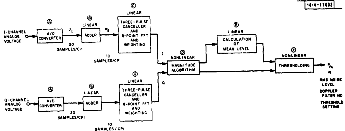
Fig. V-1. MTD processor: functional diagram.
