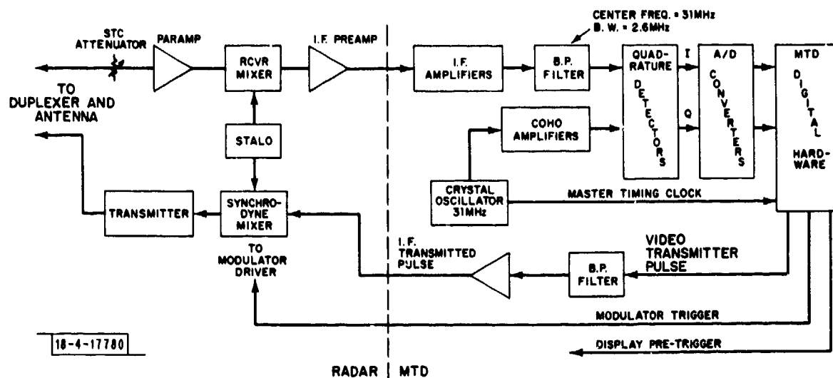
Fig. V-56. MTD interface with synchrondyne radars.
