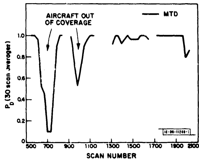
Fig. V-17. Blip/scan ratio during rain (6 August 1975).
