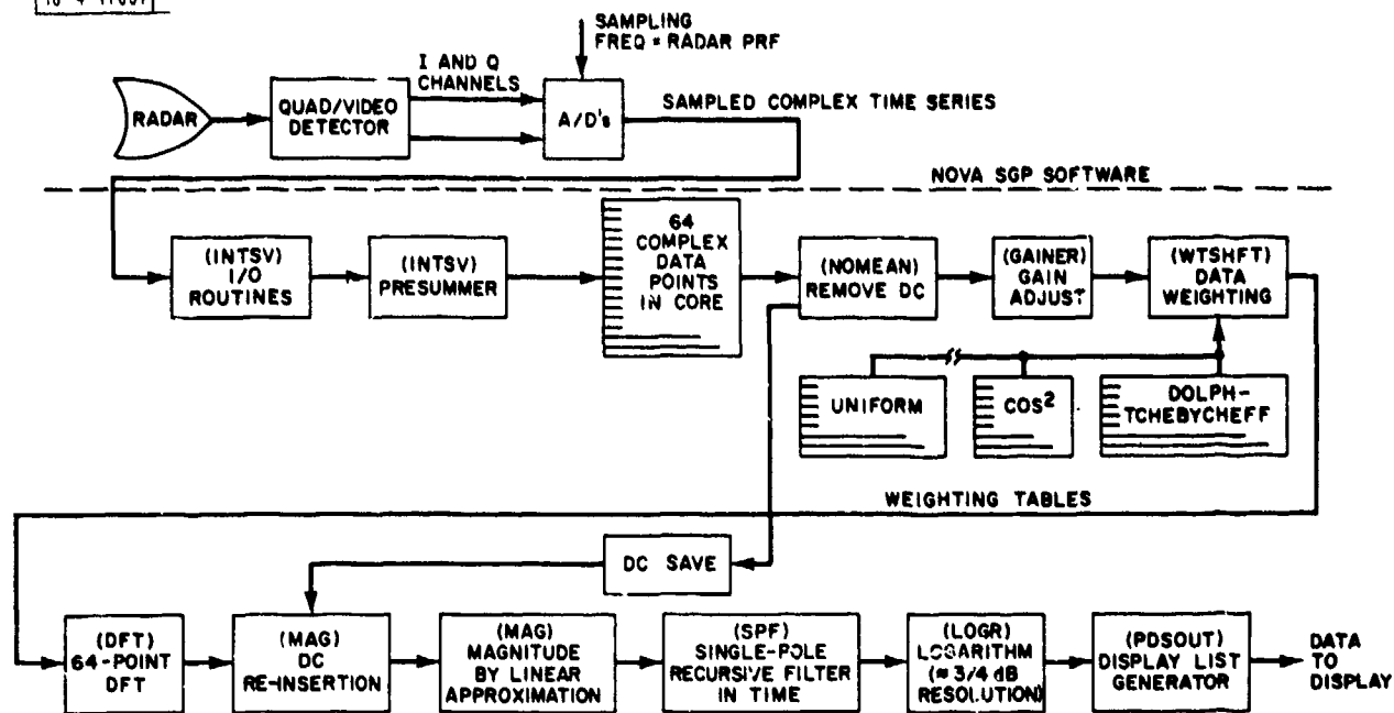
Fig. A-1. SGP system block diagram.
