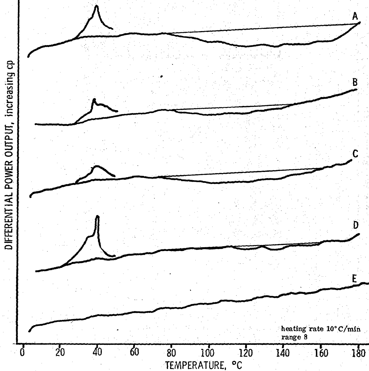
Figure 38. First DSC scans of epoxy emulsion films cured for 50 days at room temperature: A. Epon 1001-Versamid 115 combination; B. Epon 1001-Versamid 115-heated-to-55°C combination; C. (Epon 1001-bisphenol A)-Versamid 115 combination; D. Epon 1001-(Versamid 115-Dion DPM-3-800-LC) combination; E. solvent-cast Epon 1001-Versamid 115 combination.
