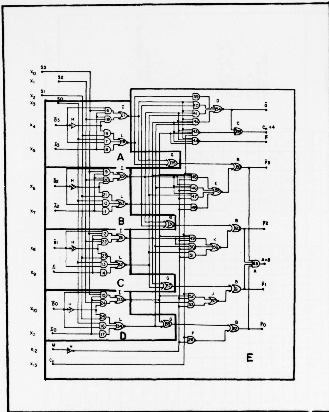
FIGURE 2. Partitioned Circuit SN 54181
