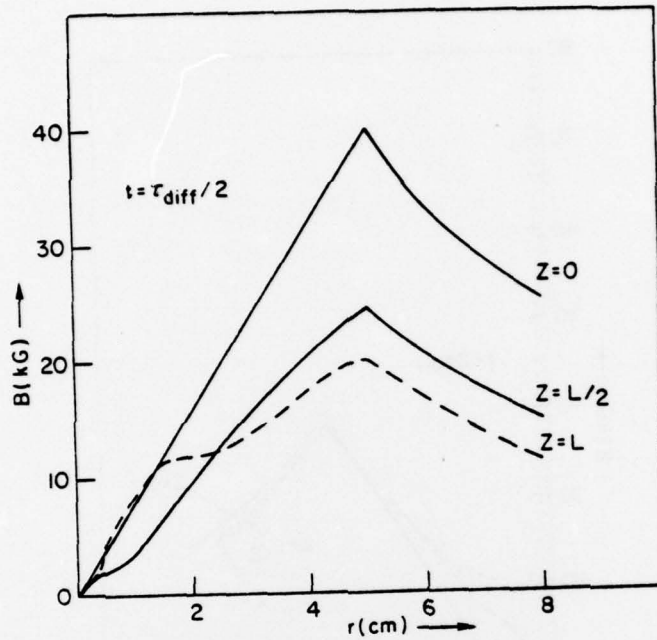
Fig. 6 — Magnetic field radial profiles at t = \tau_{diff}/2 at various z
