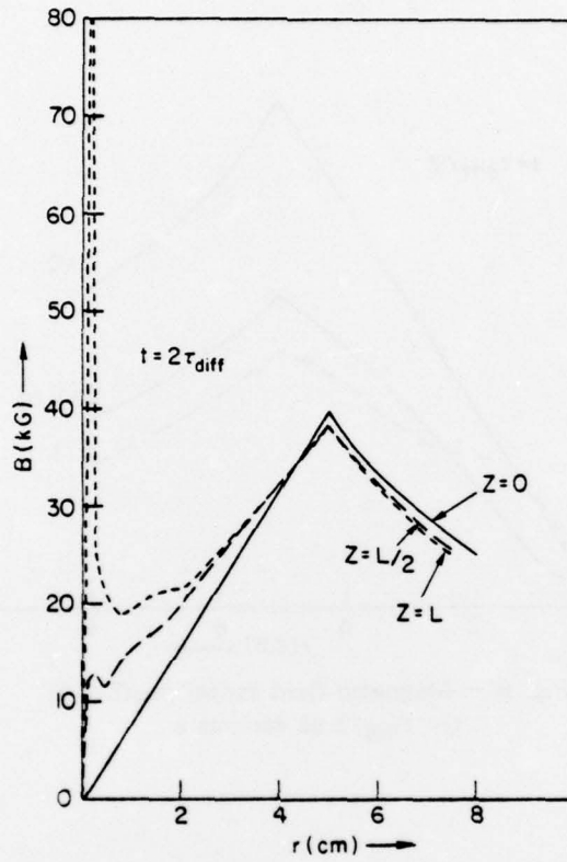
Fig. 7 - Magnetic field radial profiles at t = 2 \tau_{diff} at various z . Note that at z = 0 , the B field radial profile does not change. Also, large values of field near axis indicate pinching.
