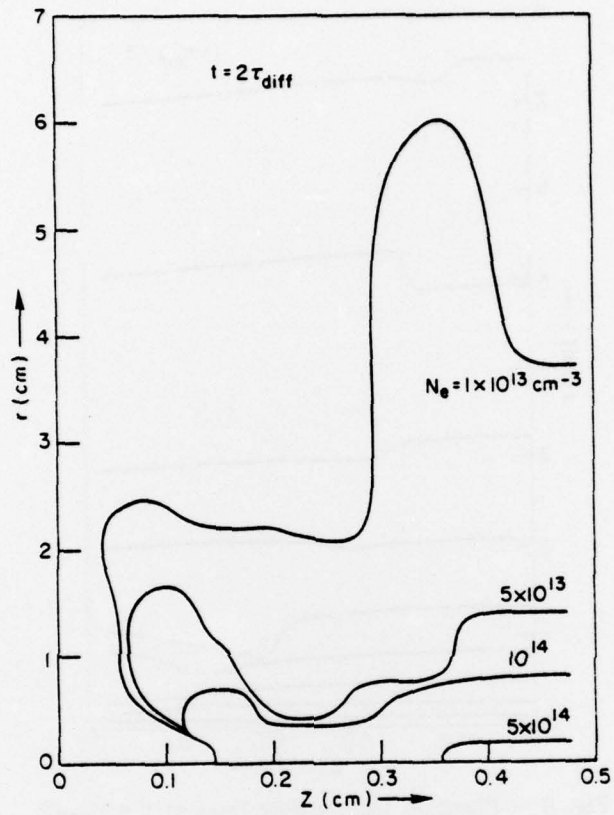
Fig. 2 — Electron density contours at t = 2 \tau_{diff}
