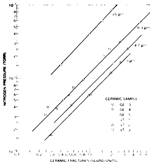
Figure 19. Nitrogen burst of trapped gas in ceramic voids.
