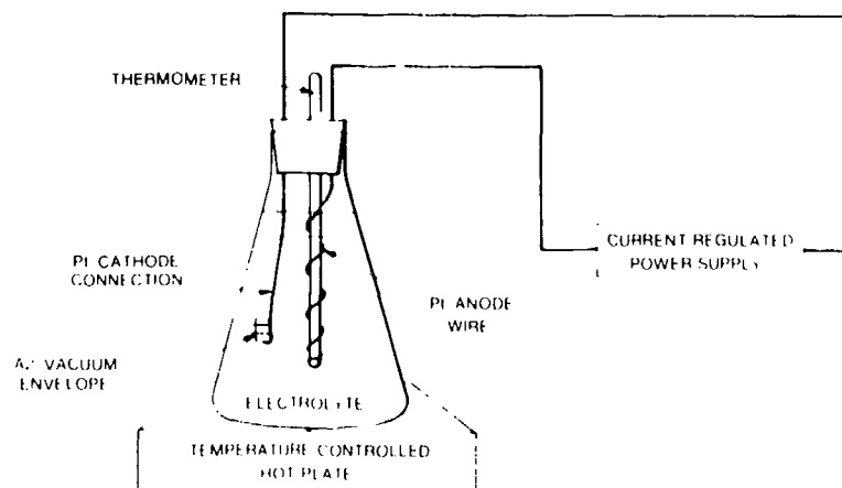
Figure 11. Electrolysis apparatus.
