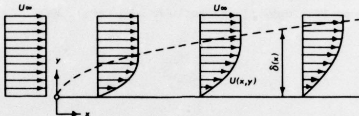
Figure 10. Theoretical boundary layer development
