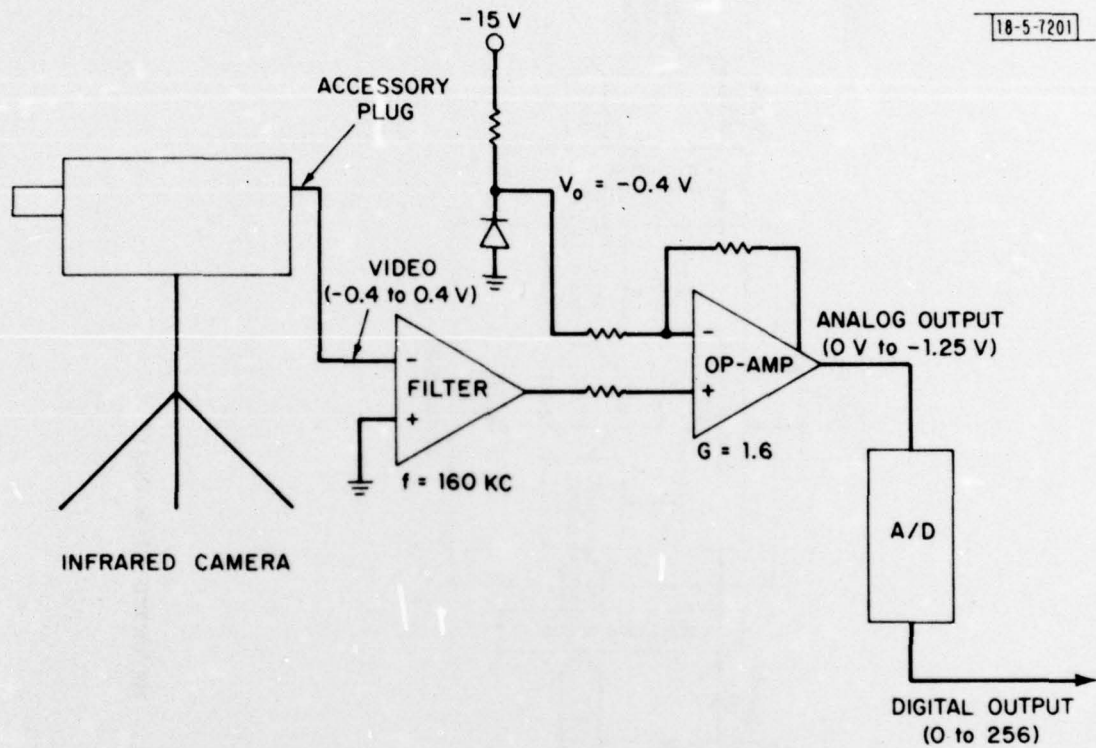
Fig. 3-2. Offset and gain circuit.
