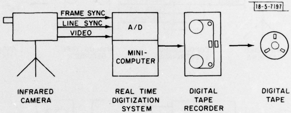
Fig. 1-1c. Direct digital recording method.
