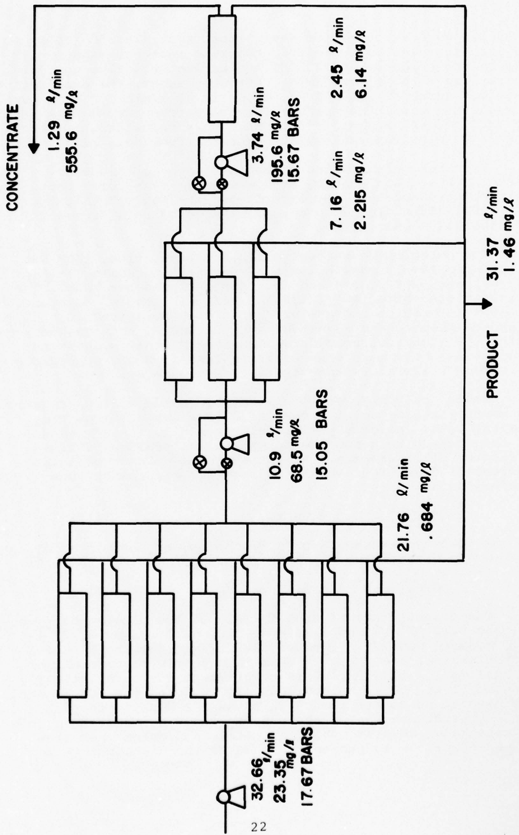
Figure 9. Reverse Osmosis Pilot Plant Designed for Starting Conditions
