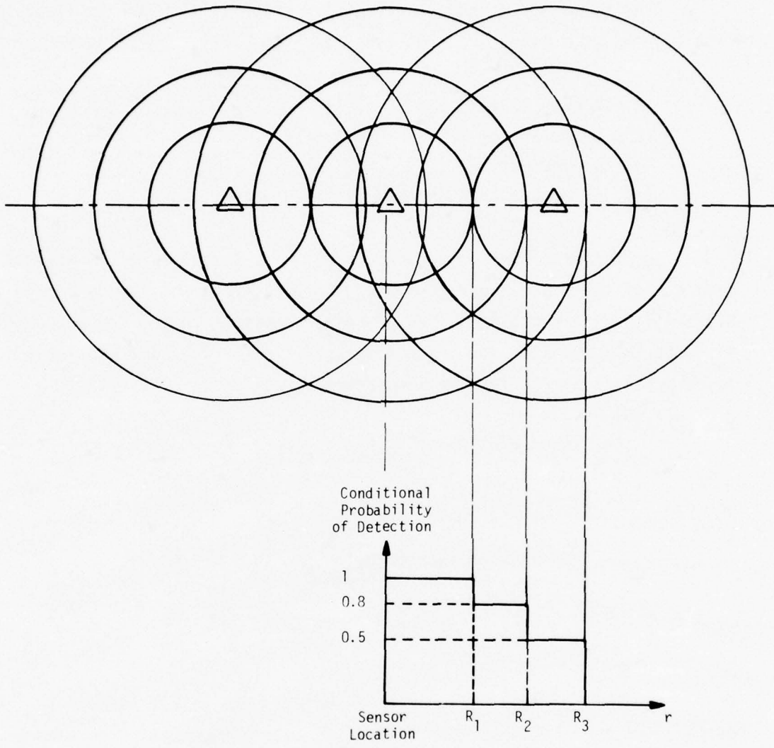
FIGURE 4-11. CONTOURS OF CONDITIONAL PROBABILITY OF SUBMARINE DETECTION AROUND A SENSOR PATTERN
