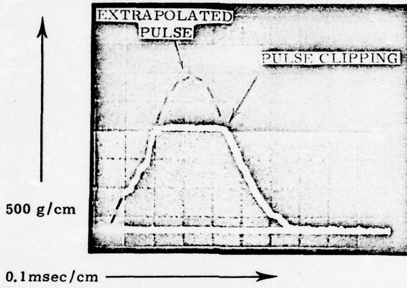
HALF SINE 2500g PULSE WIDTH 0.6msec
