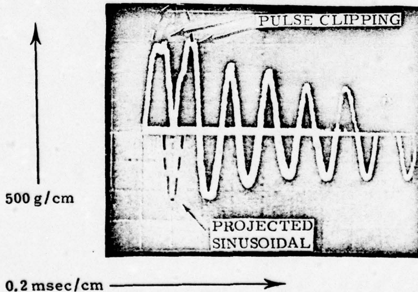
DECAYING SINUSOIDAL ACCELERATION OF T-7 WIRE SPOOL SUPERIM- POSED ON IMPACT PULSE
