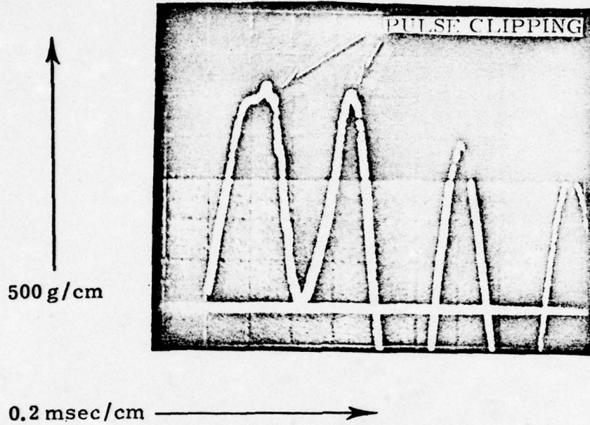
IMPACT PULSE CLIPPED AT 1,600 g DECAYING SINUSOIDAL ACCELERATION OF T-7 WIRE SPOOL
