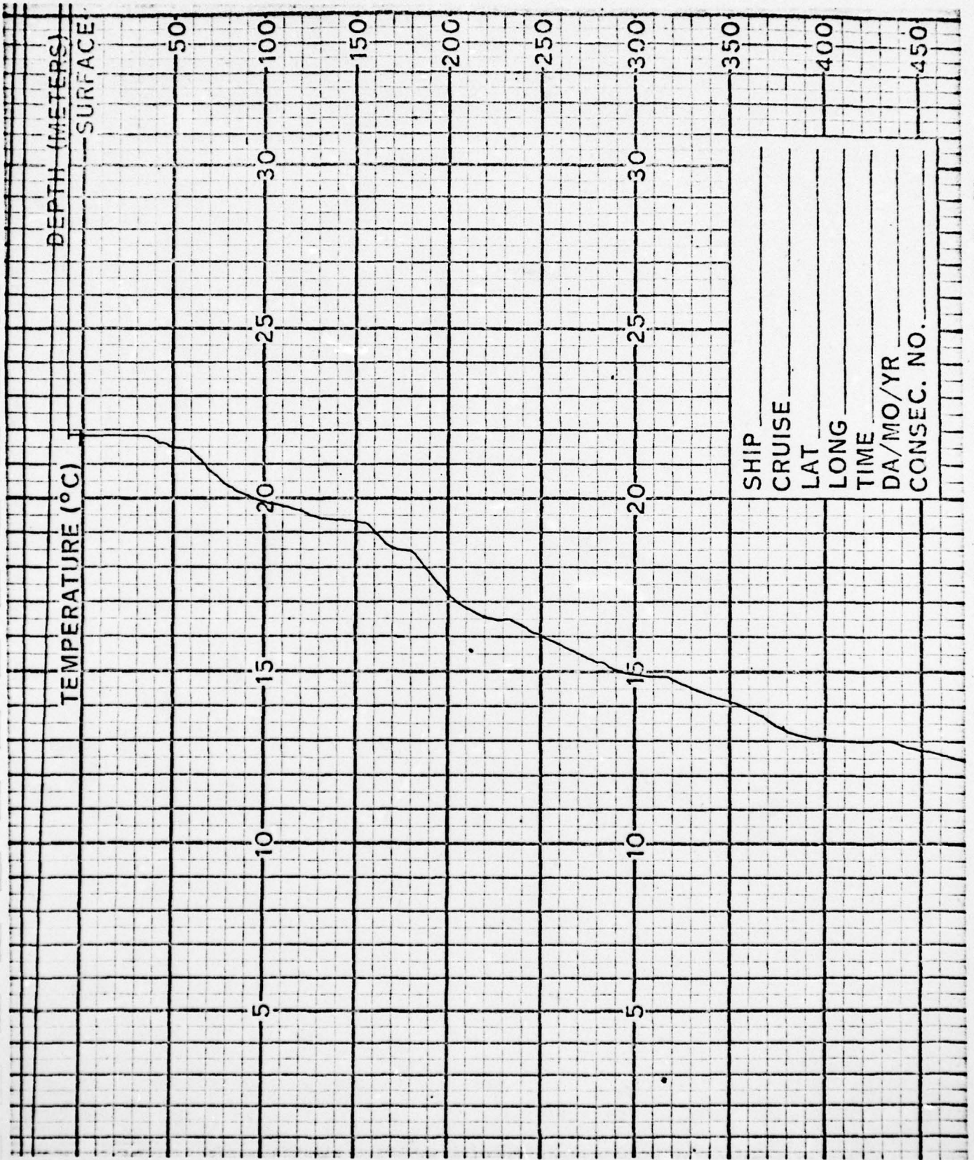
Figure 5-10 Sippican AXBT, P-3C Mockup Recorder Temperature Profile
