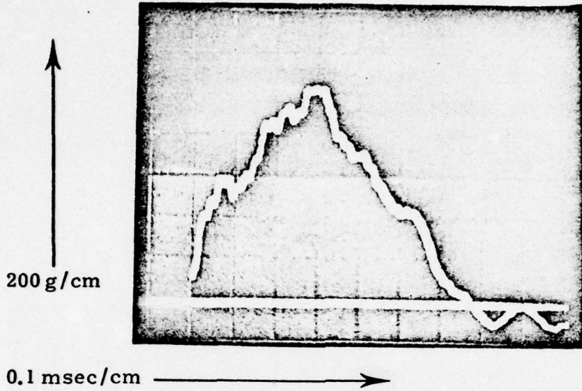
APPROXIMATE HALF SINE 1,000 g PULSE WIDTH 0.7 msec
