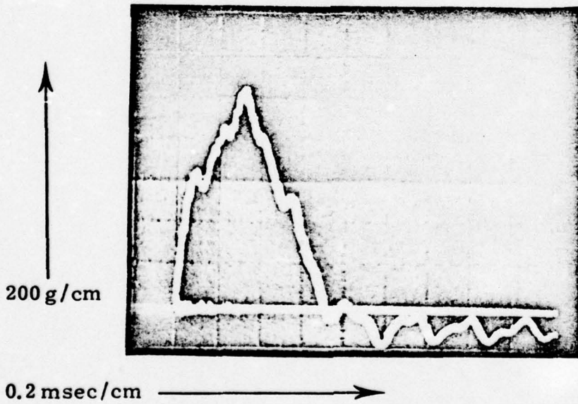
APPROXIMATE HALF SINE 1,000 g PULSE WIDTH 0.7 msec
