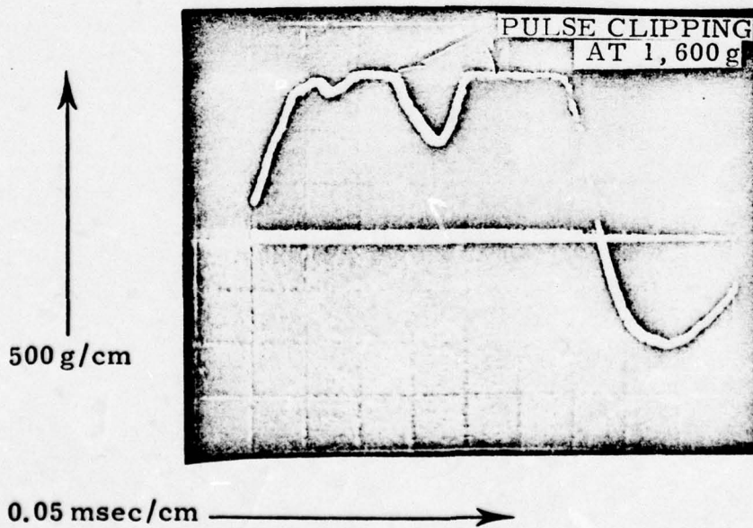
IMPACT PULSE INTERRUPTED BY DECAYING SINUSOIDAL ACCELERA- TION OF T-7 WIRE SPOOL
