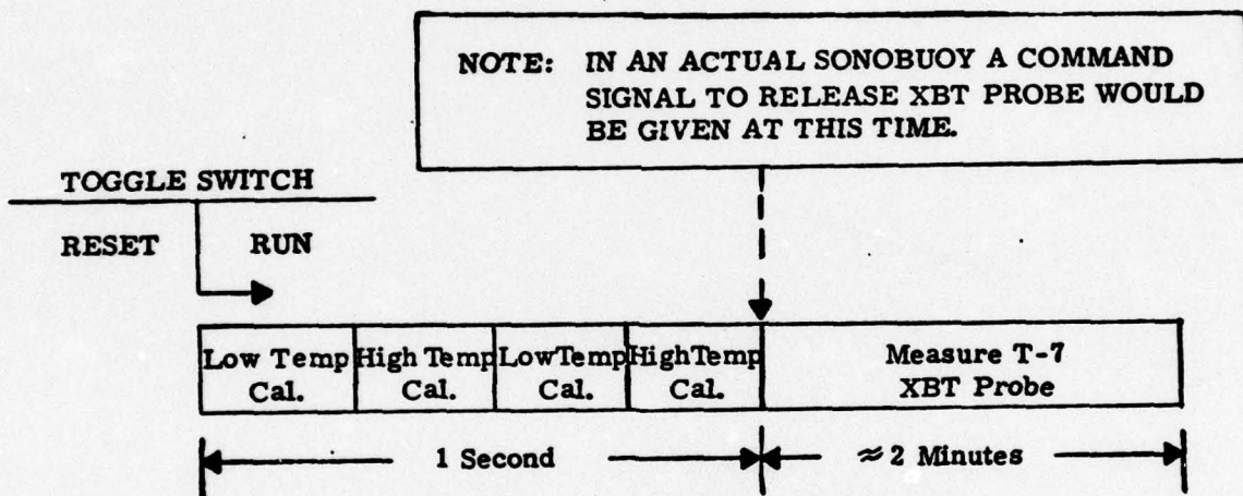
Figure 4-4 Calibration Sequence
