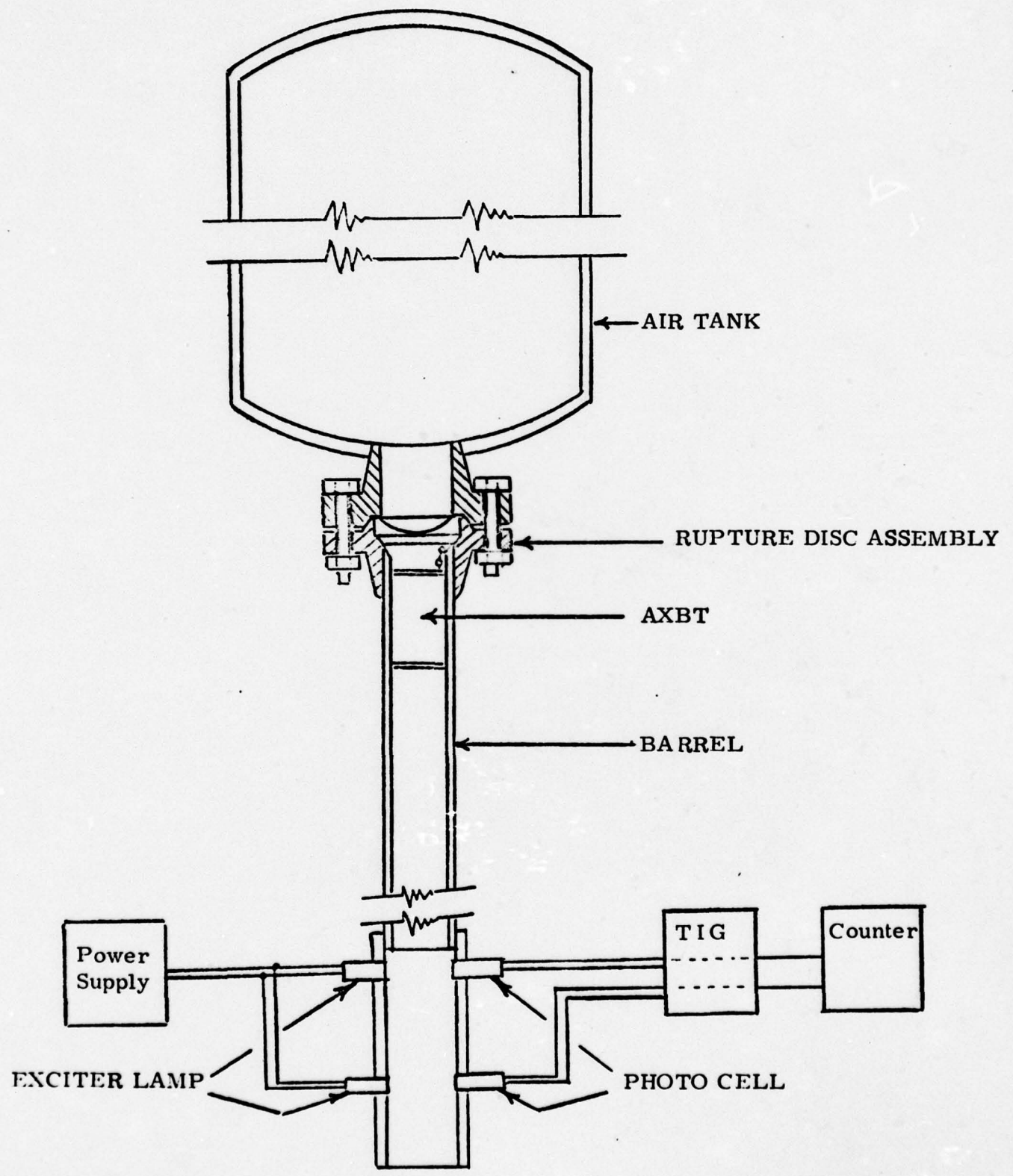
Figure 7-13 Air Gun
