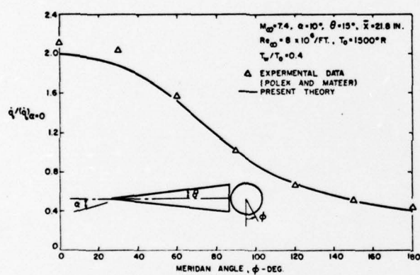
Fig. 6b Turbulent Heat Transfer Distribution on a Pointed Cone at Angle of Incidence
