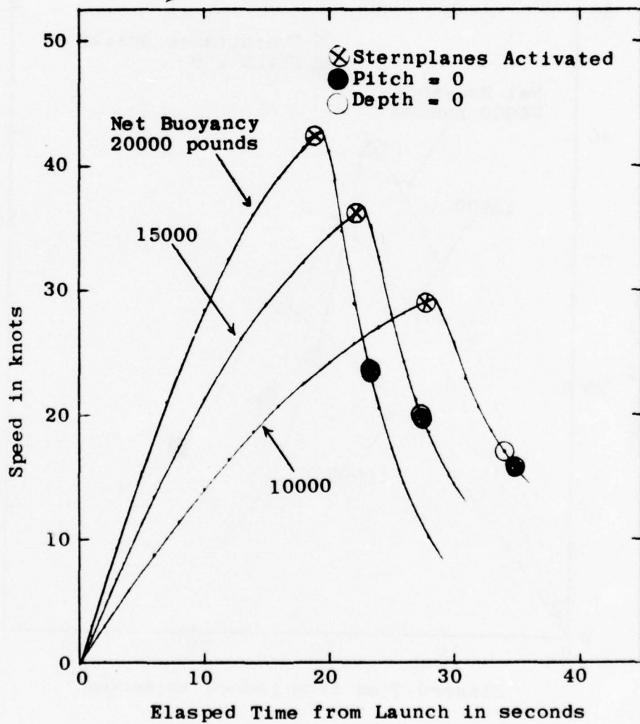
Figure 10 - Velocity Trajectories for Recovery Maneuver Initiated at 200 Feet
