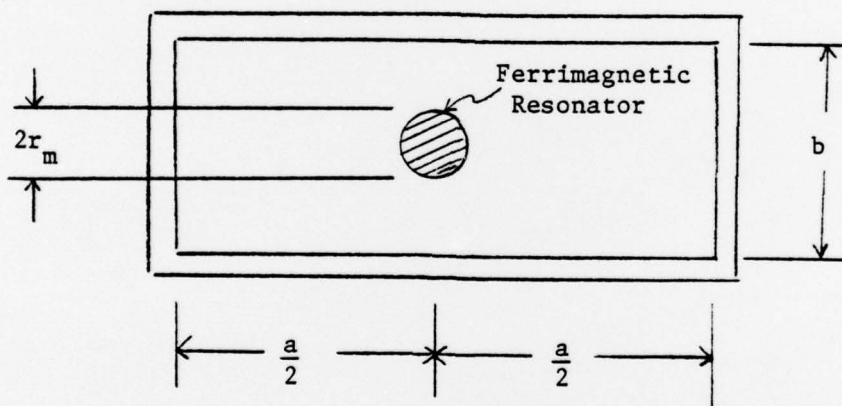
Figure 5. TE_{10} Waveguide
