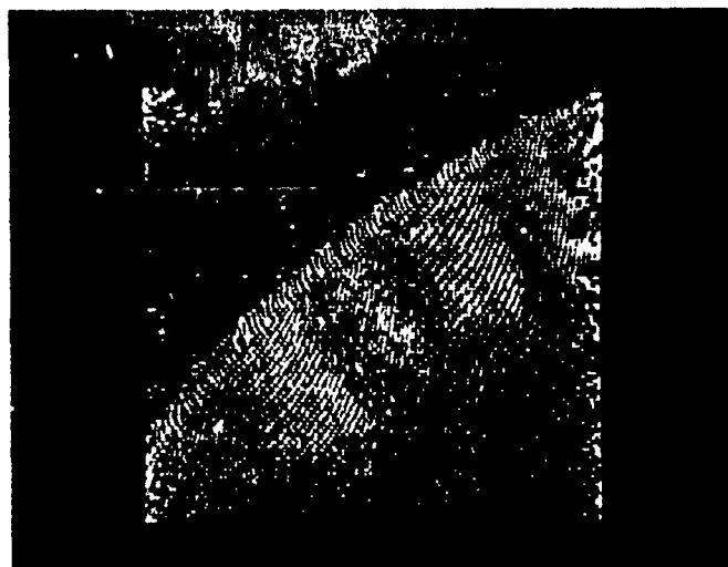
Figure 70: 11MHz Acoustical Hologram Of Two Side Drilled Holes In Resolution Standard S-1. This Hologram Contains The Phase And Amplitude Information From Which Reconstructed Images In Figures 71 - 73 Are Obtained.
