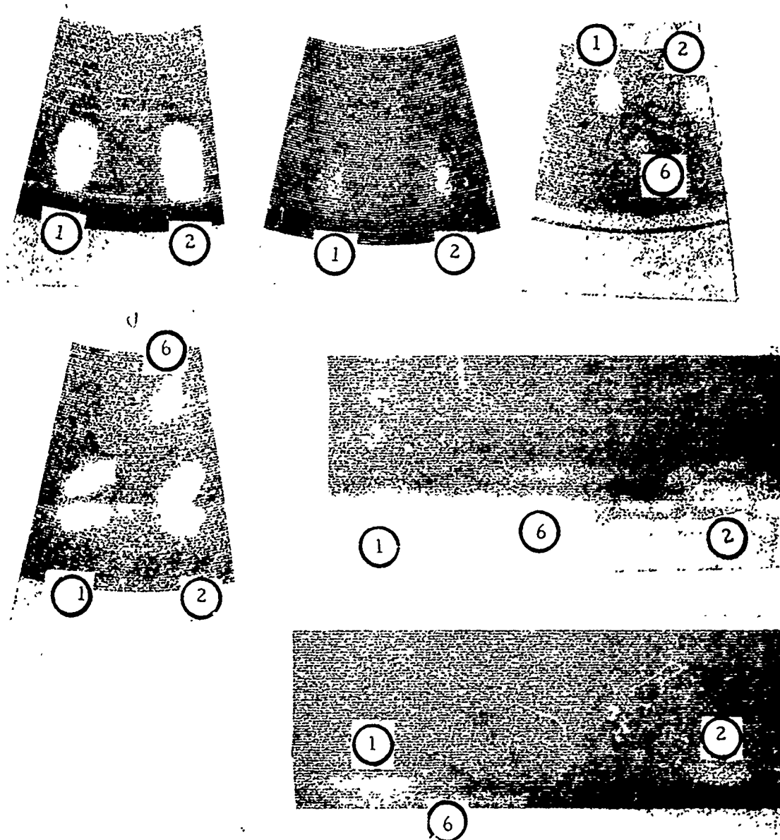
Figure 12. These 4 C-scans and 2 B-scans Illustrate a Wide Variation in Size and Shape of the Signals From Holes Numbers 1 and 2.
