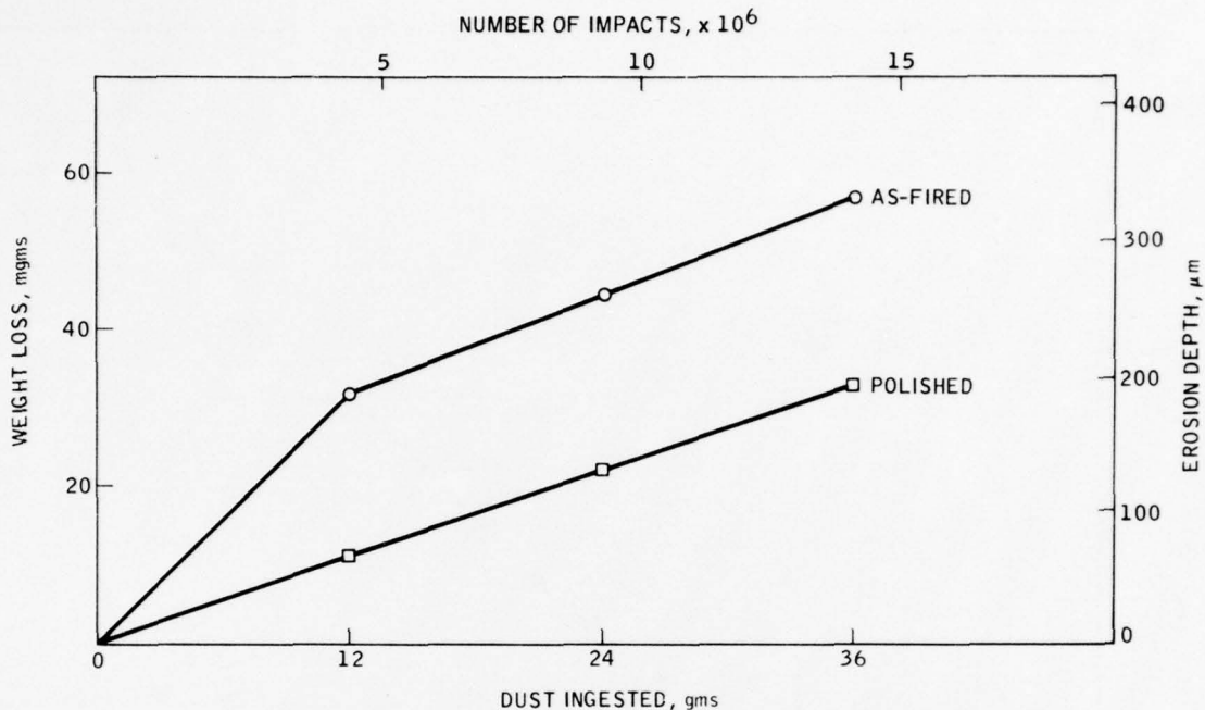
Figure 8. Effect of Surface Layer on Erosion of Reaction Bonded \text{Si}_3\text{N}_4 . As-fired Condition Contains Surface Oxide Layer. Polished Condition has Layer Removed. ( 273\mu Quartz, 155 mps).
