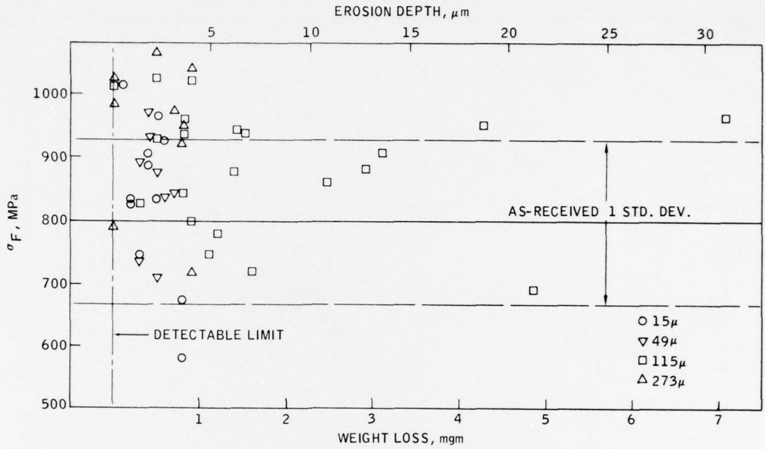
Figure 3. Effect of Erosion on Strength of Hot Pressed \text{Si}_3\text{N}_4 . Erosion conditions are the same as those of Figure 1.
