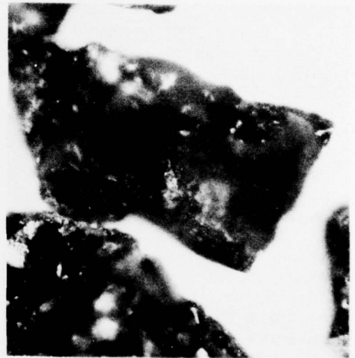
Typical Particle
