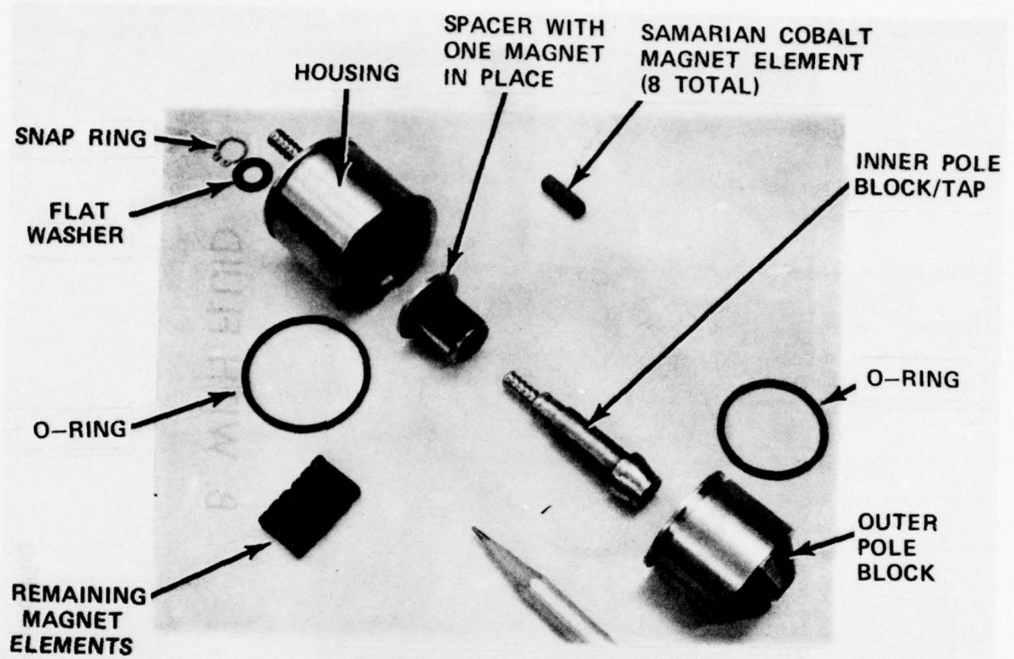
A. SEAL COMPONENTS
