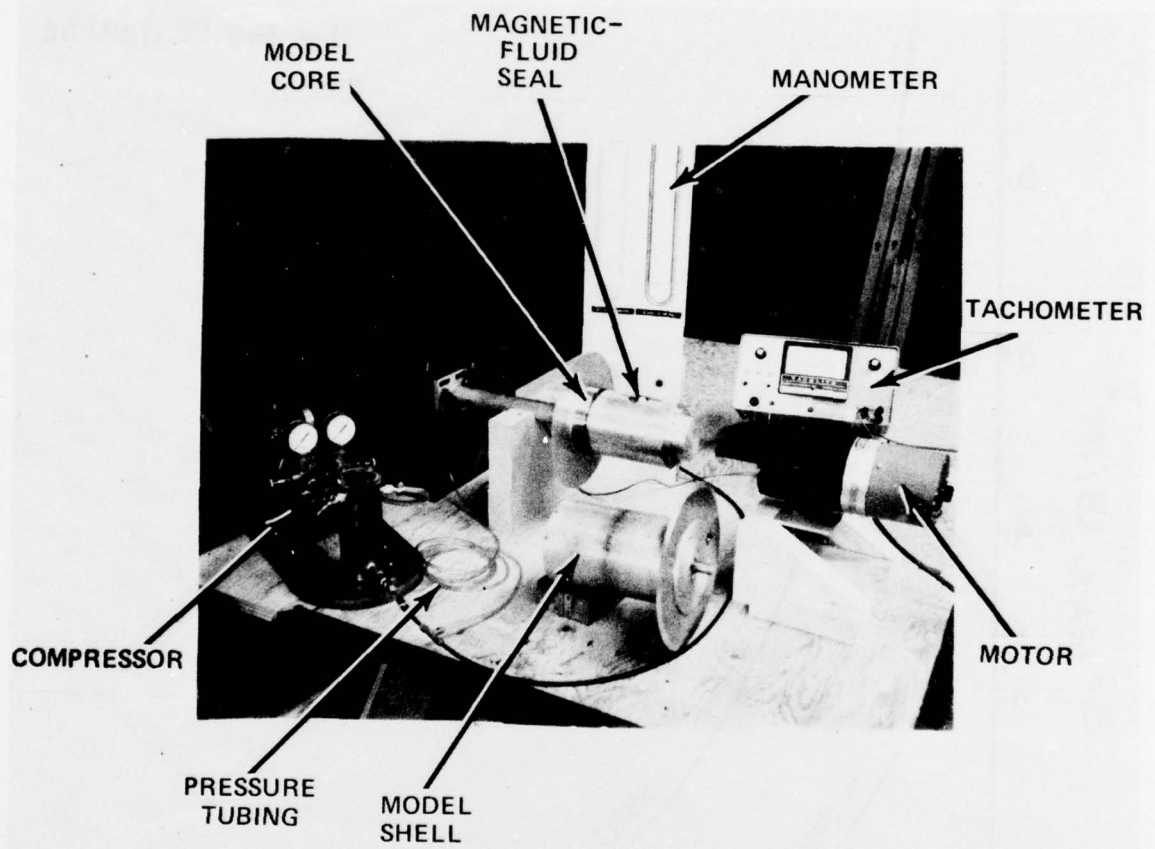
Figure A-9. Test Arrangement
