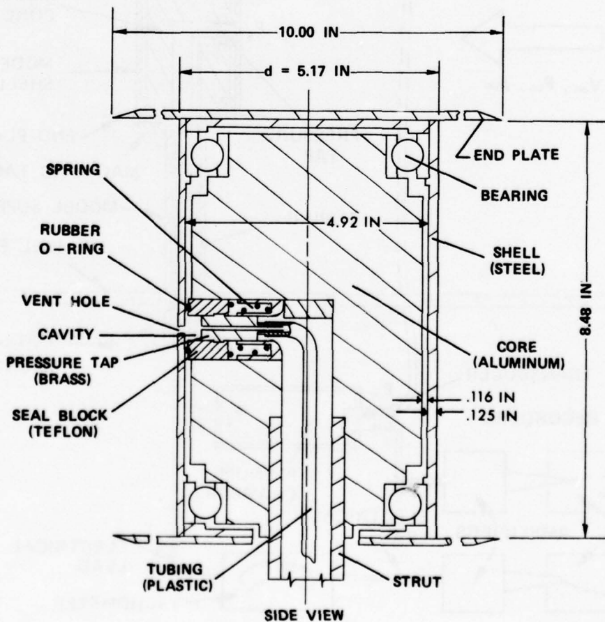
Figure A-1. Wind Tunnel Model
