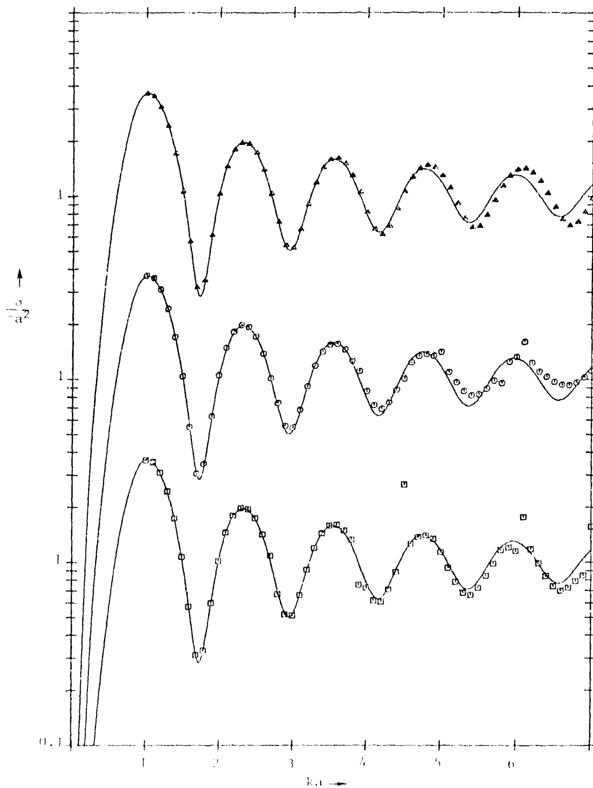
Fig. 6. Normalized radar cross section \sigma/a^2 versus ka for a conducting sphere of radius a . Solid line denotes exact solution, squares denote H-field solution, circles denote E-field solution, and triangles denote combined field solution.
