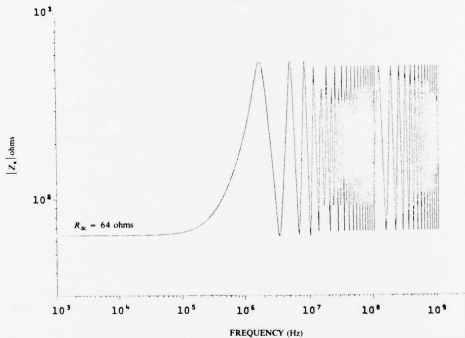
Figure 17. Transmission-line impedance computed by NLINE— l = 30 m, \psi = 90 deg, Q = 1.16 .
