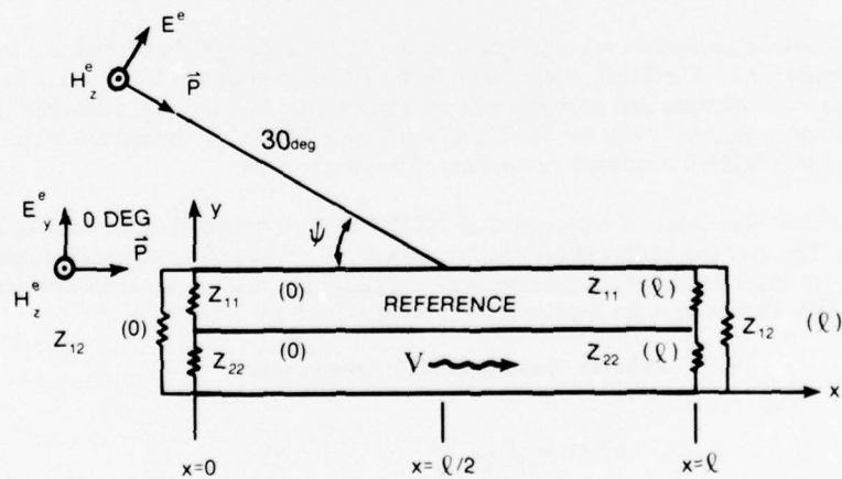
(b) Axial parameters. x, l . Propagation velocity, v . Angle of EMP incidence \psi . Incident electric and magnetic fields
